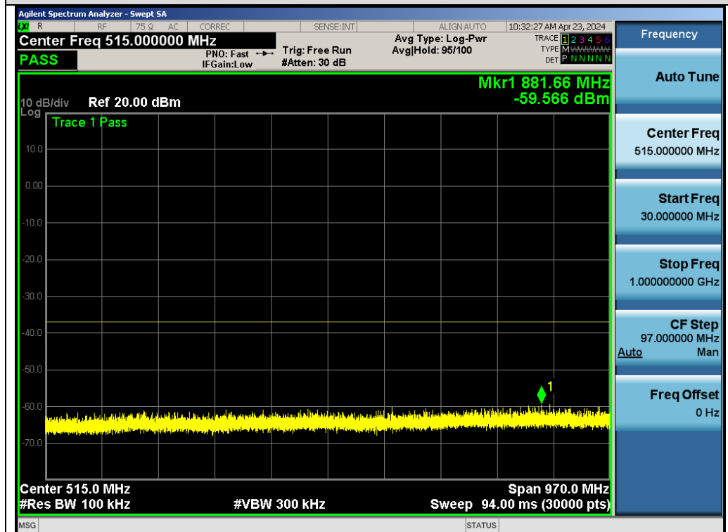
Test_Graph_802.11ac80_ANT1_5210_MCS0_Frequency Band 1
