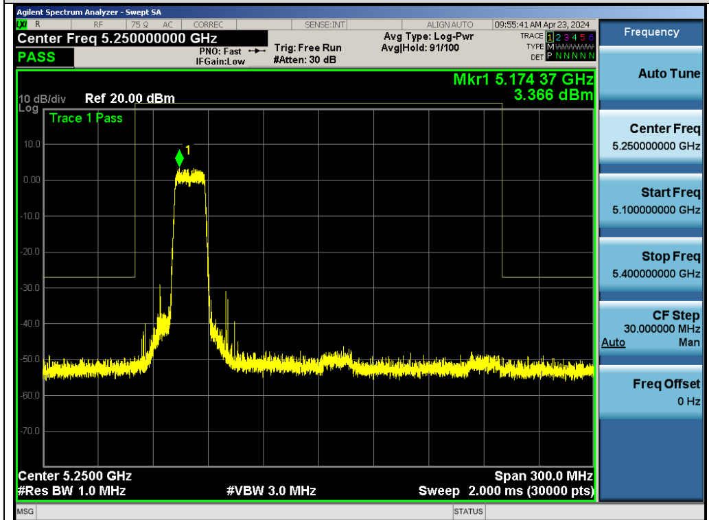
Test_Graph_802.11a_ANT1_5180_6Mbps_Frequency Band 3
