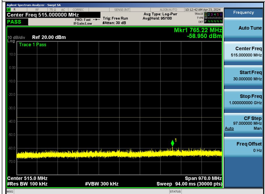
Test_Graph_802.11n40_ANT1_5190_MCS0_Frequency Band 1
