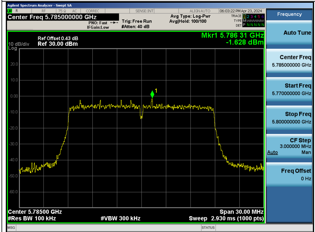
Test_Graph_802.11ac20_ANT2_5785_MCS0_PSD
