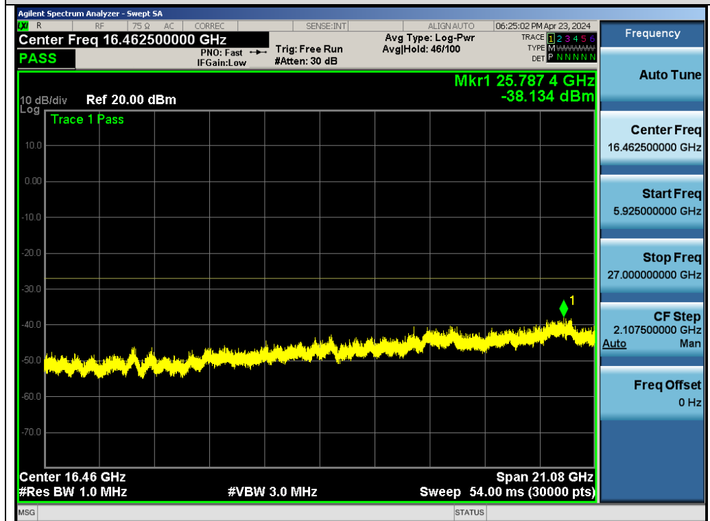
Test_Graph_802.11n40_ANT2_5795_MCS0_Frequency Band4
