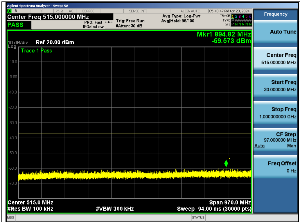
Test_Graph_802.11a_ANT2_5745_6Mbps_Frequency Band1
