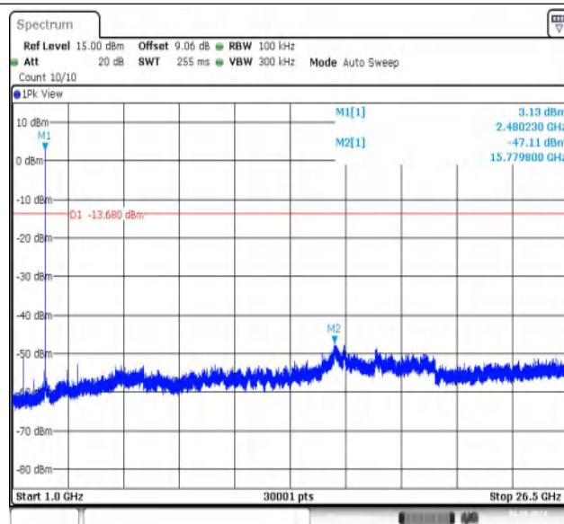
BLE_2M-Ant1-2480-1000~26500-PASS
