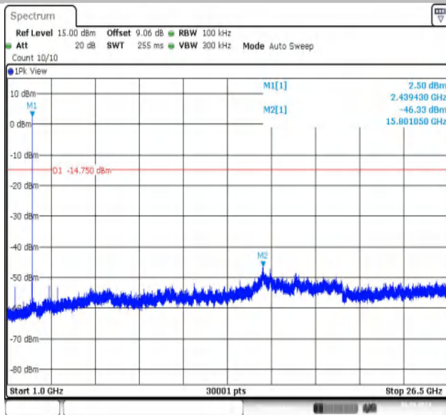
BLE_2M-Ant1-2440-0~Reference-PASS
