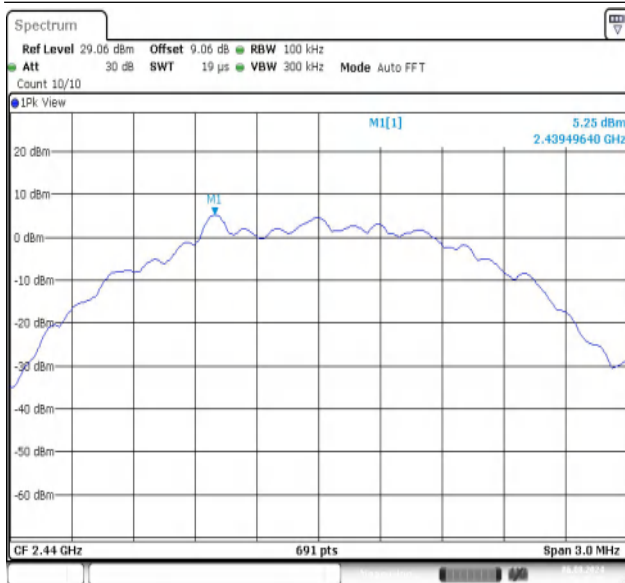
BLE_2M-Ant1-2440-0~Reference-PASS
