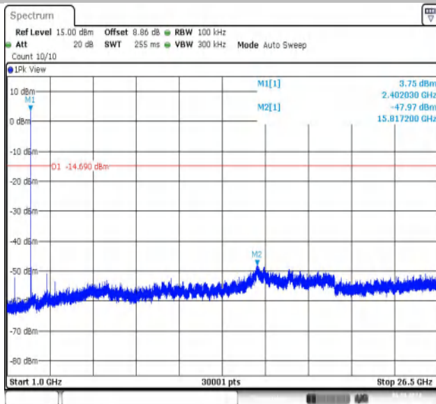
BLE_1M-Ant1-2402-0~Reference-PASS
