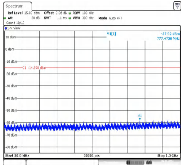
BLE_1M-Ant1-2402-30~1000-PASS
