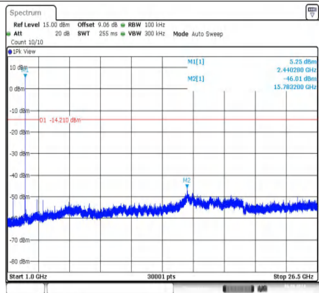
BLE_1M-Ant1-2440-1000~26500-PASS
