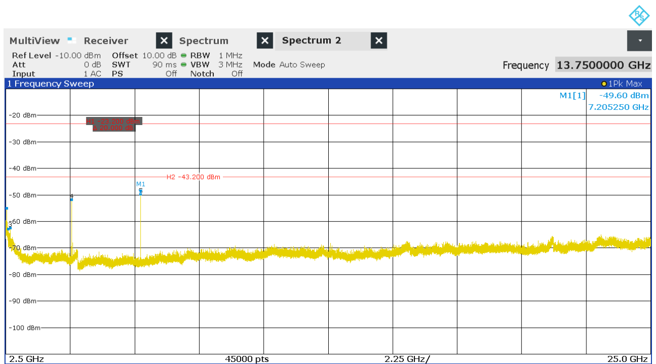
Figure 26: Chart of emissions test from 2.5 GHz to 25 GHz on lowest channel, Pk
