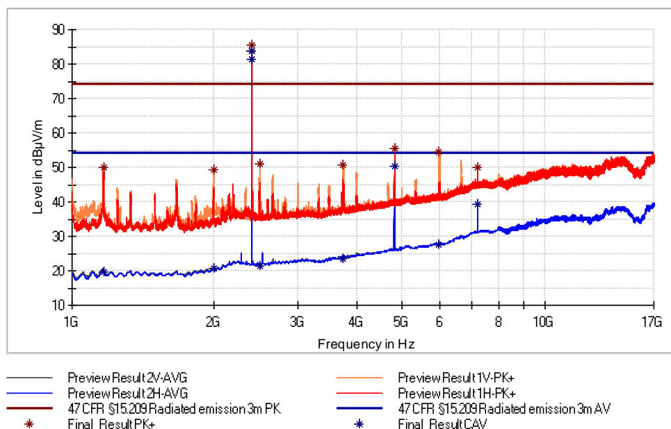
Figure 39: Chart of radiated emissions pre-measurement from 1 GHz to 17 GHz on lowest channel, EUT position Y, antenna polarization vertical and horizontal
