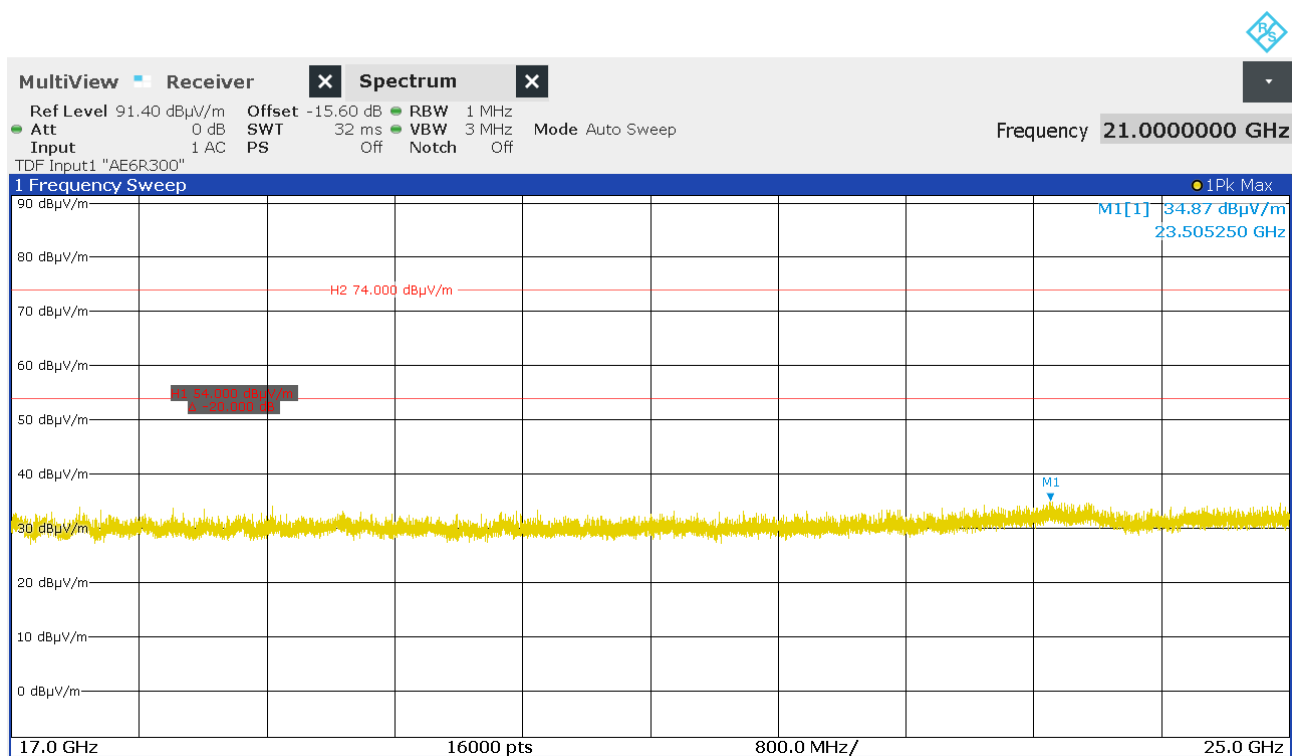
Figure 44: Chart of exploratory emissions measurement from 17 GHz to 25 GHz on highest channel, EUT position Y, antenna polarization vertical and horizontal
