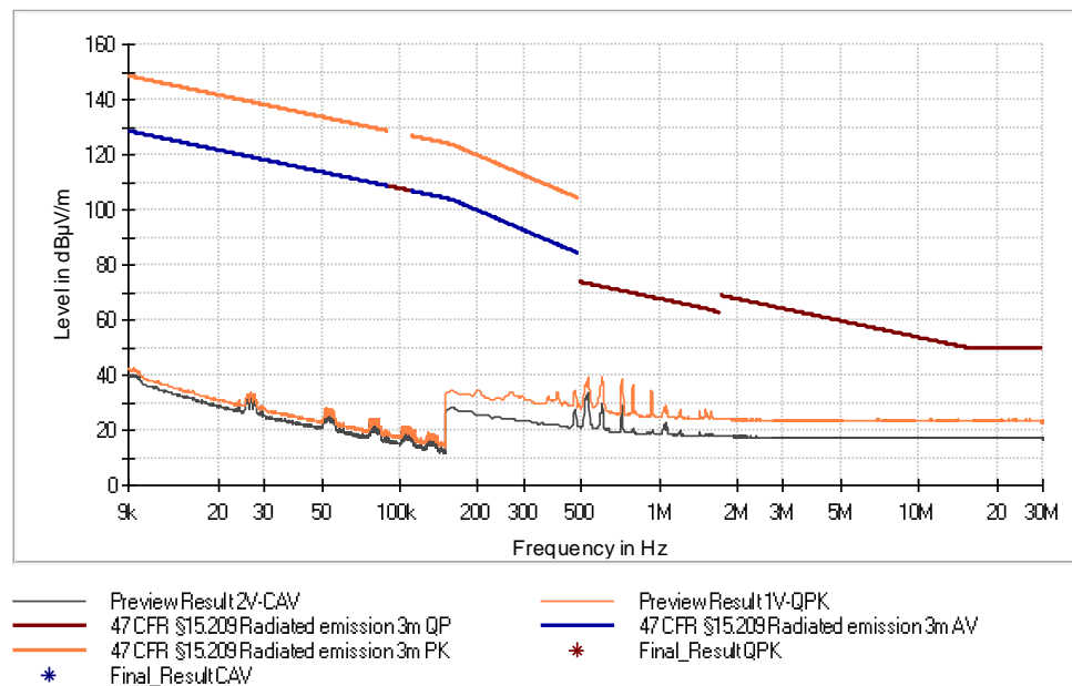
Figure 33: Chart of emissions test below 30 MHz on middle channel, EUT position Y, antenna in line
