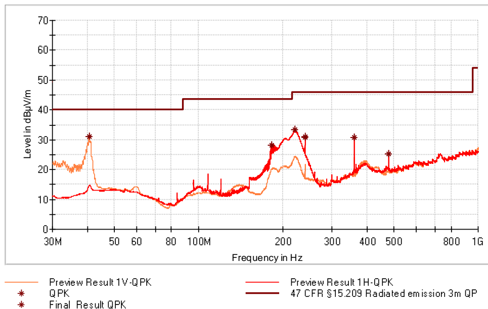
Figure 36: Chart of radiated emissions test from 30 MHz to 1 GHz on lowest channel, EUT position Y, antenna polarization vertical and horizontal
