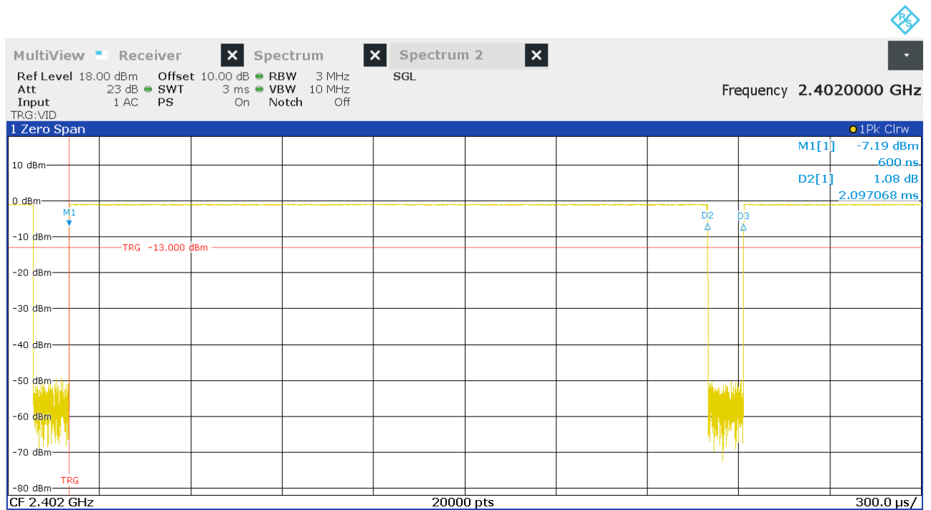
Figure 8: Chart of duty cycle test on lowest channel
