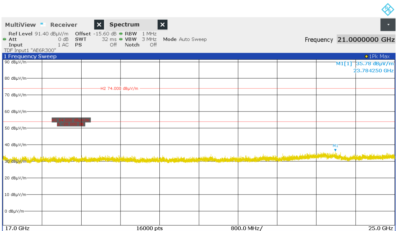
Figure 40: Chart of exploratory radiated emissions measurement from 17 GHz to 25 GHz on lowest channel, EUT position Y, antenna polarization vertical and horizontal
