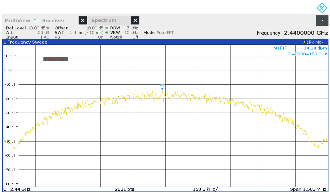
Figure 19: Chart of power spectral density on middle channel
