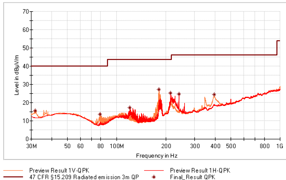
Figure 37: Chart of radiated emissions test from 30 MHz to 1 GHz on lowest channel, EUT position Y, antenna polarization vertical and horizontal
