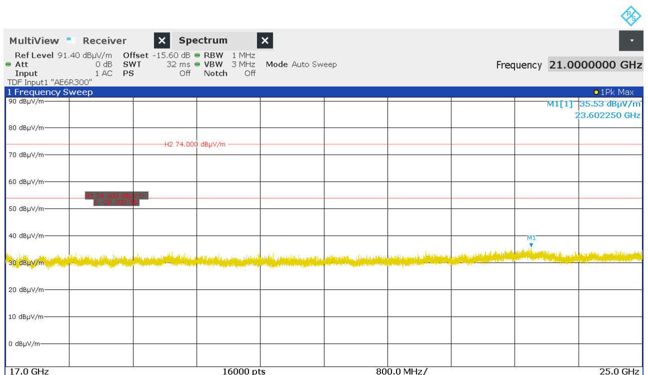
Figure 42: Chart of exploratory emissions measurement from 17 GHz to 25 GHz on middle channel, EUT position Y, antenna polarization vertical and horizontal
