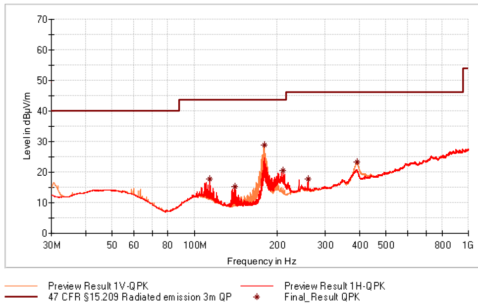
Figure 38: Chart of radiated emissions test from 30 MHz to 1 GHz on lowest channel, EUT position Y, antenna polarization vertical and horizontal
