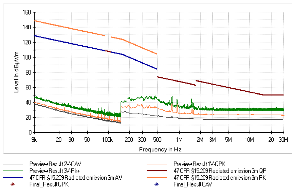
Figure 34: Chart of emissions test below 30 MHz on middle channel, EUT position Y, antenna parallel
