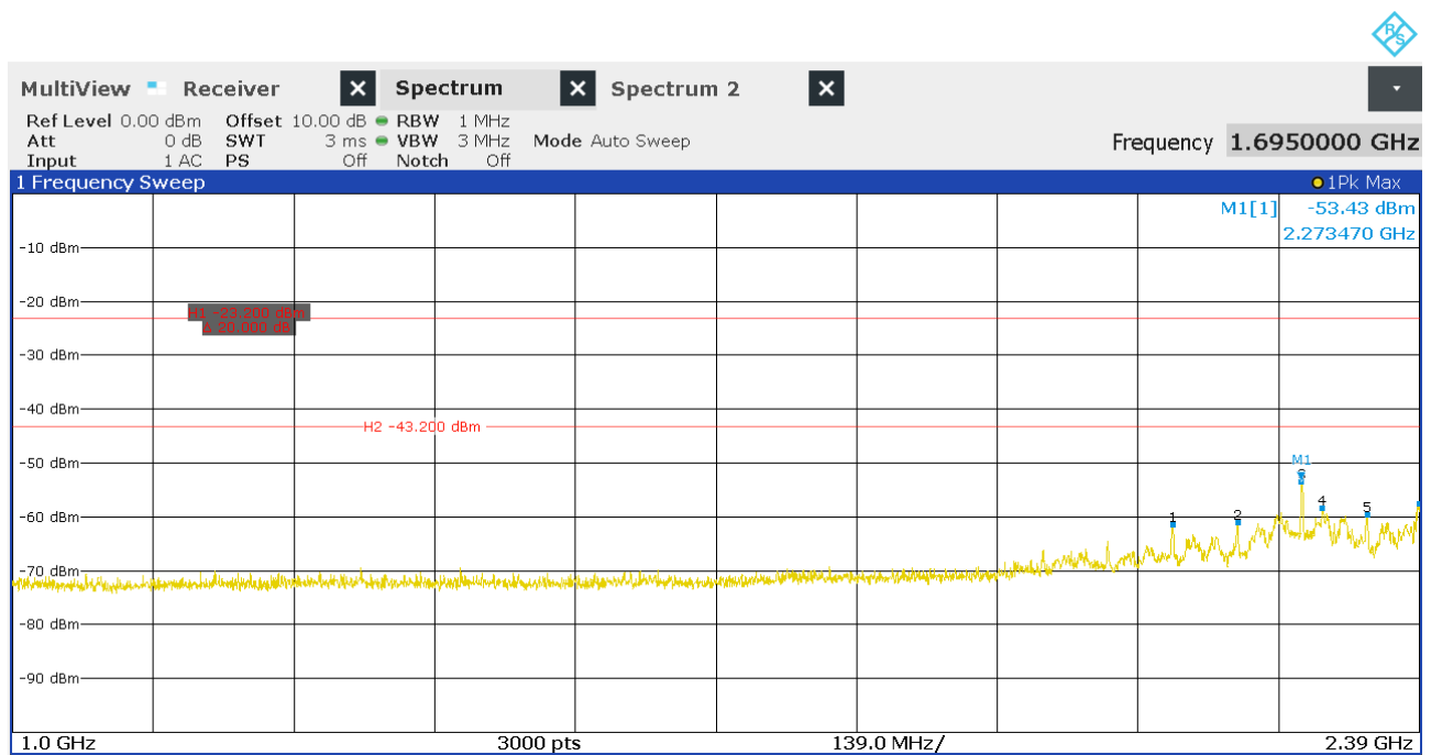
Figure 25: Chart of emissions test from 1 GHz to 2.39 GHz on lowest channel, Pk
