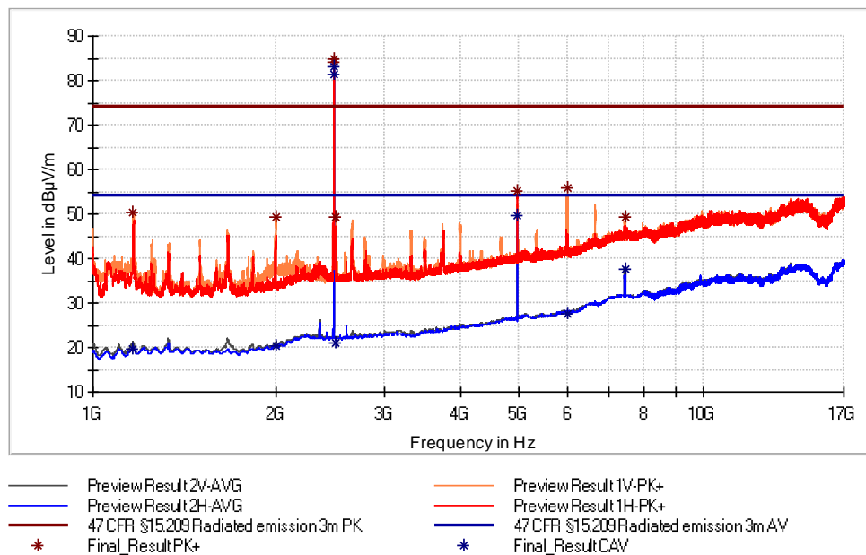
Figure 43: Chart of radiated emissions pre-measurement from 1 GHz to 17 GHz on highest channel, EUT position Y, antenna polarization vertical and horizontal
