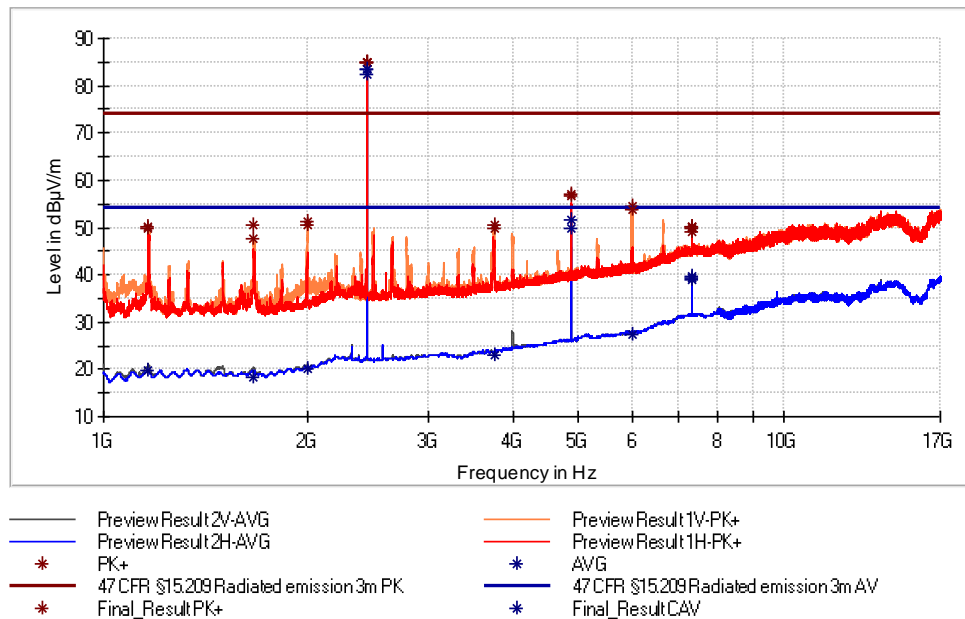
Figure 41: Chart of radiated emissions pre-measurement from 1 GHz to 17 GHz on middle channel, EUT position Y, antenna polarization vertical and horizontal
