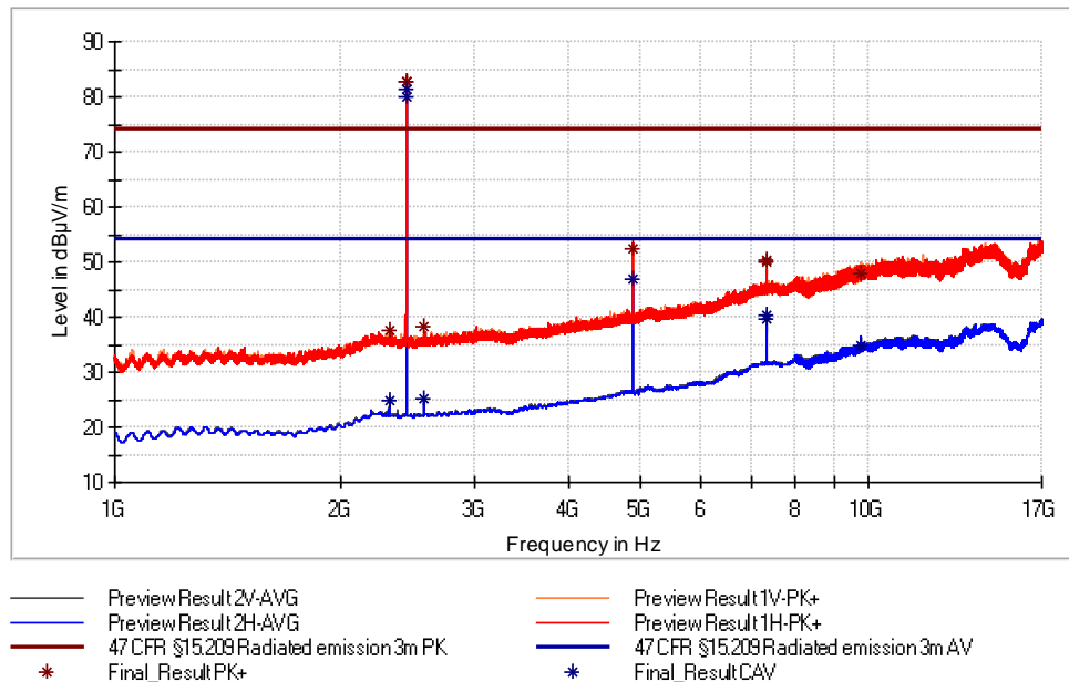
Figure 47: Chart of radiated emissions pre-measurement from 1 GHz to 17 GHz on middle channel, EUT position Y, antenna polarization vertical and horizontal
