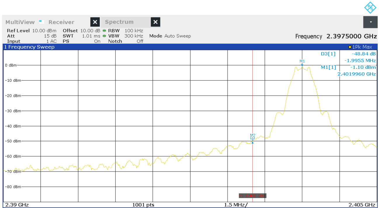
Figure 21: Chart of lower band-edge measurement on lowest channel
