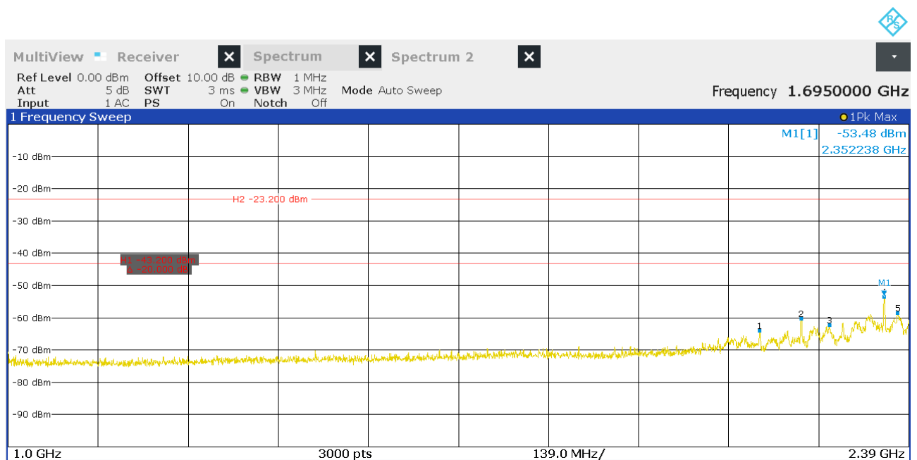
Figure 31: Chart of emissions test from 1 GHz to 2.39 GHz on highest channel, Pk
