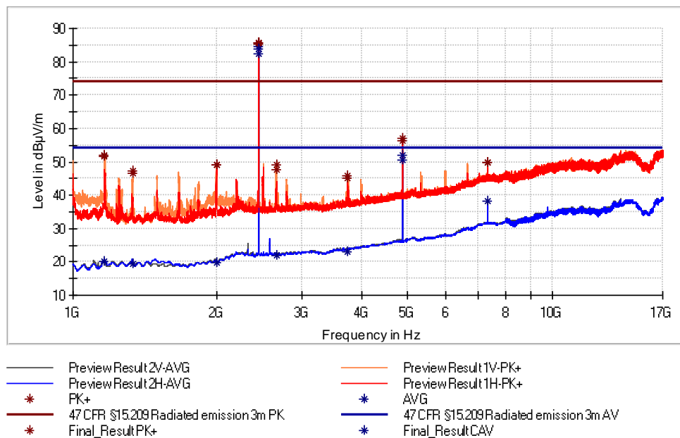
Figure 45: Chart of radiated emissions pre-measurement from 1 GHz to 17 GHz on middle channel, EUT position Y, antenna polarization vertical and horizontal
