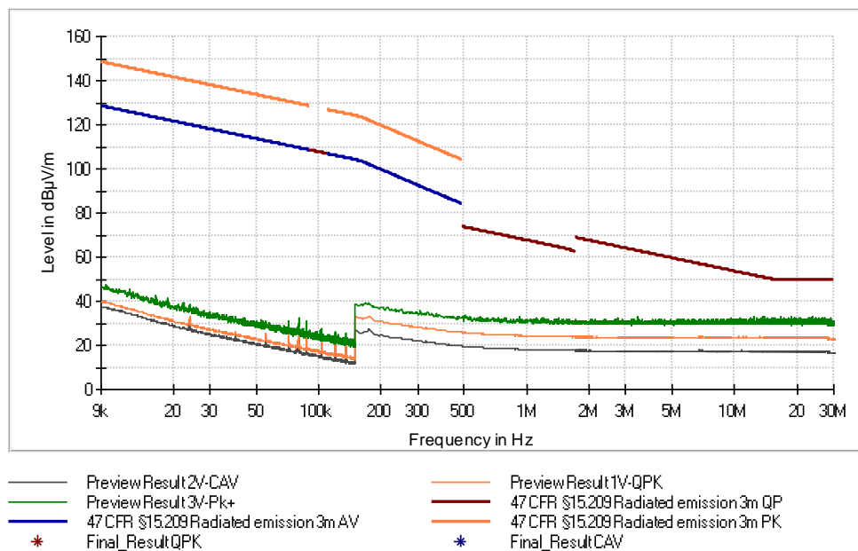
Figure 35: Chart of emissions test below 30 MHz on middle channel, EUT position Y, antenna parallel
