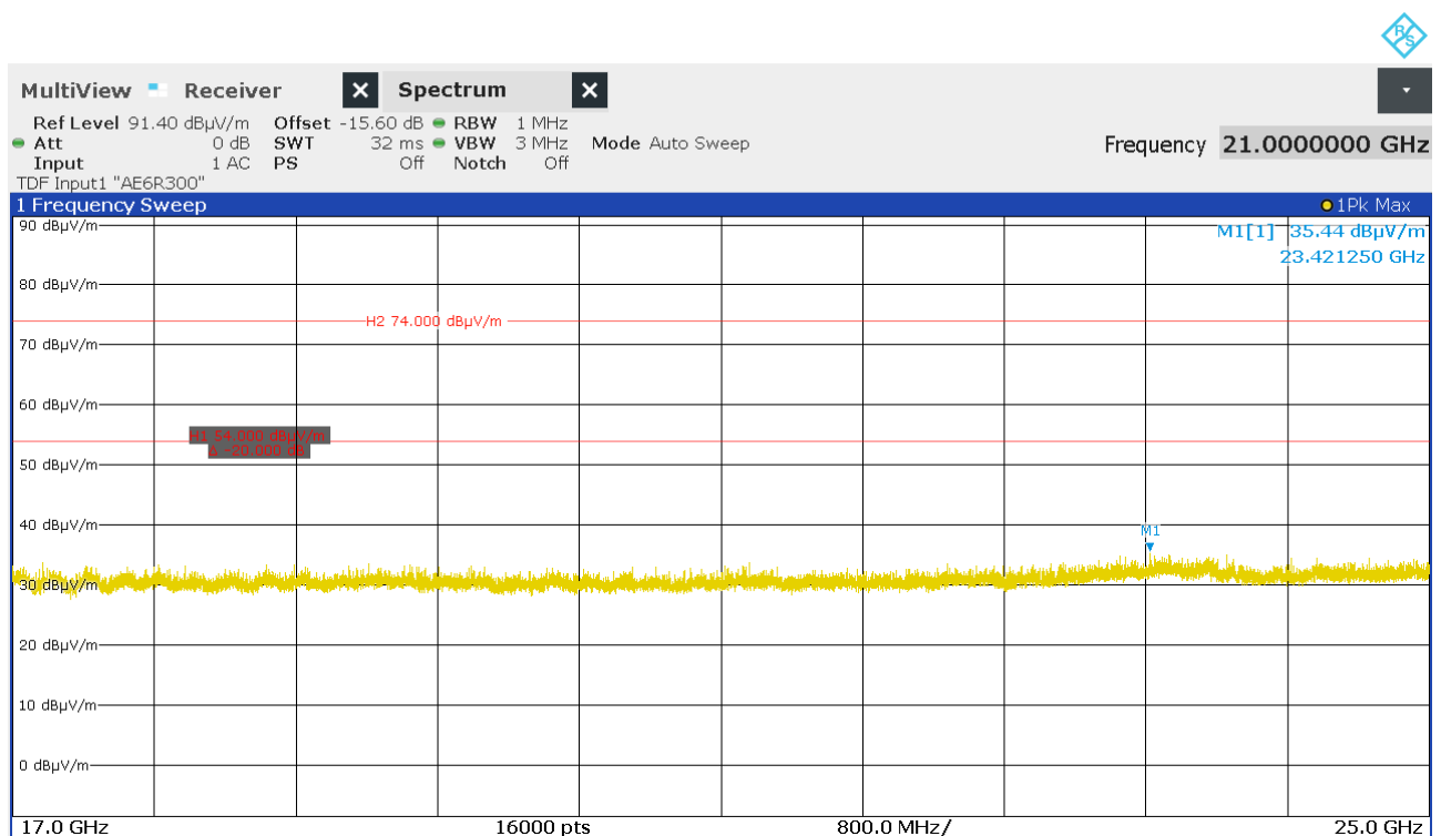
Figure 48: Chart of exploratory emissions measurement from 17 GHz to 25 GHz on middle channel, EUT position Y, antenna polarization vertical and horizontal
