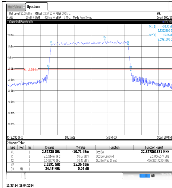
NTNV-N7-PC3-15-25-M-DFT-QPSK-Outter_Full-Ant1-PASS
