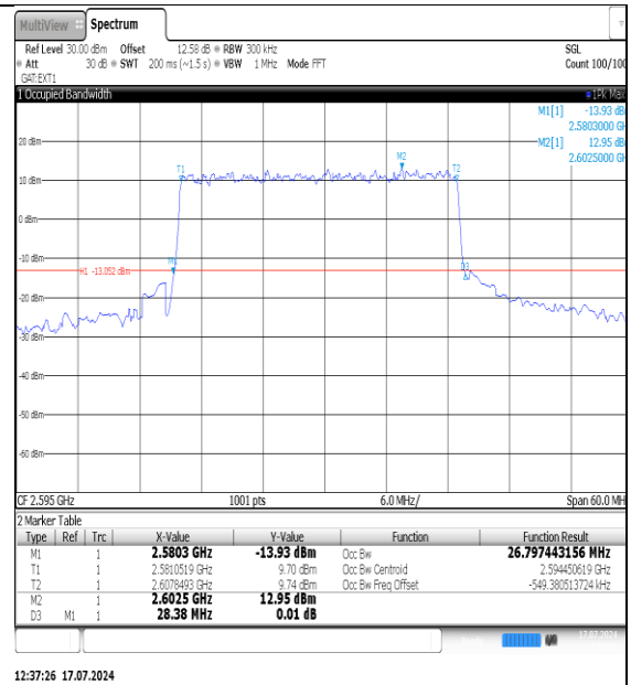
NTNV-N38-PC3-30-30-M-DFT-16QAM-Outer_Full- Ant1-PASS
