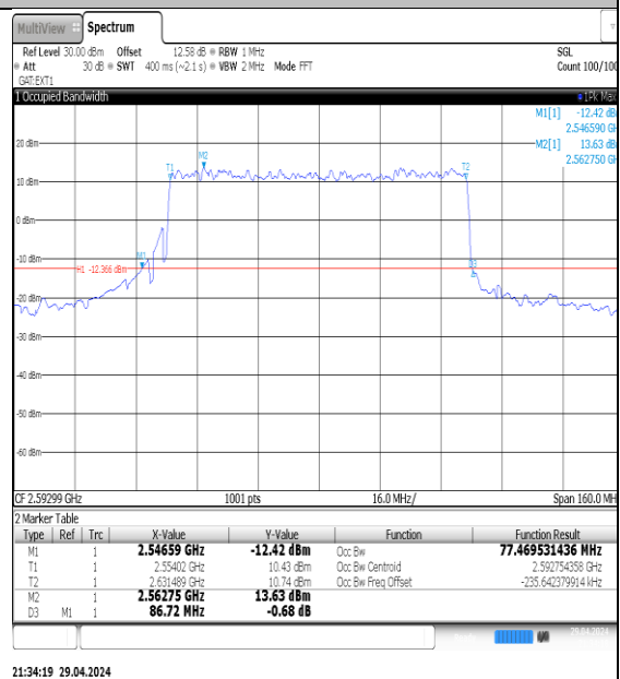
NTNV-N41-PC3-30-80-M-DFT-16QAM-Outer_Full-Ant1-PASS
