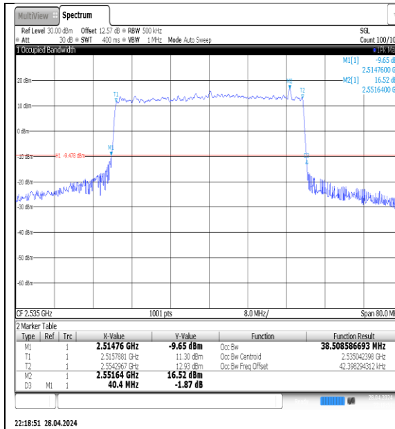
NTNV-N7-PC3-15-40-M-DFT-QPSK-Outter_Full-Ant1-PASS
