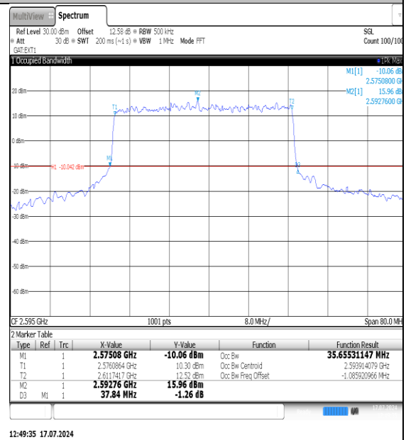
NTNV-N38-PC3-30-40-M-DFT-QPSK-Outer_Full- Ant1-PASS
