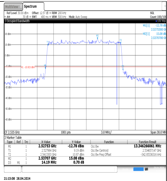
NTNV-N7-PC3-15-15-M-DFT-16QAM-Outet_Full-Ant1-PASS
