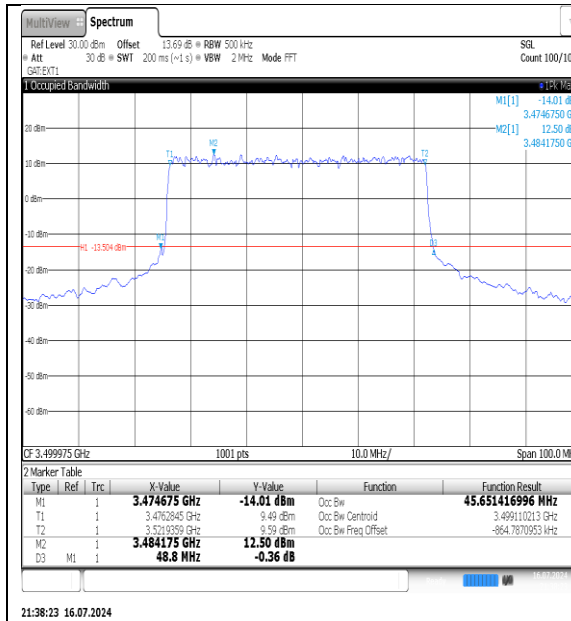
NTNV-N77-3450-3550-PC3-30-50-M-DFT- PI2BPSK-Outer_Full-Ant1-PASS
