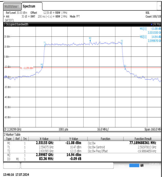
NTNV-N41-PC3-30-80-M-DFT-PI2BPSK-Outer_Full-Ant1-PASS
