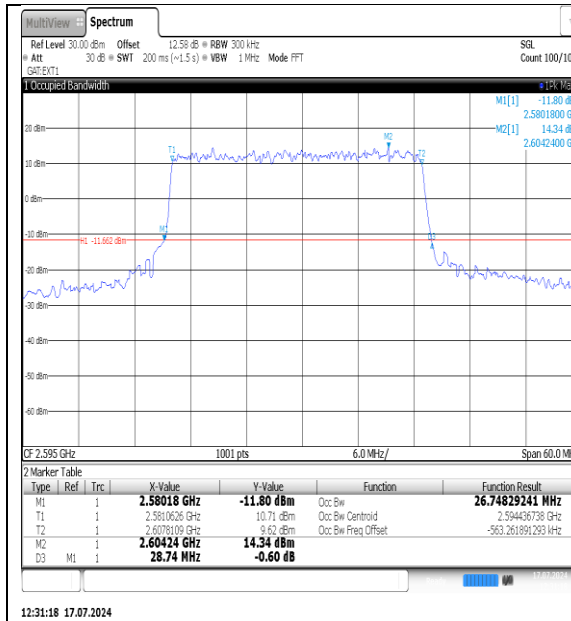
NTNV-N38-PC3-30-30-M-DFT-QPSK-Outer_Full- Ant1-PASS
