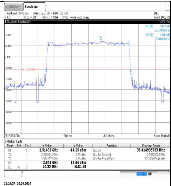
NTNV-N7-PC3-15-40-M-DFT-16QAM-Outter_Full-Ant1-PASS
