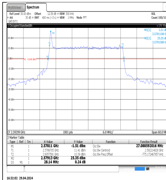
NTNV-N41-PC3-30-30-M-DFT-16QAM-Outer_Full-Ant1-PASS
