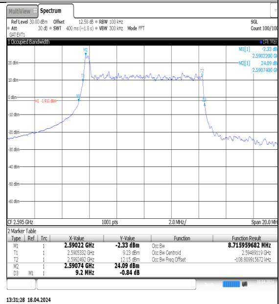
NTNV-N38-PC3-30-10-M-DFT-QPSK-Outter_Full-Ant1-PASS
