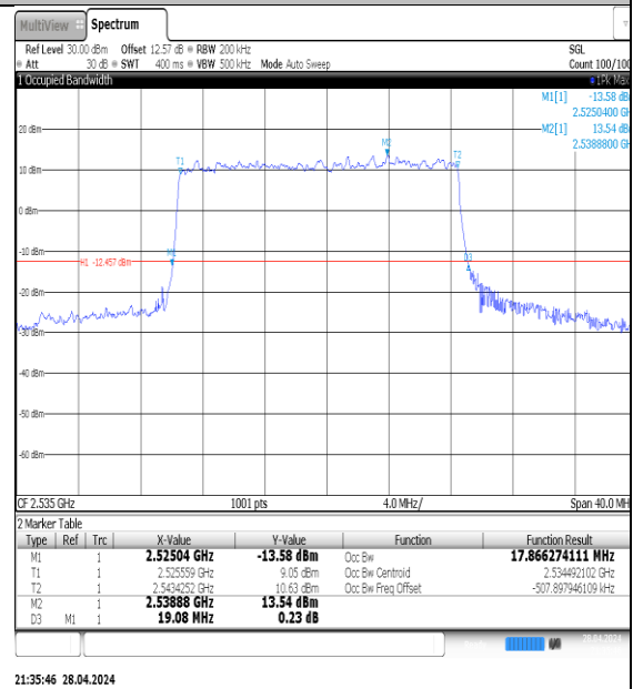
NTNV-N7-PC3-15-20-M-DFT-16QAM-Outet_Full-Ant1-PASS
