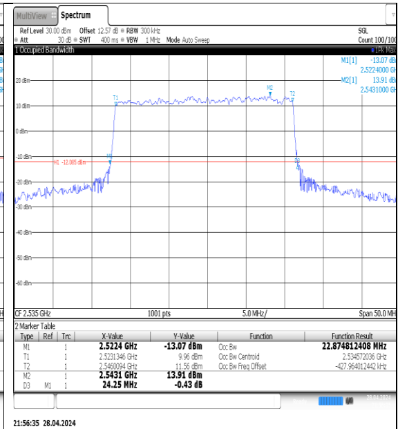
NTNV-N7-PC3-15-25-M-DFT-16QAM-Outter_Full-Ant1-PASS
