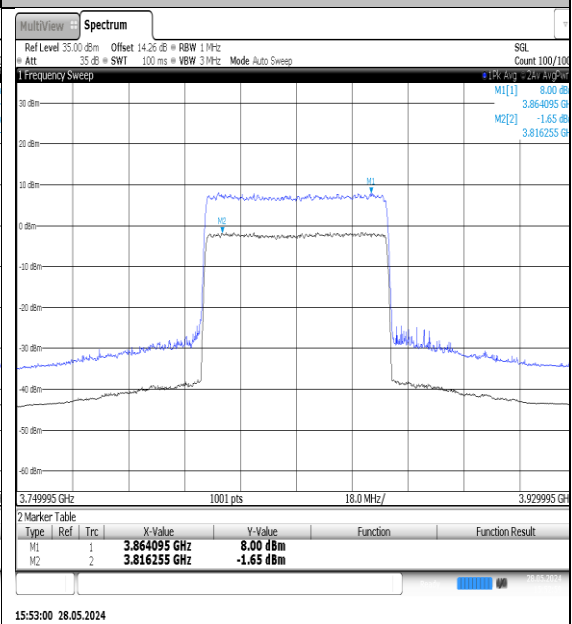
NTNV-N77-3700-3980-PC3-30-60-M-DFT-QPSK- Outer_Full-Ant1-PASS
