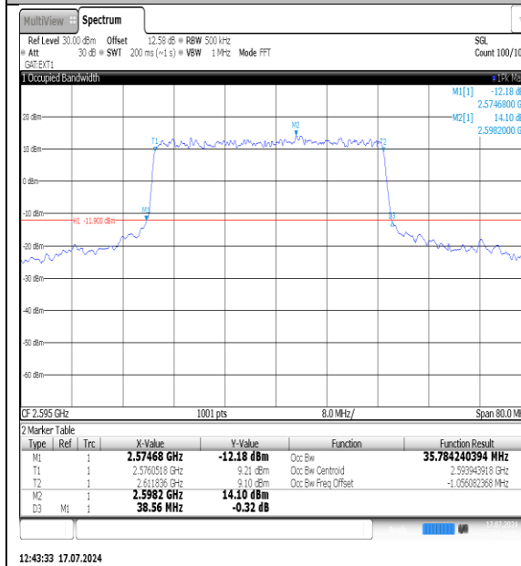
NTNV-N38-PC3-30-40-M-DFT-PI2BPSK- Outer_Full-Ant1-PASS
