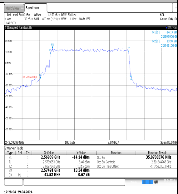
NTNV-N41-PC3-30-40-M-DFT-16QAM-Outer_Full-Ant1-PASS
