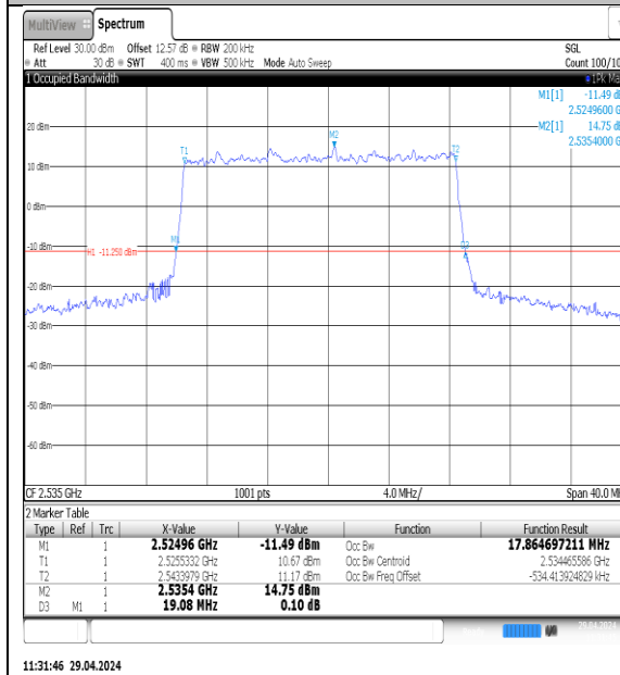
NTNV-N7-PC3-15-20-M-DFT-QPSK-Outet_Full-Ant1-PASS
