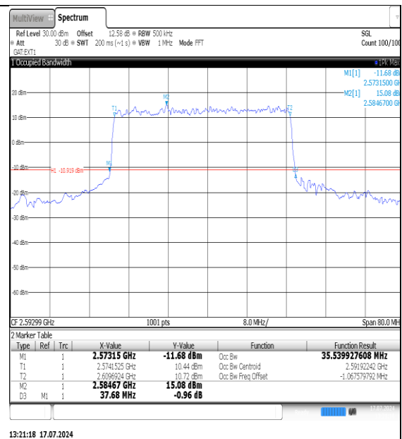
NTNV-N41-PC3-30-40-M-DFT-PI2BPSK-Outer_Full-Ant1-PASS
