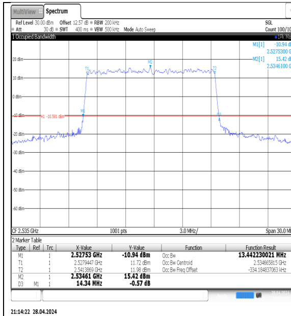
NTNV-N7-PC3-15-15-M-DFT-QPSK-Outet_Full-Ant1-PASS
