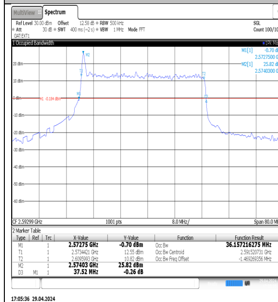
NTNV-N41-PC3-30-40-M-DFT-QPSK-Outer_Full-Ant1-PASS
