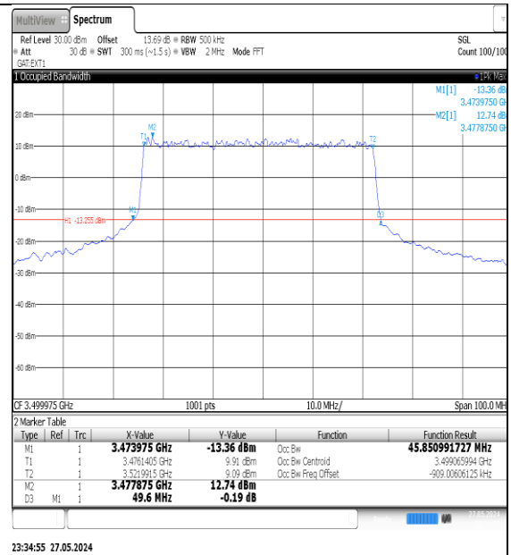
NTNV-N77-3450-3550-PC3-30-50-M-DFT-QPSK- Outer_Full-Ant1-PASS
