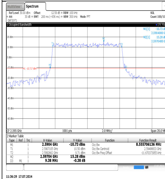
NTNV-N38-PC3-30-10-M-DFT-PI2BPSK-Outter_Full-Ant1-PASS
