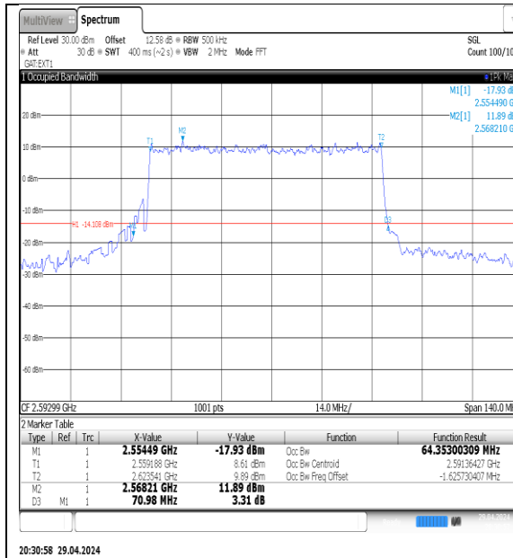
NTNV-N41-PC3-30-70-M-DFT-16QAM-Outer_Full-Ant1-PASS
