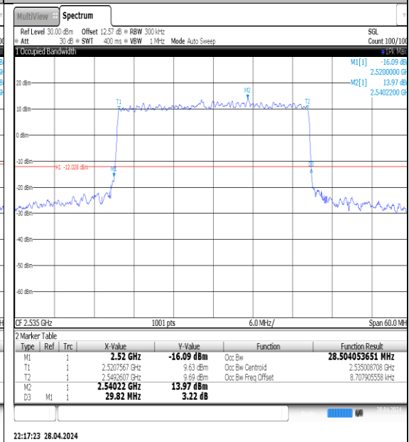
NTNV-N7-PC3-15-30-M-DFT-16QAM-Outter_Full-Ant1-PASS
