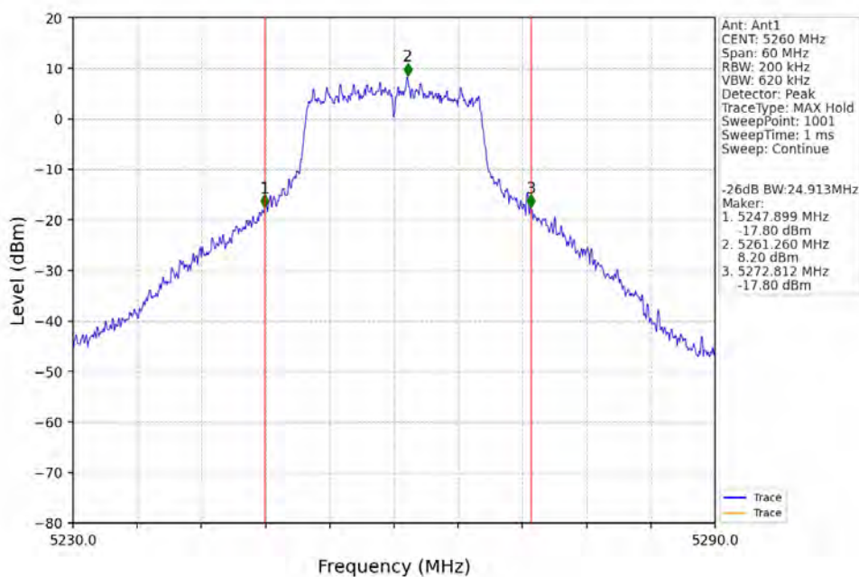
802.11a_LCH_5260MHz_Ant1_NTNV
