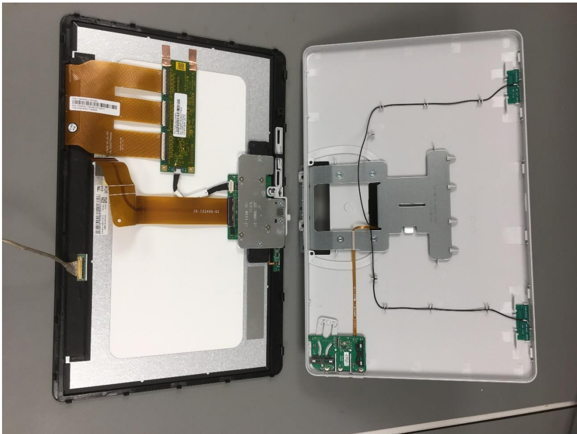
Inside screen (PCB antennas to the left):
