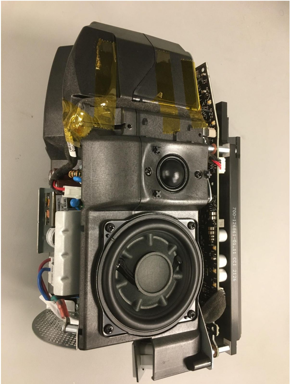
Front speaker, mainboard and PSU:
