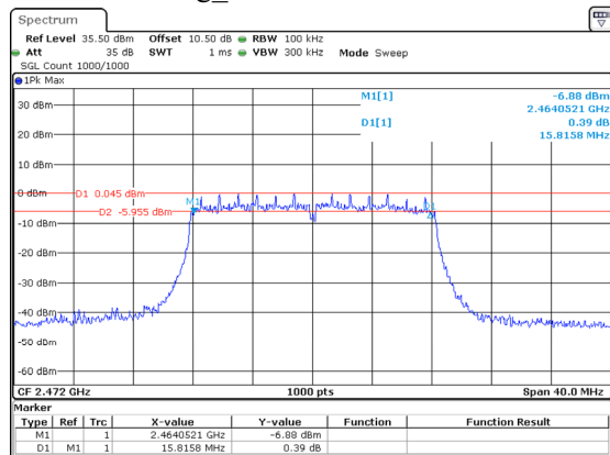
802.11g_2472MHz 15.816MHz
