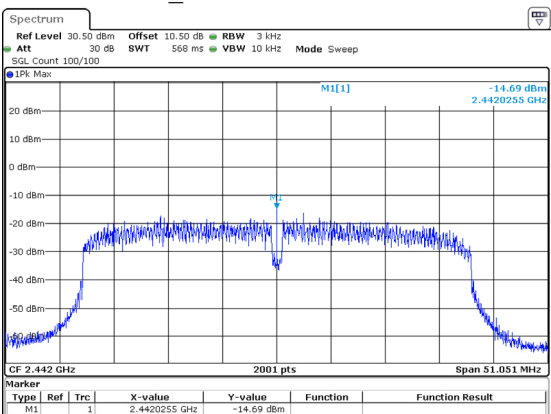
802.11n40_2442MHz -14.69dBm/3kHz
