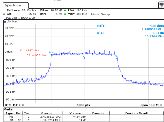
802.11g_2412MHz 16.376MHz
