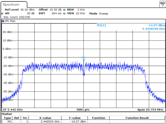
802.11n20_2442MHz -14.27dBm/3kHz
