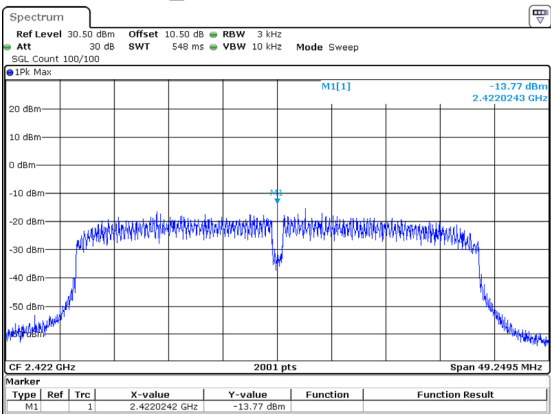
802.11n40_2422MHz -13.77dBm/3kHz
