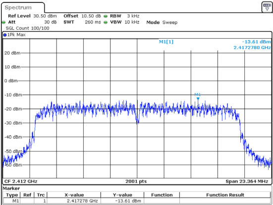
802.11n20_2412MHz -13.61dBm/3kHz
