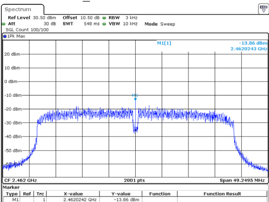
802.11n40_2462MHz -13.86dBm/3kHz
