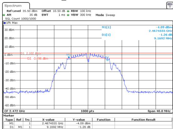
802.11b_2472MHz 9.169MHz
