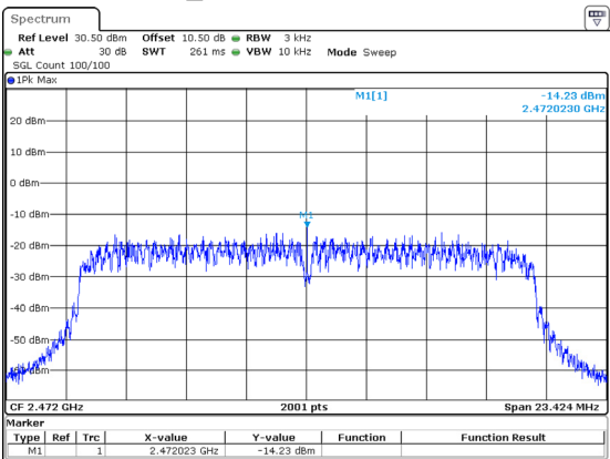
802.11n20_2472MHz -14.23dBm/3kHz
