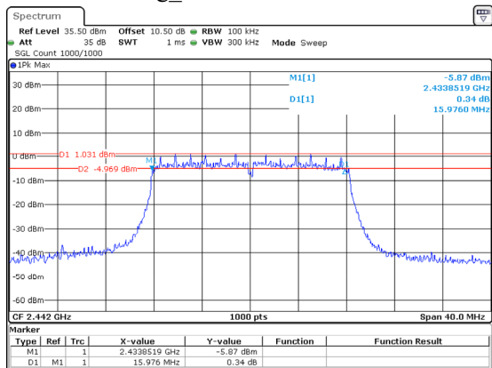
802.11g_2442MHz 15.976MHz
