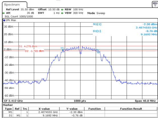
802.11b_2412MHz 9.169MHz
