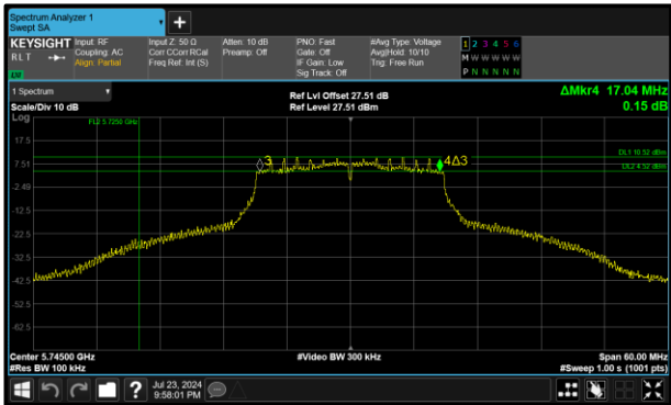
Figure 281 - 802.11n HT20 Maximum 6 dB EBW
