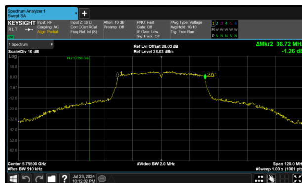
Figure 295 - 802.11n HT40 Maximum 99% OBW
