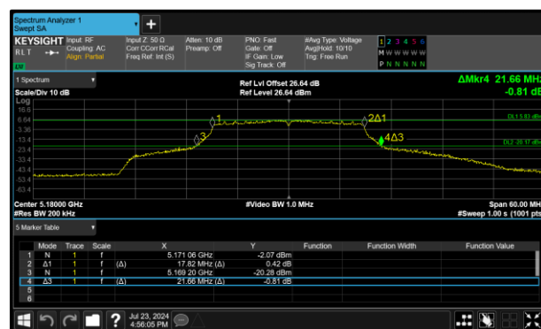
Figure 293 - 802.11n HT20 Maximum 99% OBW
