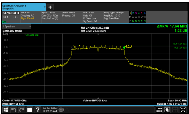
Figure 309 - 802.11n HT20 Maximum 6 dB EBW
