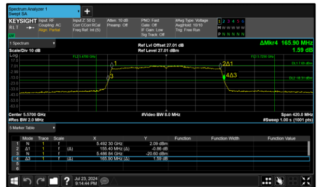
Figure 279 - 802.11ax HE160 SU Maximum 99% OBW
