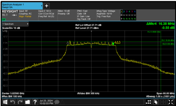
Figure 280 - 802.11n HT20 Minimum 6 dB EBW
