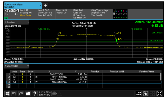
Figure 271 - 802.11ac VHT160 Maximum 99% OBW
