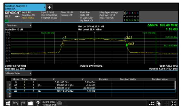
Figure 307 - 802.11ax HE160 SU Maximum 99% OBW
