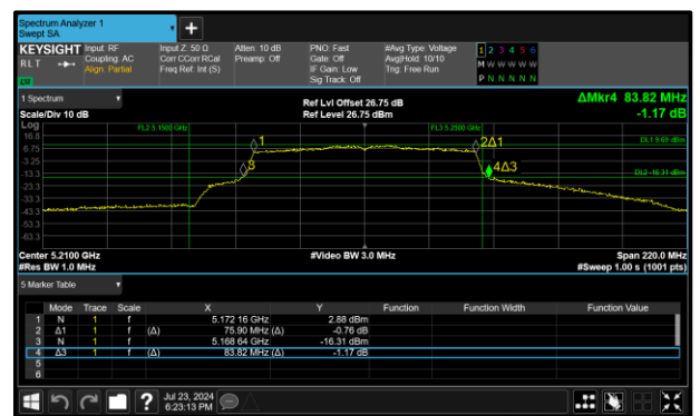
Figure 269 - 802.11ac VHT80 Maximum 99% OBW
