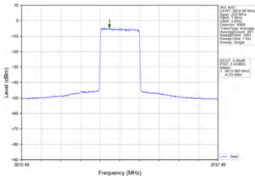
n78d 30kHz MIMO NTNV 90MHz CP-OFDM 256 QAM 3624.99MHz Inner Full
