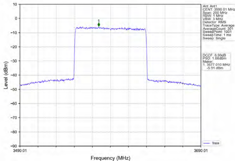
n78d_30kHz_MIMO_NTNV_80MHz_CP-OFDM_16_QAM_3590.01MHz_Inner_Full
