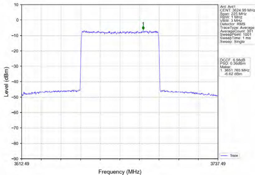
n78d 30kHz MIMO NTNV 90MHz CP-OFDM 256 QAM 3624.99MHz Inner Full
