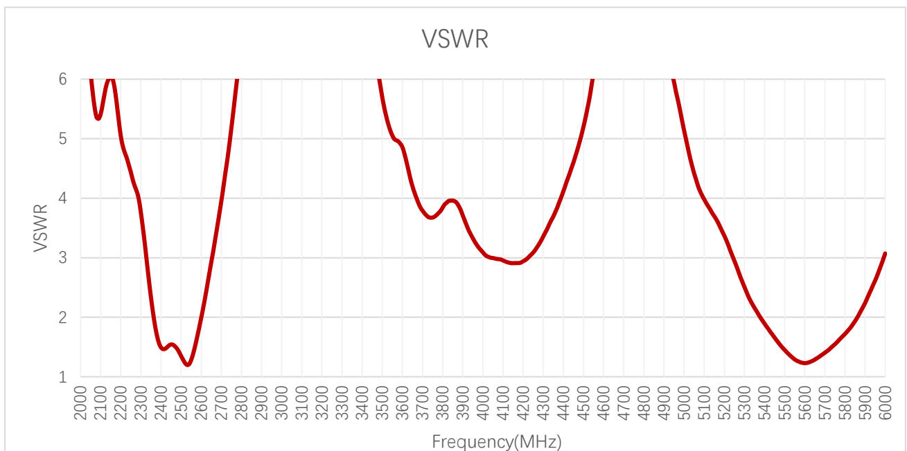
VSWR – Wi-Fi
