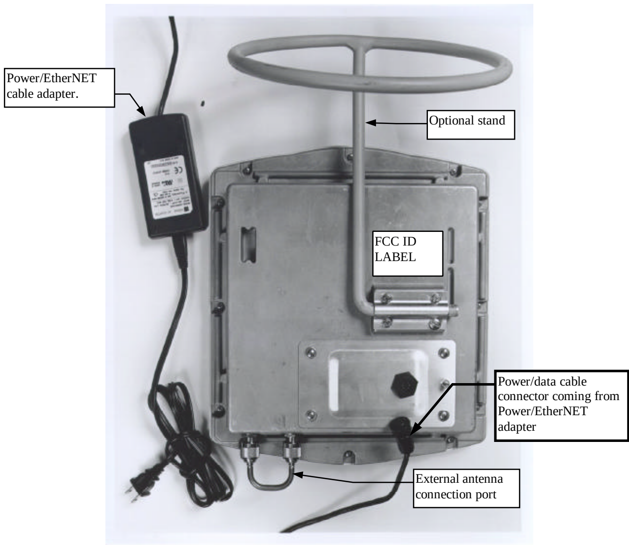
Photo Shows rear outside view of Wireless Modem(xDR232)
