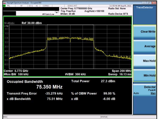
Plot 7-185. 6dB BW & 99% OBW Antenna 3b (80MHz BW 802.11ac - Ch. 155, MCS2)
