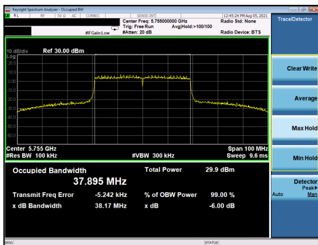
Plot 7-202. 6dB BW & 99% OBW Antenna 1b (40MHz BW 802.11ax(SU) - Ch. 151, MCS2)
