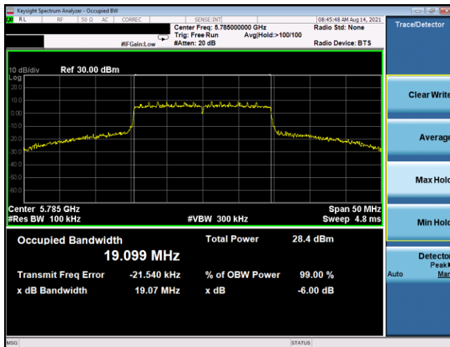
Plot 7-176. 6dB BW & 99% OBW Antenna 5T (20MHz BW 802.11ax(SU) – Ch. 157, MCS5)
