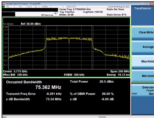
Plot 7-203. 6dB BW & 99% OBW Antenna 1b (80MHz BW 802.11ac - Ch. 155, MCS2)
