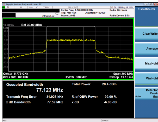
Plot 7-204. 6dB BW & 99% OBW Antenna 1b (80MHz BW 802.11ax(SU) - Ch. 155, MCS2)
