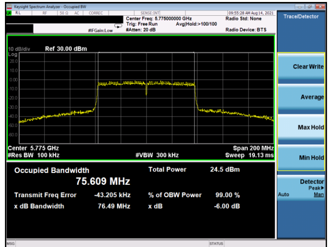
Plot 7-215. 6dB BW & 99% OBW Antenna 1b (80MHz BW 802.11ac - Ch. 155, MCS5)
