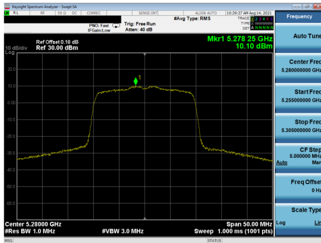
Plot 7-224. PSD Antenna 5T (20MHz BW 802.11ax(SU) – Ch. 56, MCS2)
