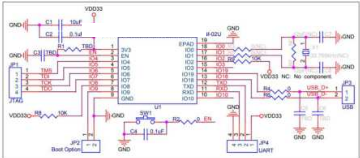
Figure 7 Application Circuit
