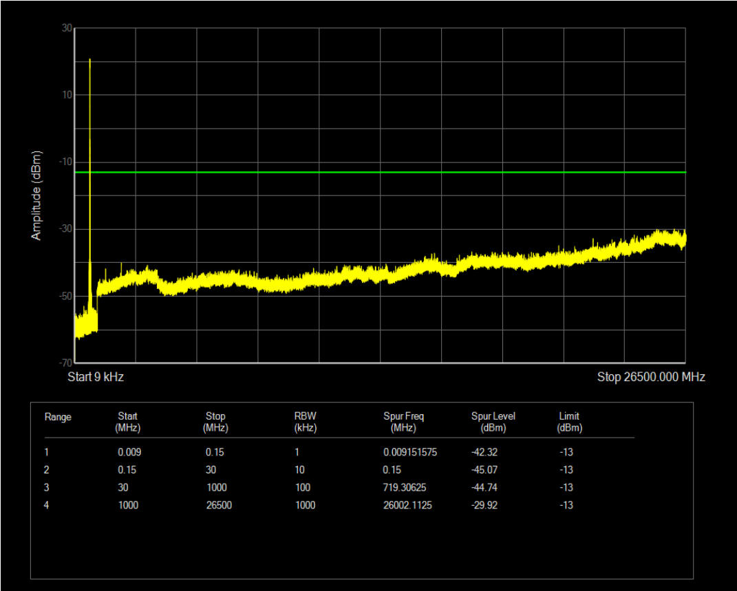
Band71 QPSK Channel=133297 nTones=1@47 Spacing=3.75kHz
