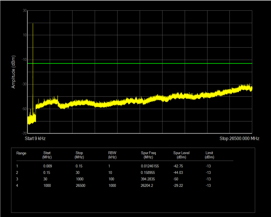
Band71 BPSK Channel=133297 nTones=1@0 Spacing=3.75kHz
