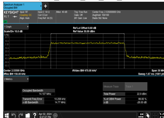
N7(15M)_CP-OFDM_256 QAM_Outer_Full_Mid_CH
