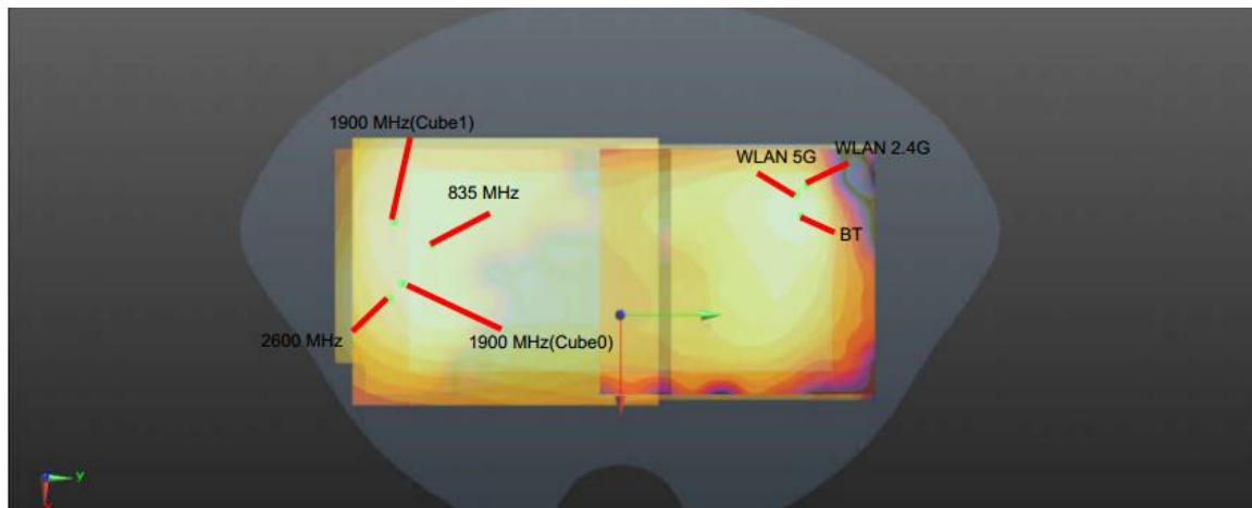
WWAN+ WLAN2.4GHz/ WLAN5GHz/Bluetooth _Back 5mm
