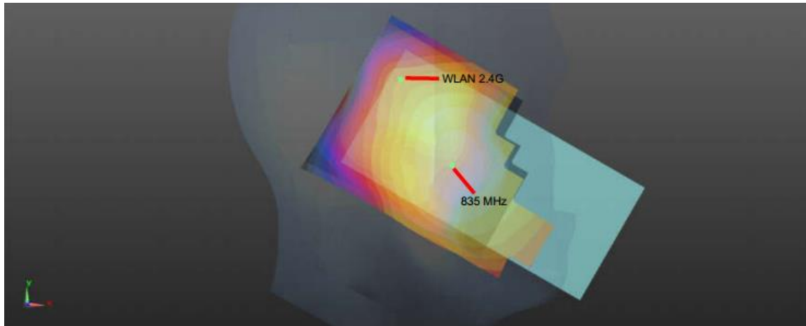
WWAN+WLAN2.4GHz _Left Cheek 0mm
