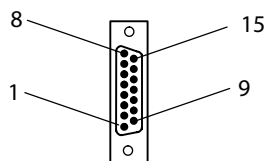
15-Pin DSUB Male
