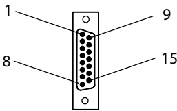
15-Pin DSUB Female
