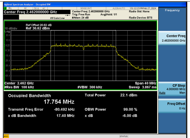
802.11ac_VHT20-CH 11
