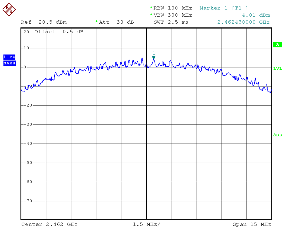
(Plot 2.5 C1: Channel = 11 @ 802.11b)
