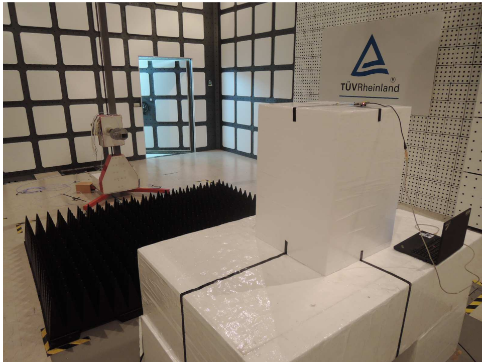
Photograph 5: Set-up for Spurious Emissions (IC)
