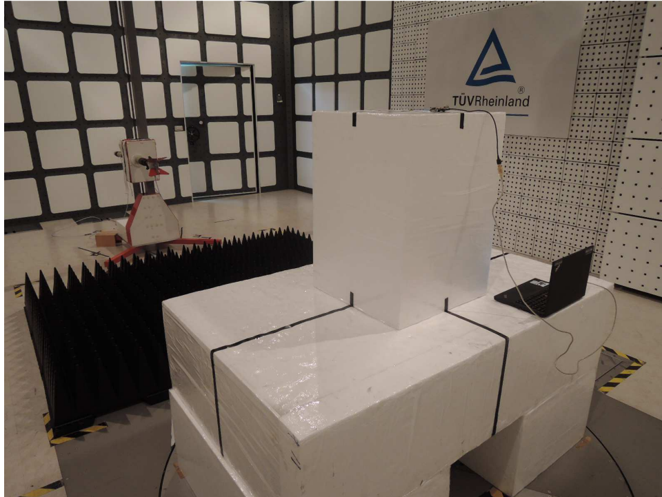
Photograph 4: Set-up for Spurious Emissions (IC)
