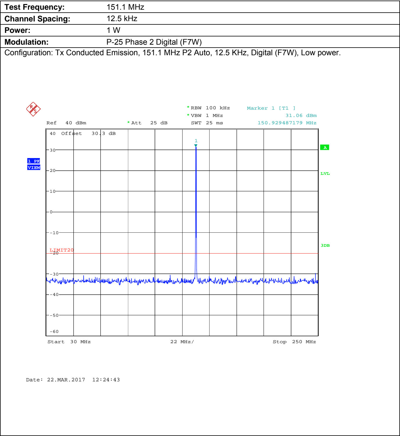
Plot 5.9.4.2.2. Conducted Transmitter Spurious Emissions for 151.1 MHz, Low Power
