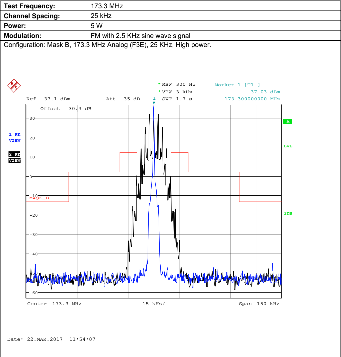
Plot 5.8.4.3.3. Emission Mask B, High Power
