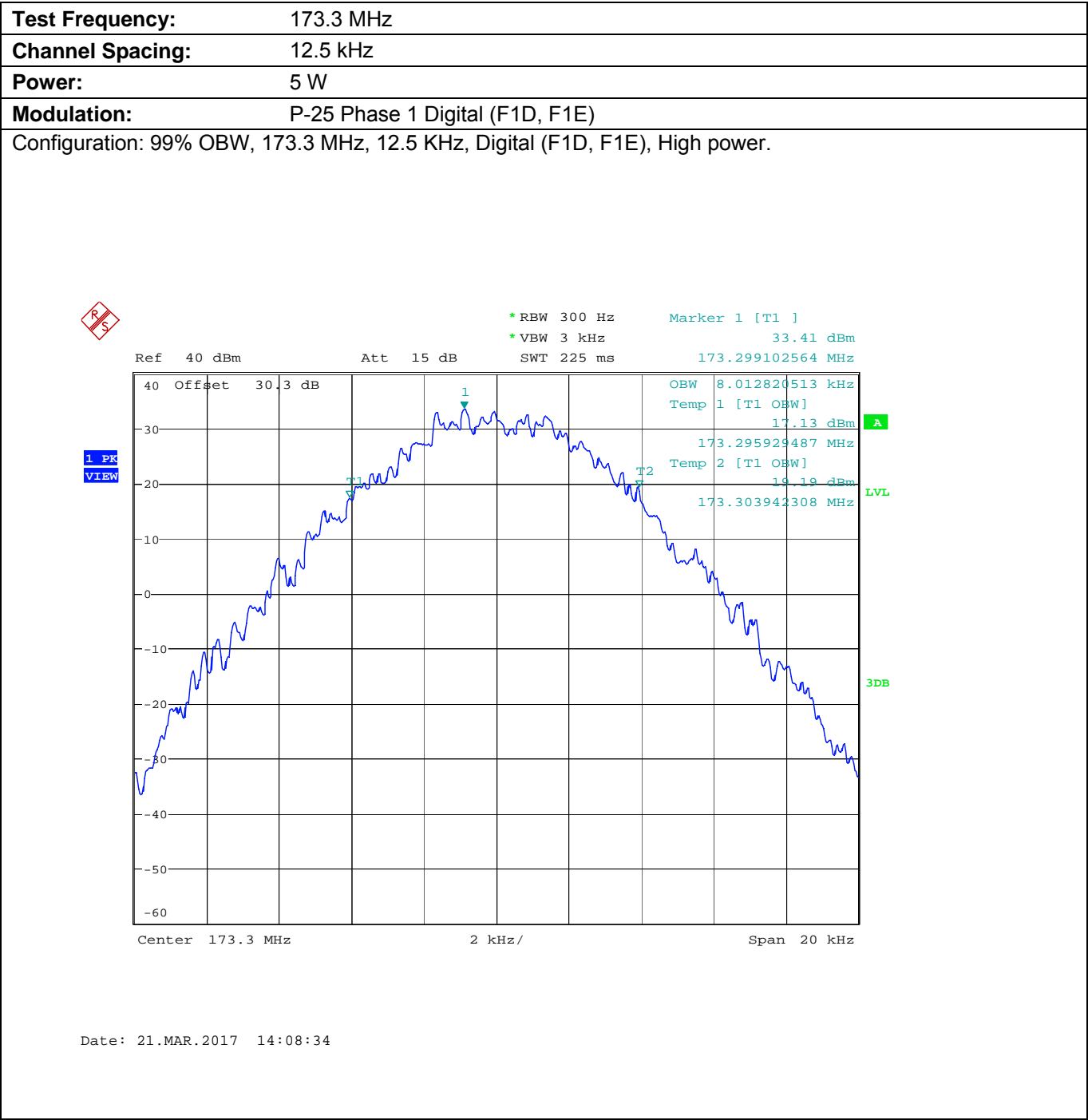
Plot 5.8.4.1.9. Occupied Bandwidth
