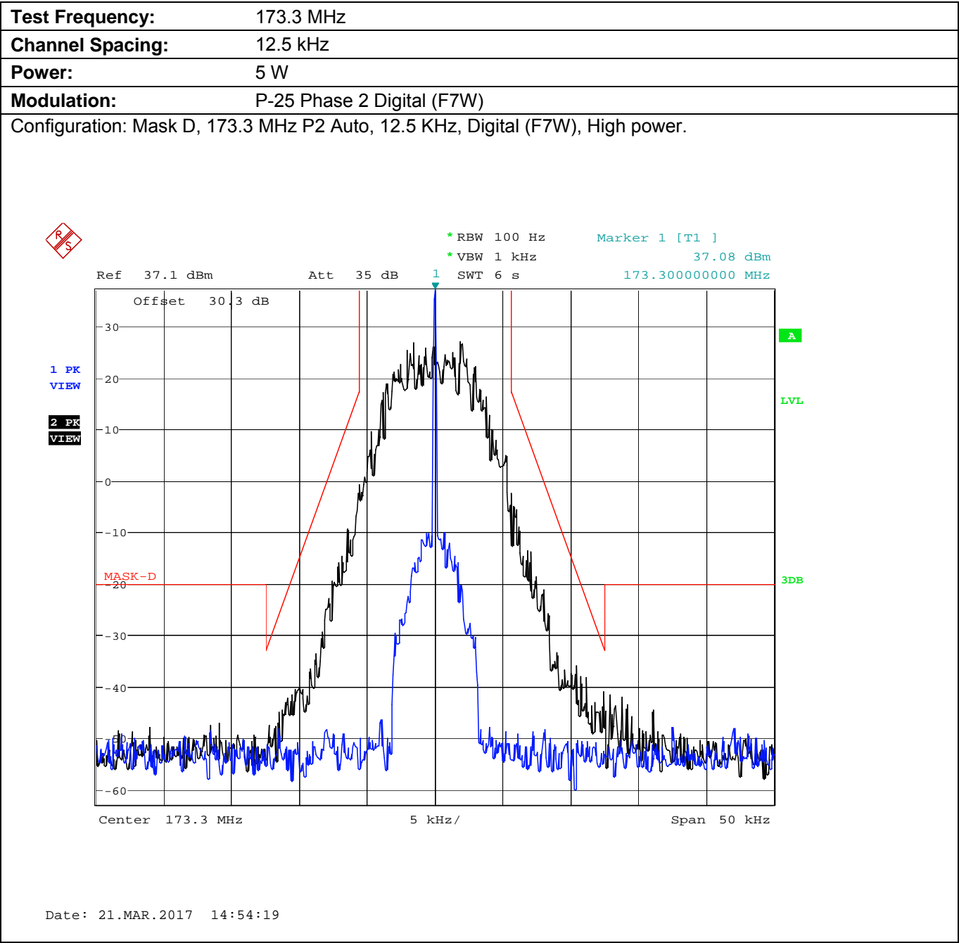
Plot 5.8.4.2.15. Emission Mask D, High Power
