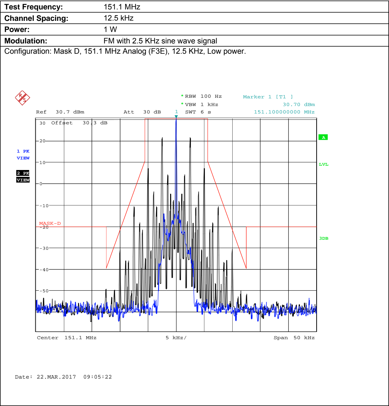
Plot 5.8.4.2.5. Emission Mask D, Low Power
