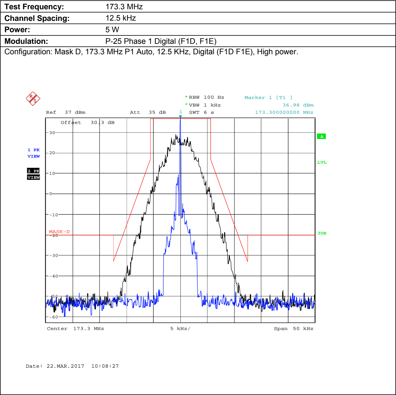
Plot 5.8.4.2.9. Emission Mask D, High Power
