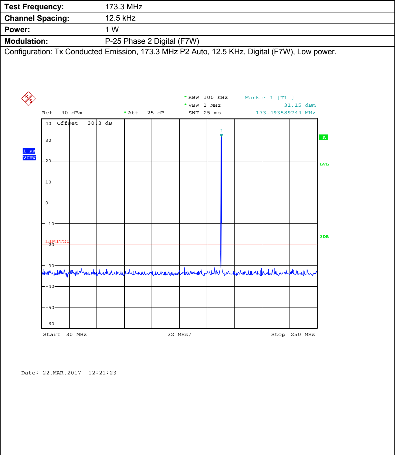
Plot 5.9.4.3.2. Conducted Transmitter Spurious Emissions for 173.3 MHz, Low Power
