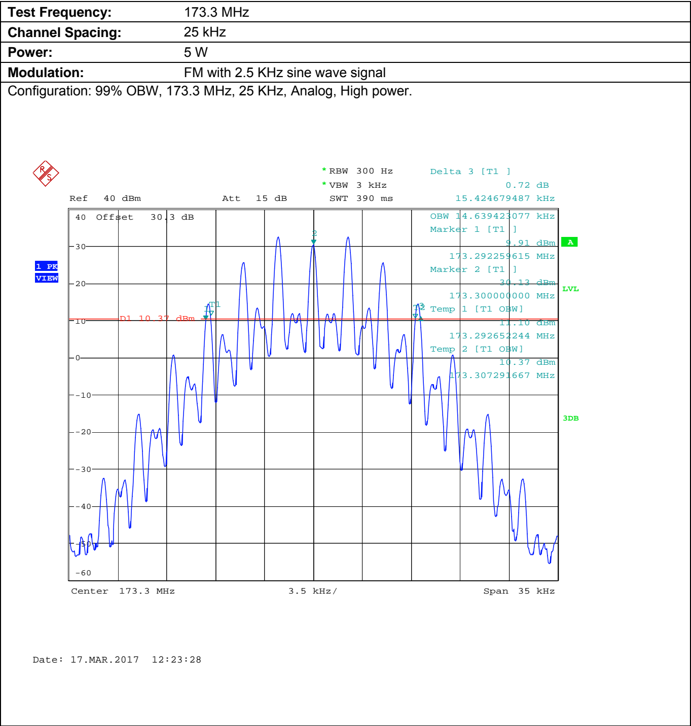
Plot 5.8.4.1.6. Occupied Bandwidth
