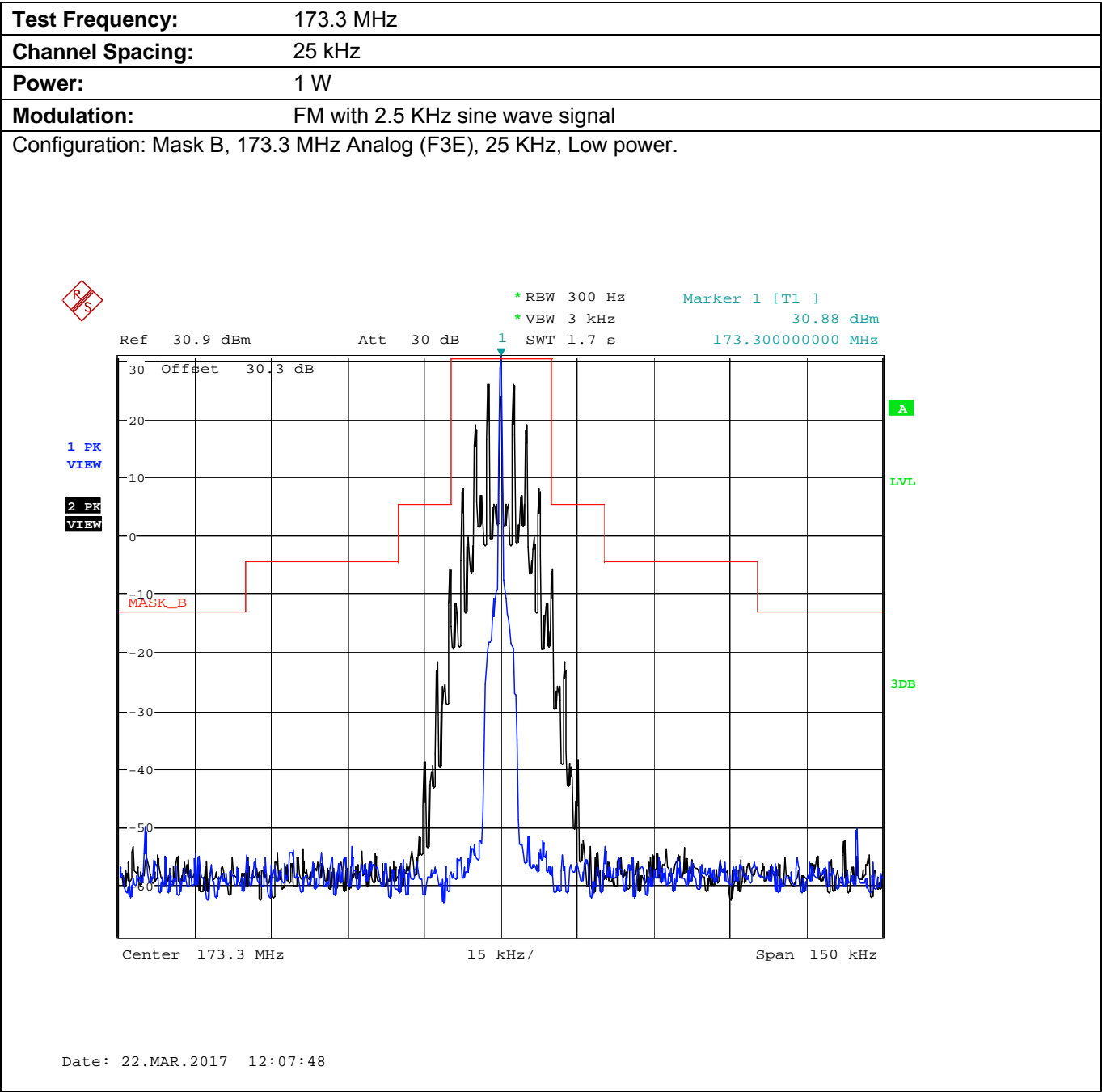
Plot 5.8.4.3.6. Emission Mask B, Low Power
