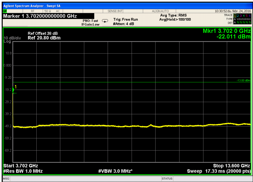
Figure 239.— 10MHz CBW -3702.0MHz -13.6GHz band, top frequency, 64QAM
