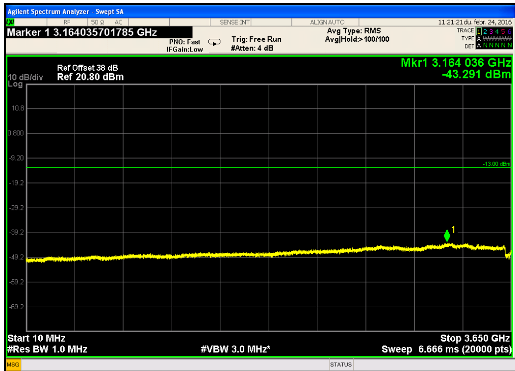
Figure 277.— 15MHz CBW -10.0MHz-3650.0MHz band, top frequency, QPSK
