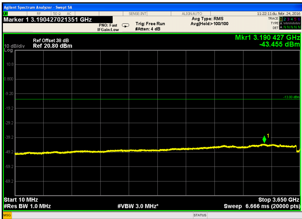
Figure 267.— 15MHz CBW - 10.0MHz-3650.0MHz band, top frequency, 64QAM
