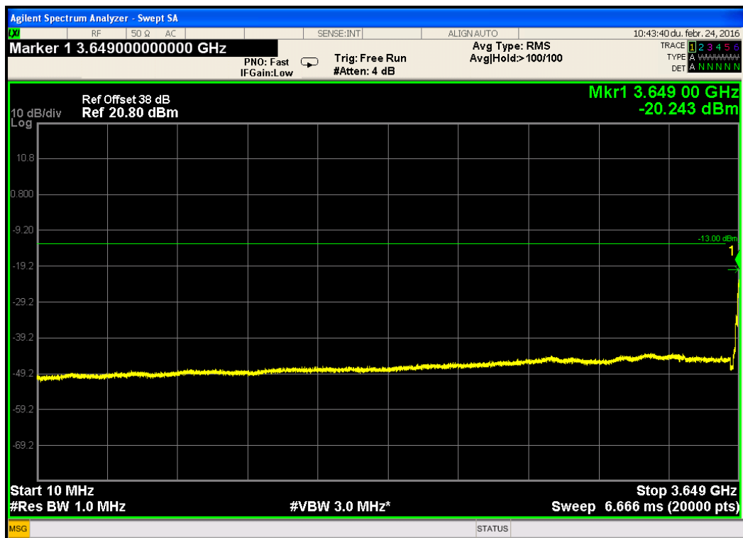
Figure 257. — 15MHz CBW - 10.0MHz-3649.0MHz band, bottom frequency, 16QAM
