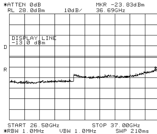
Figure 260. — 15MHz CBW - 13.6GHz-26.5GHz band, bottom frequency, 16QAM
