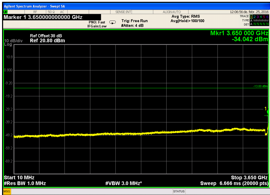
Figure 307.— 20MHz CBW - 10.0MHz-3650.0MHz band, top frequency, QPSK
