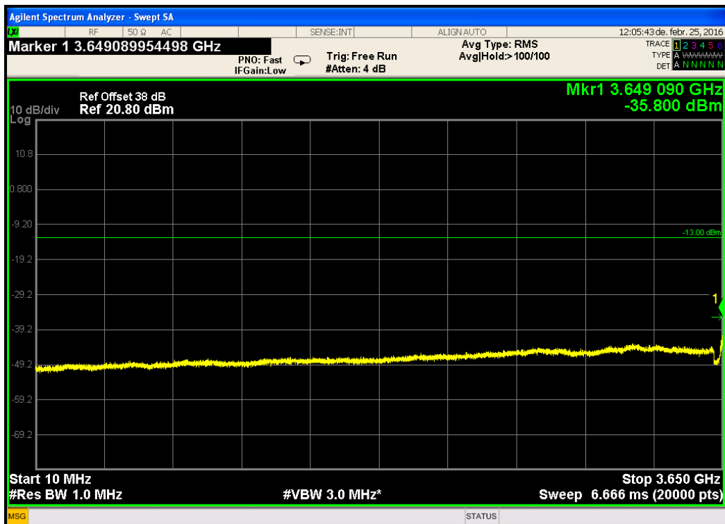
Figure 297.— 20MHz CBW - 10.0MHz-3650.0MHz band, top frequency, 64QAM
