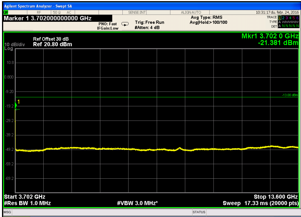
Figure 244.— 10MHz CBW - 3702.0MHz -13.6GHz band, top frequency, 16QAM
