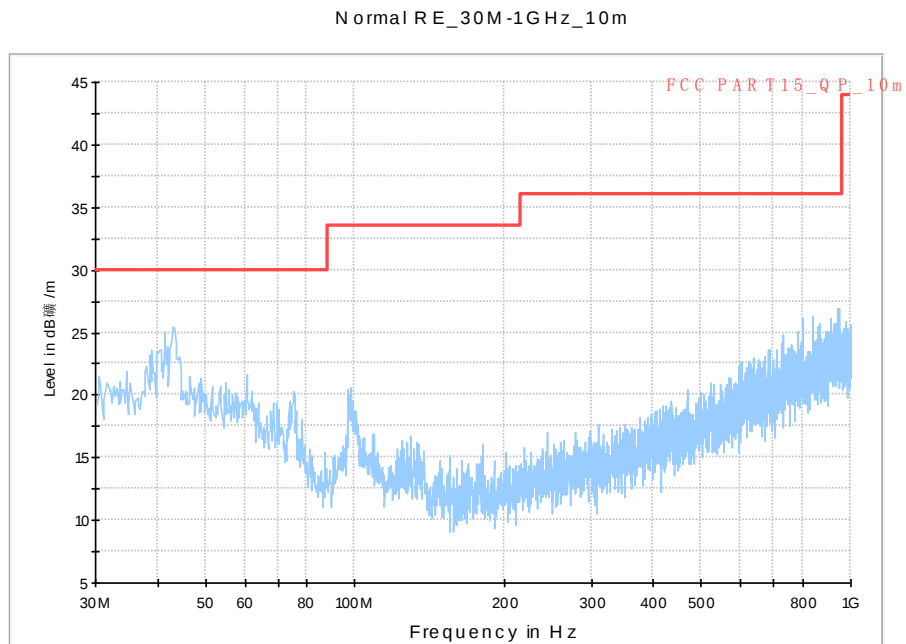
Fig.A.6.2.4 Transmitter Spurious Emission - Radiated (802.11b, Ch6, 30 MHz-1 GHz)
