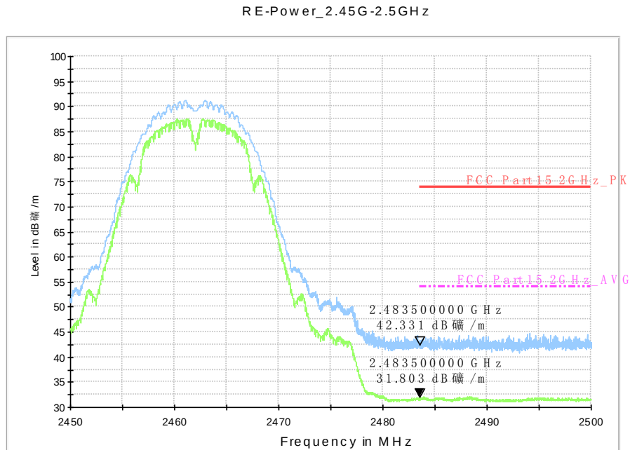
Fig.A.6.2.8 Transmitter Spurious Emission - Radiated (Power): 802.11b, ch11, 2.45 GHz - 2.50GHz
