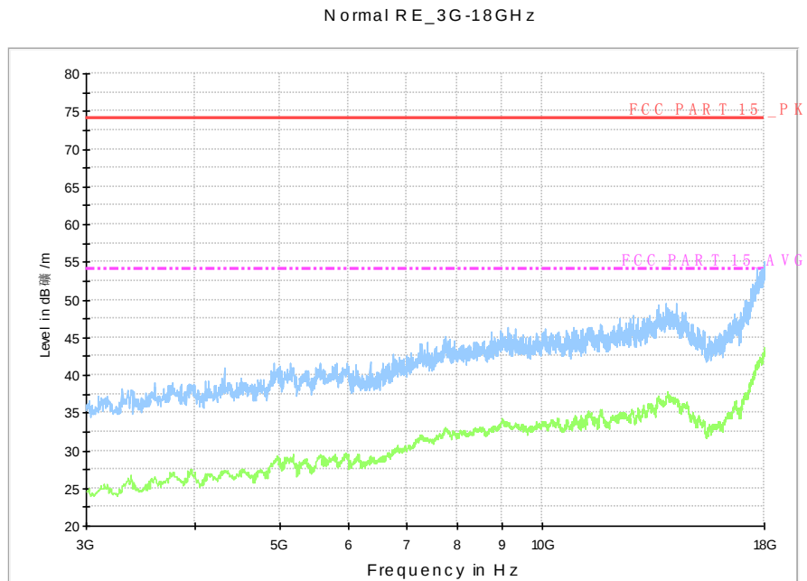
Fig.A.6.2.33 Transmitter Spurious Emission - Radiated (802.11n-HT40, ch3, 3 GHz-18 GHz)
