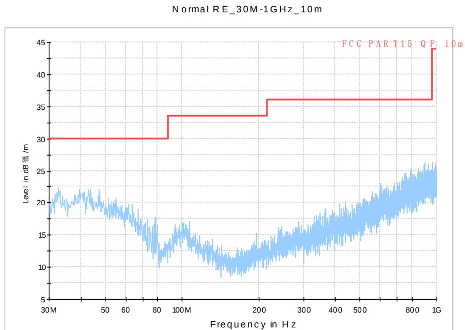
Fig.A.6.2.34 Transmitter Spurious Emission - Radiated (802.11n-HT40, Ch6, 30 MHz-1 GHz)
