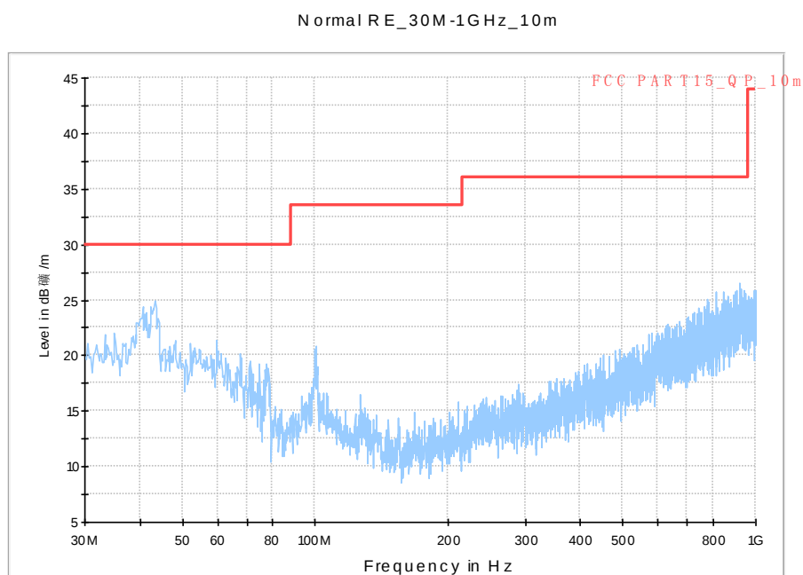
Fig.A.6.2.14 Transmitter Spurious Emission - Radiated (802.11g, Ch6, 30 MHz-1 GHz)
