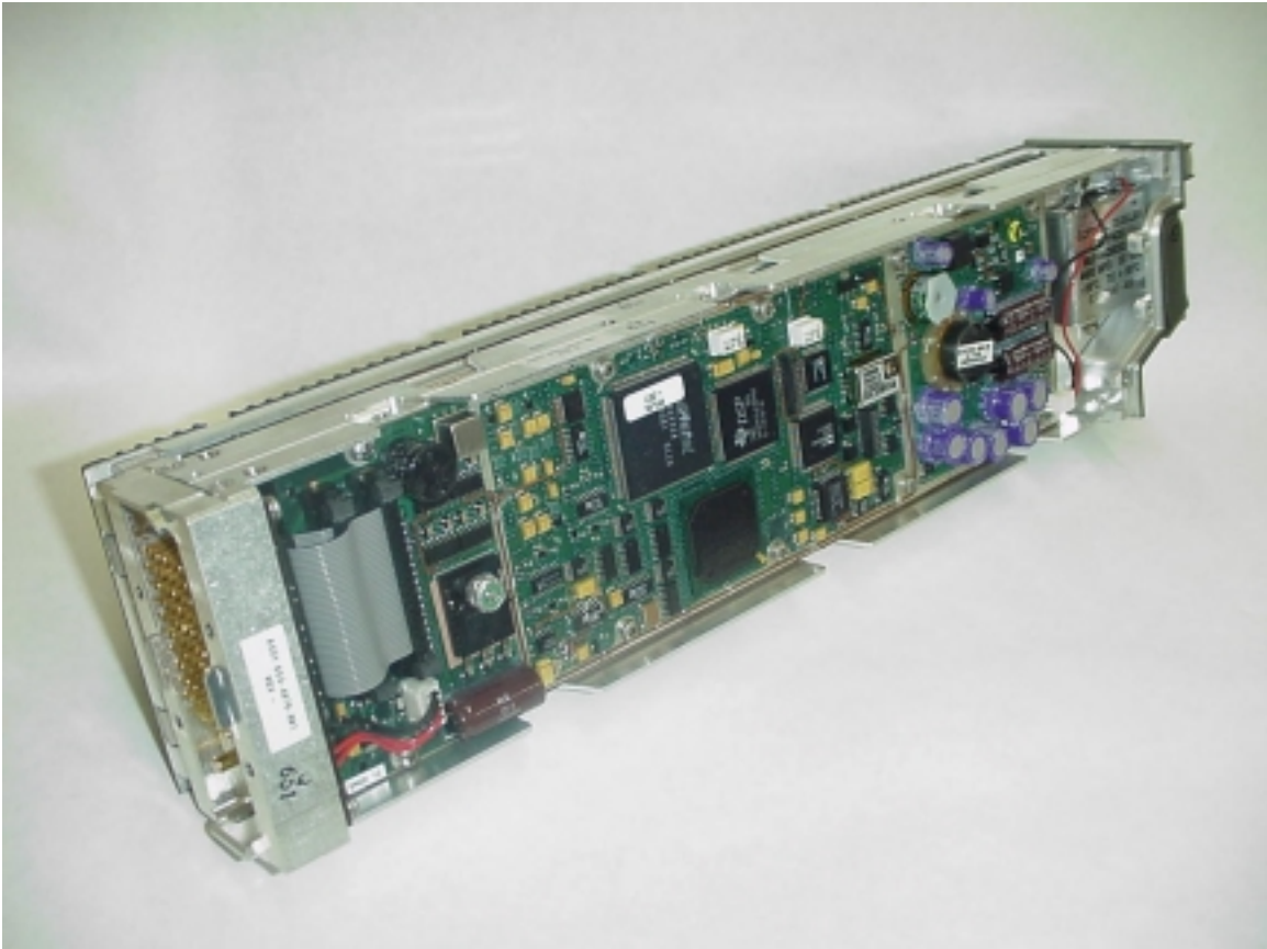
Photo 6: Assembled VHF-4000, with cover removed. View of DSP/Power Supply Circuit Card side
