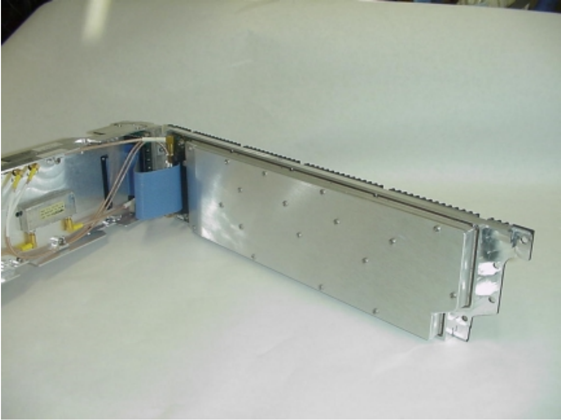
Photo 8: View of RF Circuit Card in shielded assembly.
