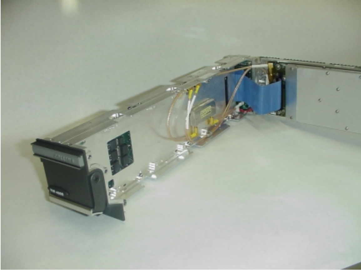
Photo 7: Open Chassis view of VHF-4000 showing RF card assembly on the right, interconnections, and chassis web under DSP/Power Supply. The Connectorized component at middle right is a lowpass filter in both receive and transmit paths. See circuit description, exhibit L.
