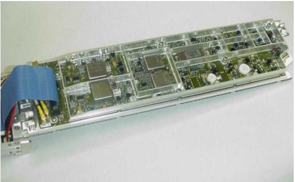
Photo 9: View of RF Circuit Card Assembly, showing placement of shield walls.
