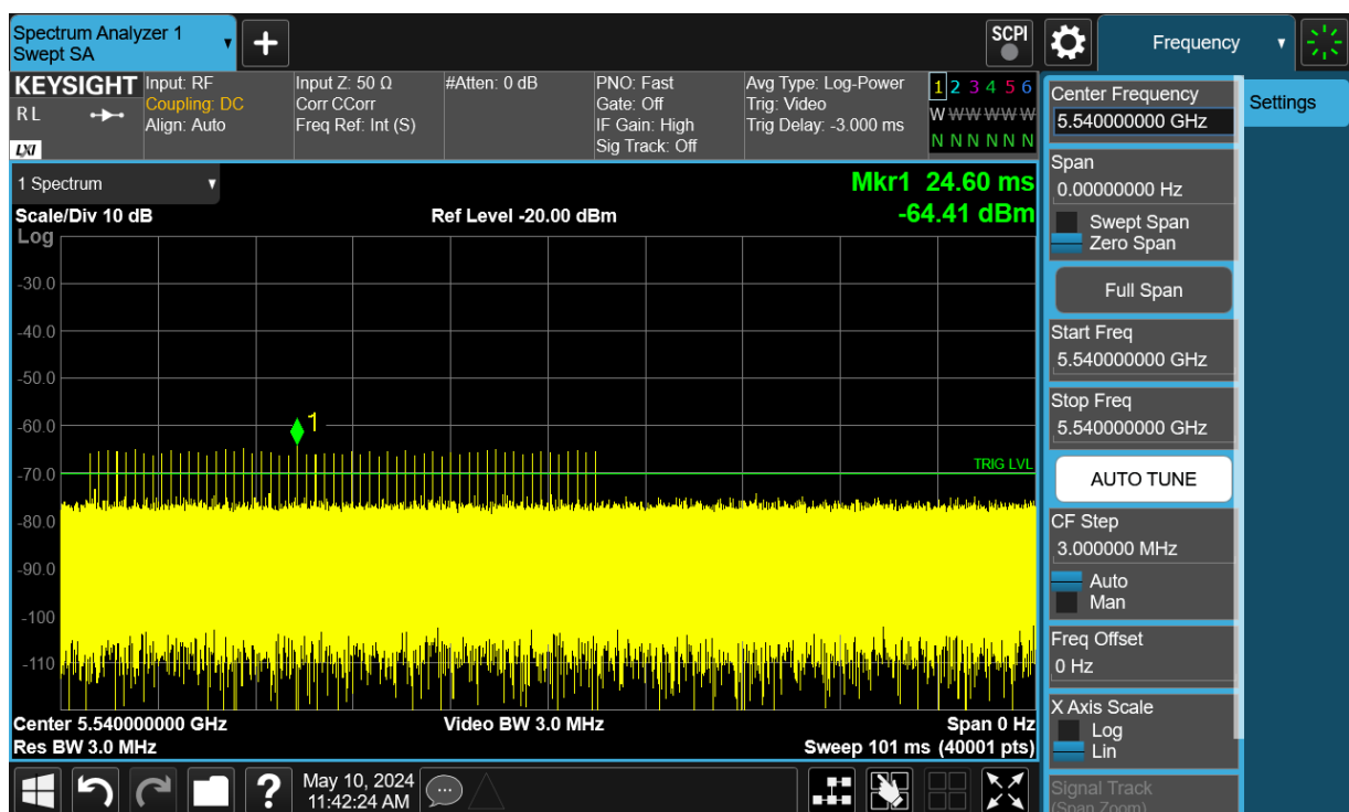
Radar Signal 1
