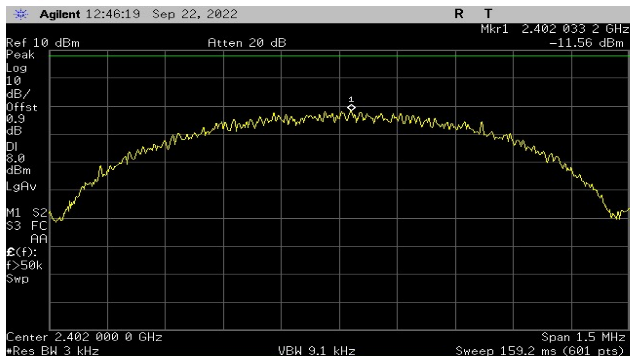
Plot 23 – Power Spectral Density – Lowest Channel
