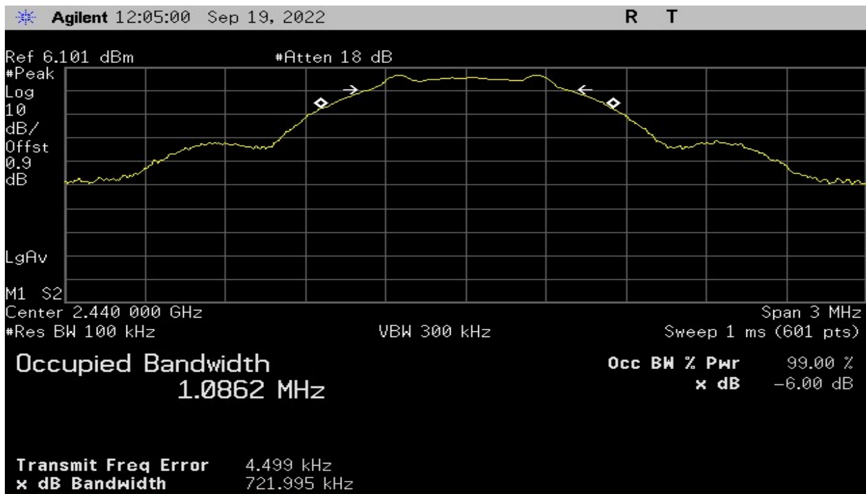
Plot 4 – Middle Channel – 6dB BW
