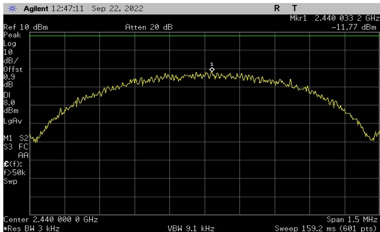
Plot 24 – Power Spectral Density – Middle Channel
