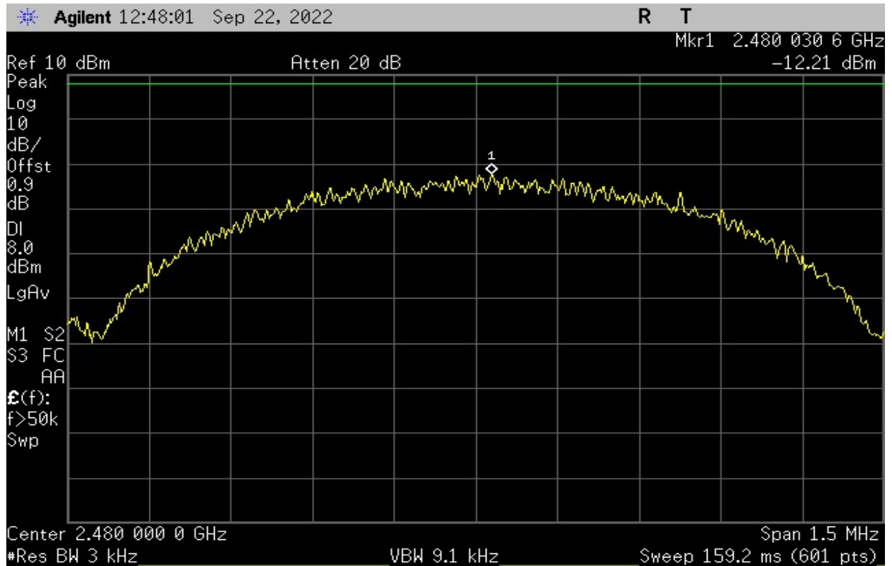
Plot 25 – Power Spectral Density – Highest Channel
