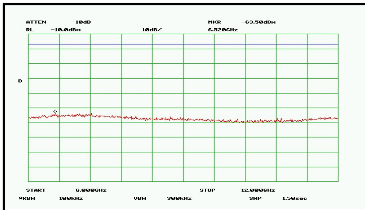
Plot 19 – High Band – 6GHz to 12GHz
