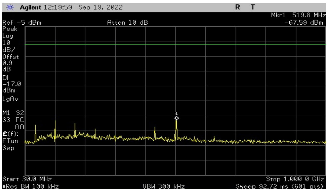
Plot 17 – High Band – 30MHz to 1000MHz
