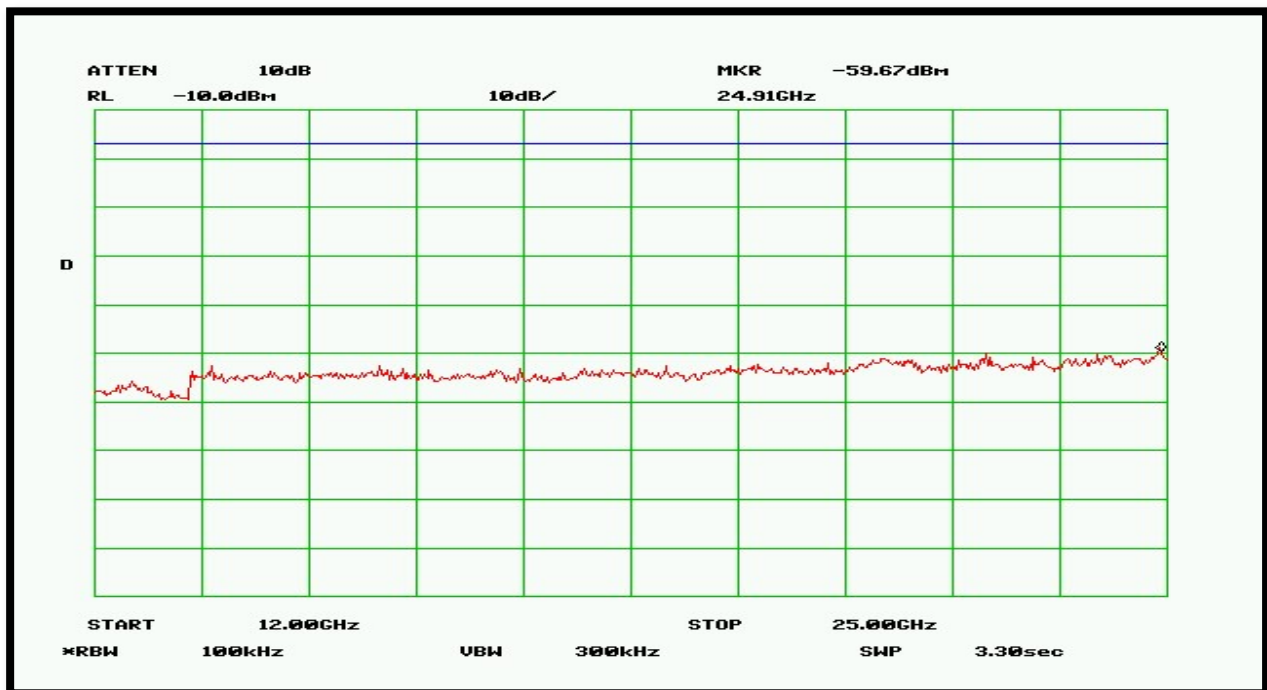
Plot 16 – Mid Band – 12GHz to 25GHz
