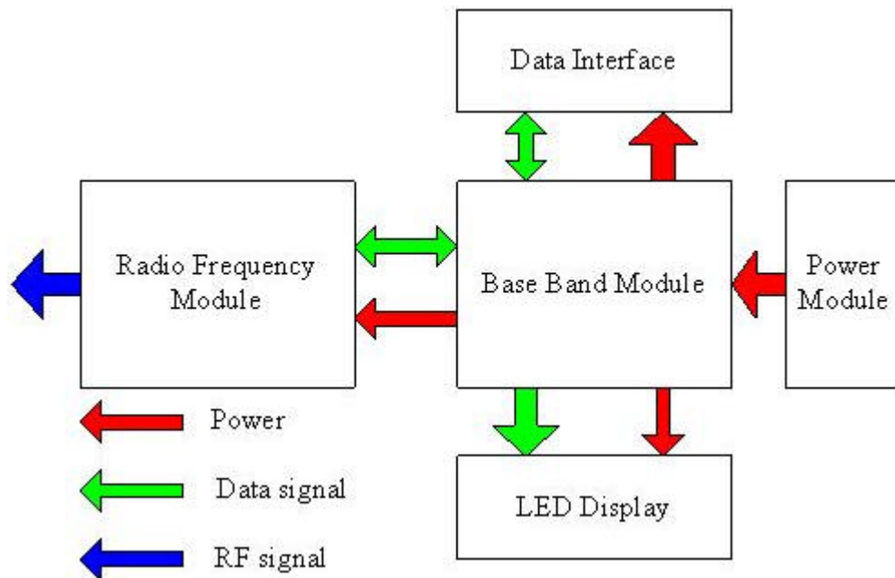
System Module Block Diagram
