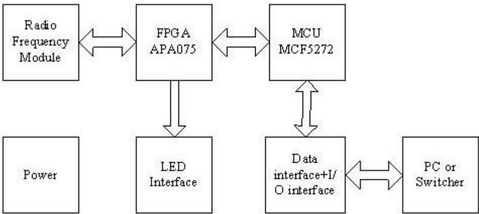
Base Band Module Block Diagram
