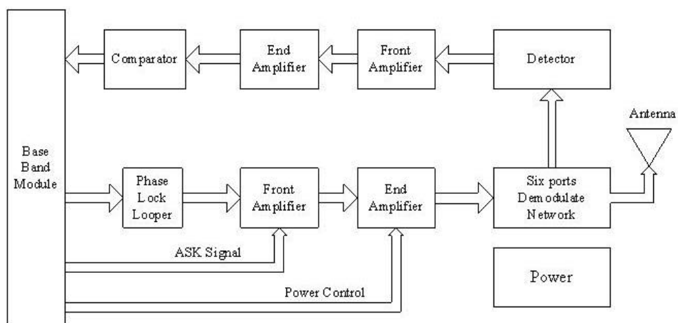
Radio Frequency Module Block Diagram
