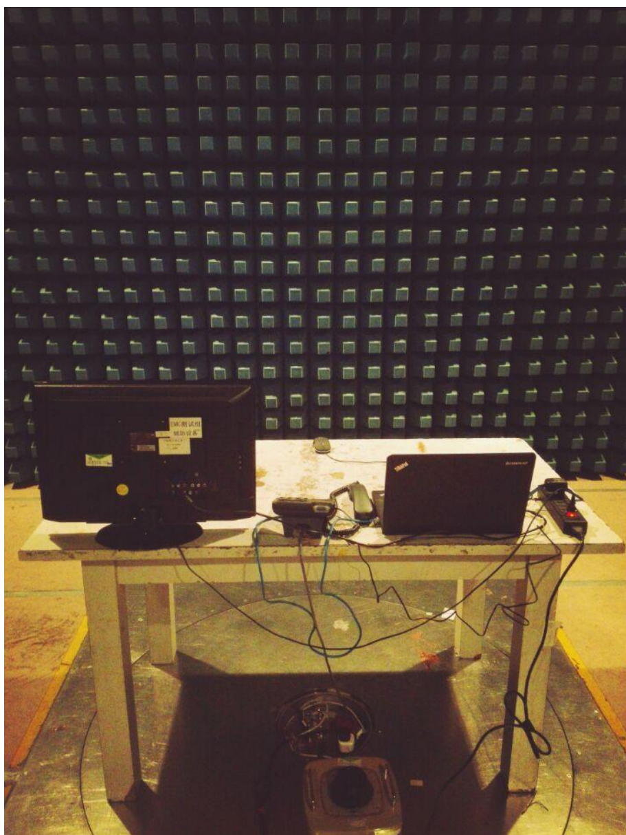
Radiated Emission Test Set-up (Back view)
