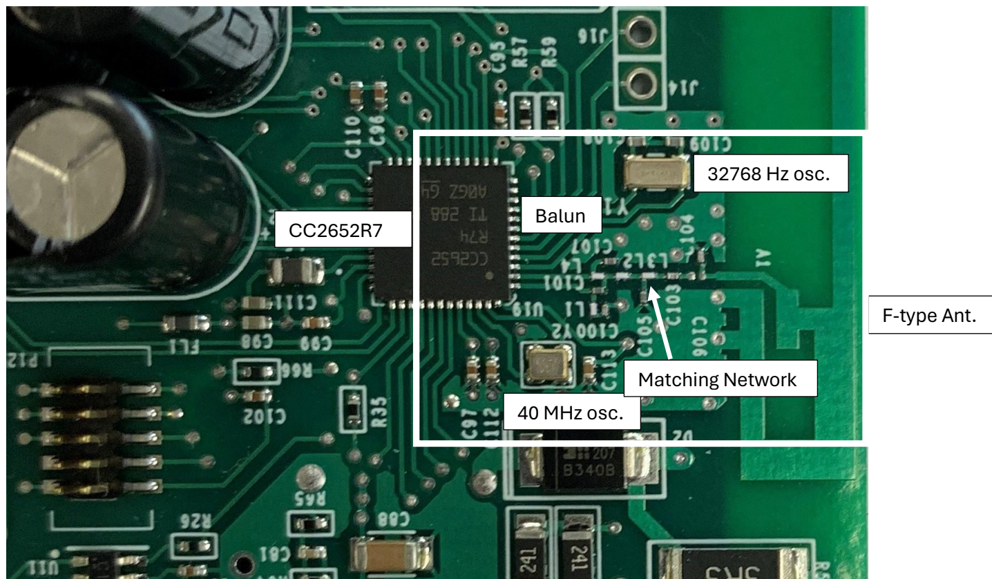
RF section of circuit board
