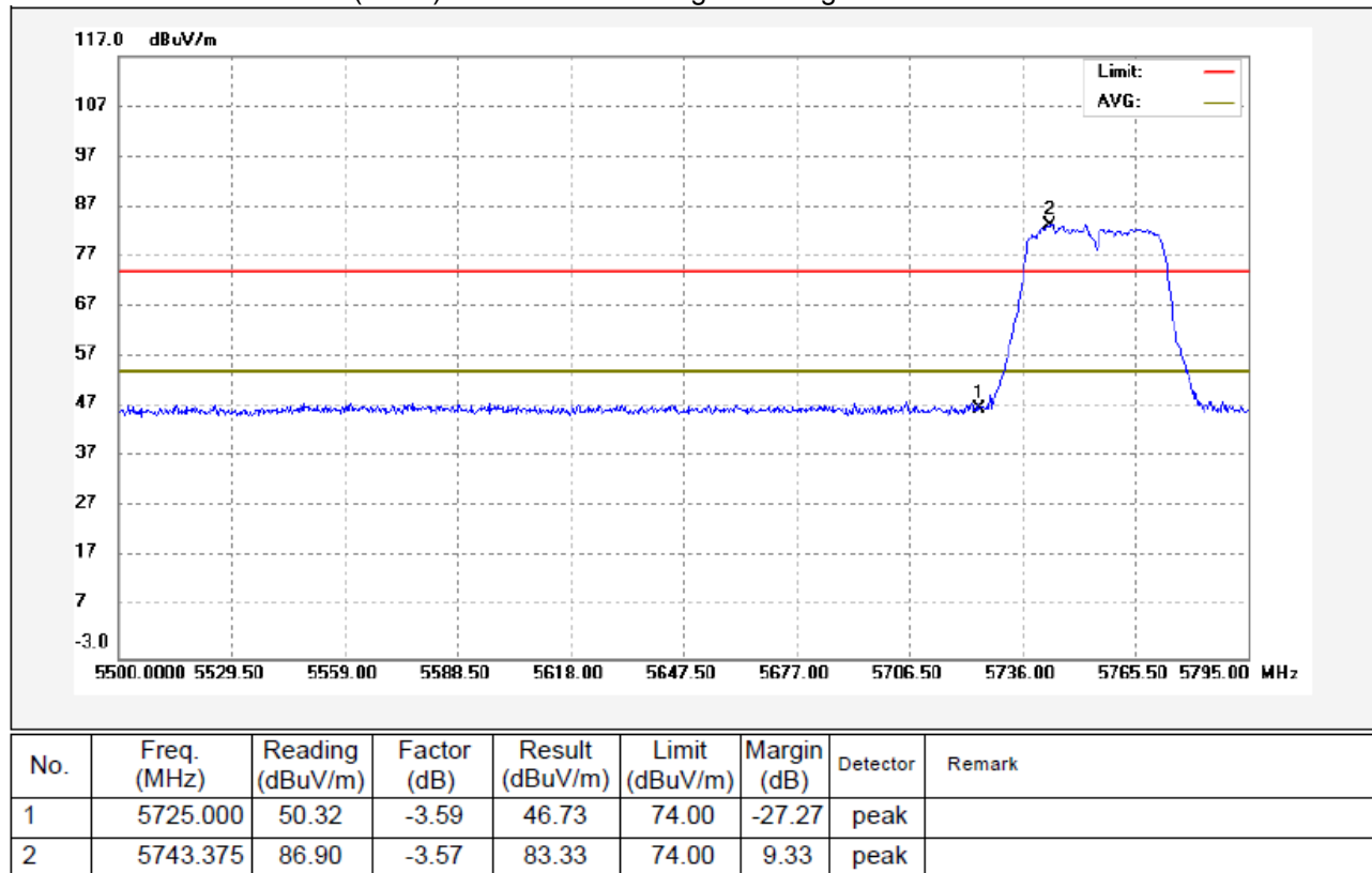
802.11n(HT40) U-NII-3 Transmitting Band edge-right side Vertical
