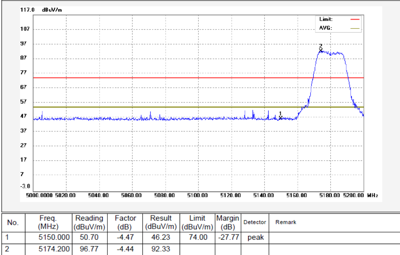
802.11ac(HT20) U-NII-1 Transmitting Band edge-left side Horizontal
