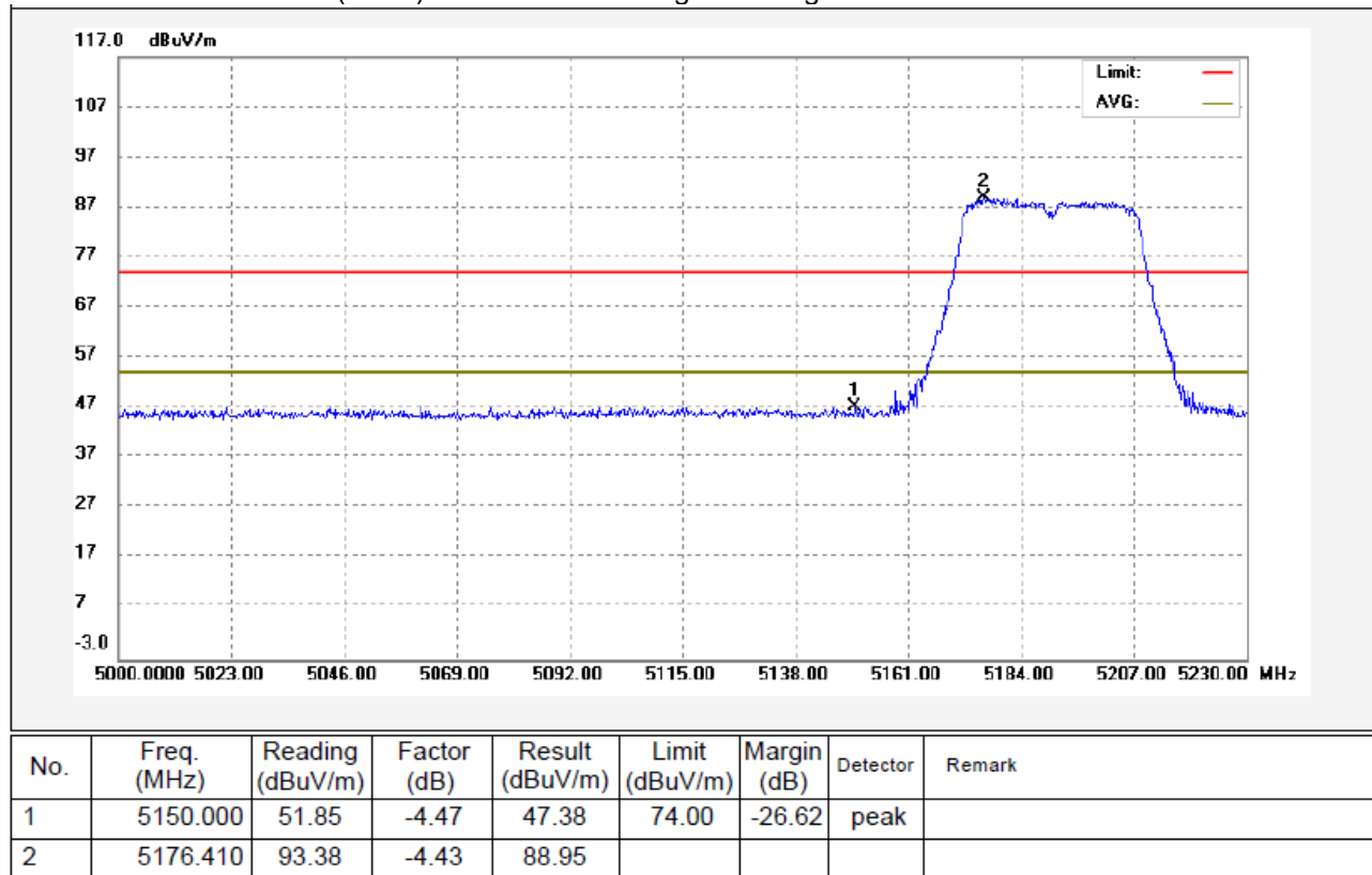
802.11n(HT40) U-NII-1 Transmitting Band edge-left side Horizontal
