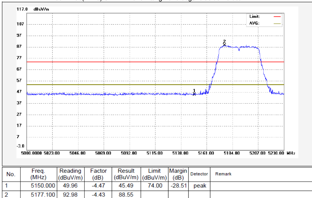
802.11ac(HT40) U-NII-1 Transmitting Band edge-left side Vertical
