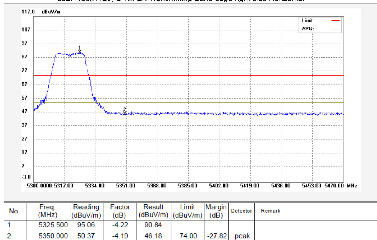
802.11ac(HT20) U-NII-2A Transmitting Band edge-right side Horizontal
