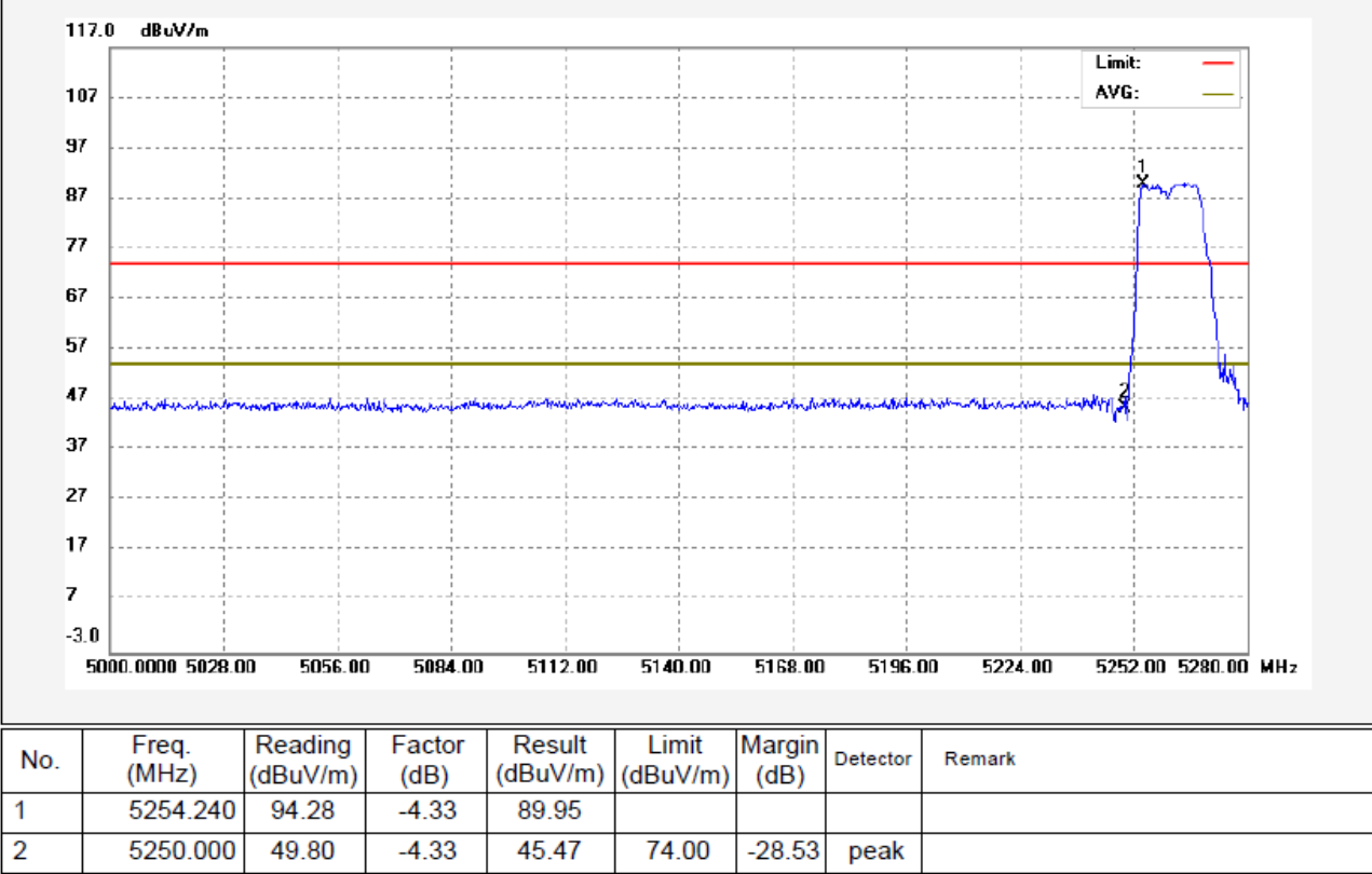
802.11a(HT20) U-NII-2A Transmitting Band edge-left side Horizontal
