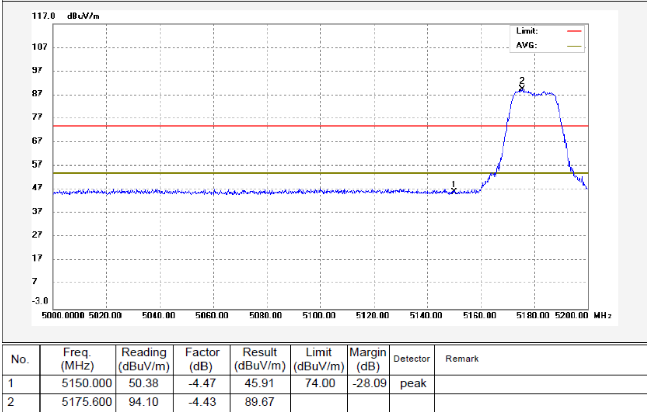
802.11ac(HT20) U-NII-1 Transmitting Band edge-left side Vertical
