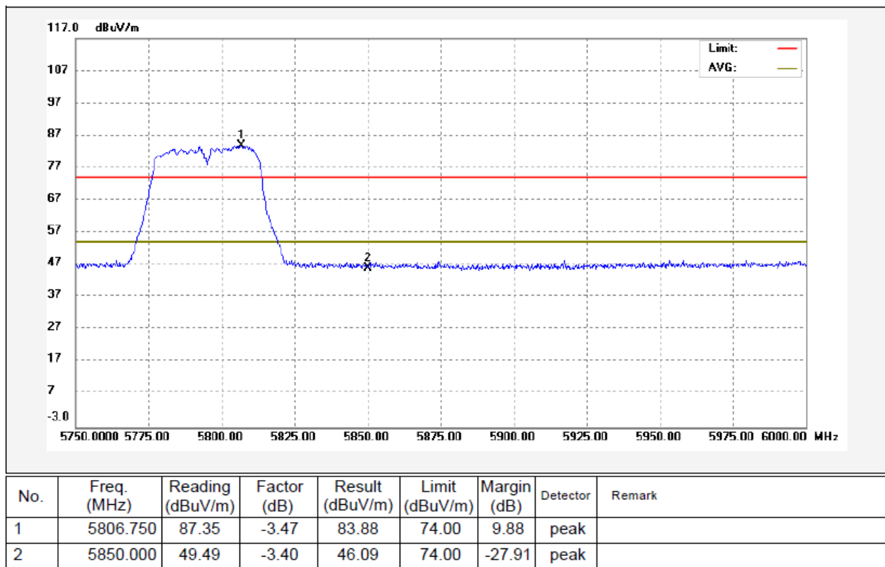
802.11ac(HT40) U-NII-3 Transmitting Band edge-right side Horizontal
