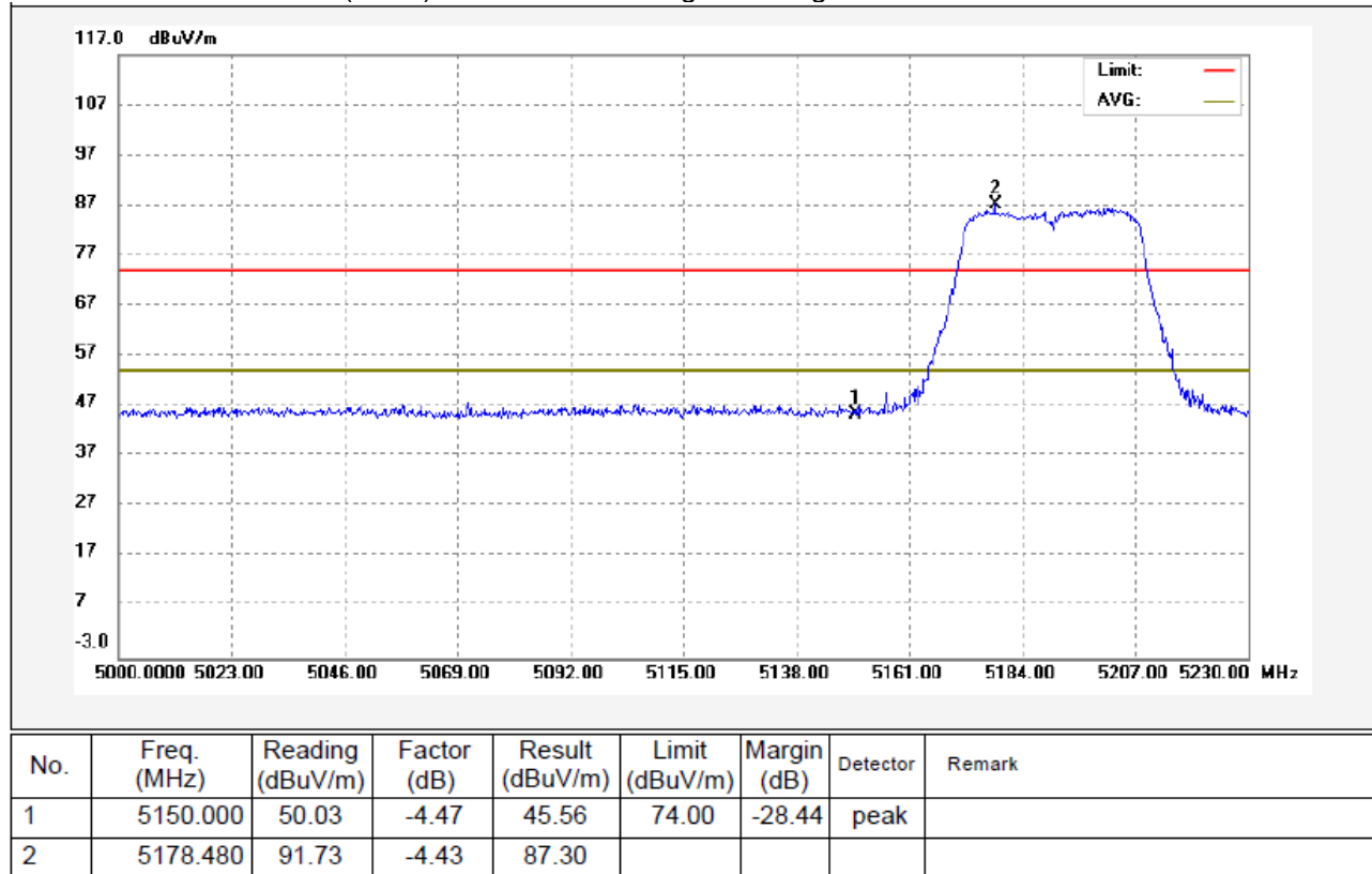
802.11ac(HT40) U-NII-1 Transmitting Band edge-left side Horizontal
