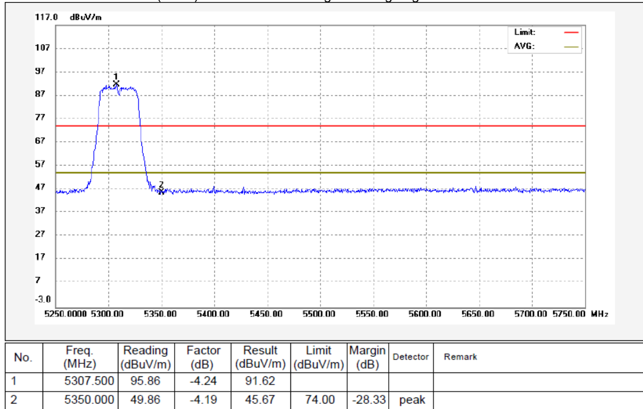
802.11n(HT40) U-NII-2A Transmitting Band edge-right side Vertical
