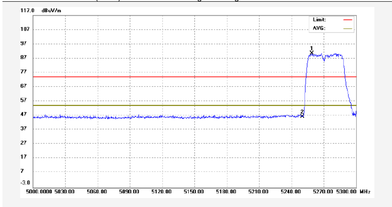
802.11ac(HT40) U-NII-2A Transmitting Band edge-left side Horizontal
