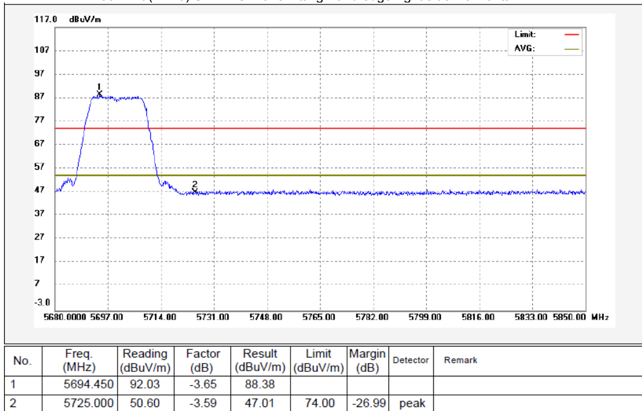
802.11a(HT20) U-NII-2C Transmitting Band edge-right side Horizontal
