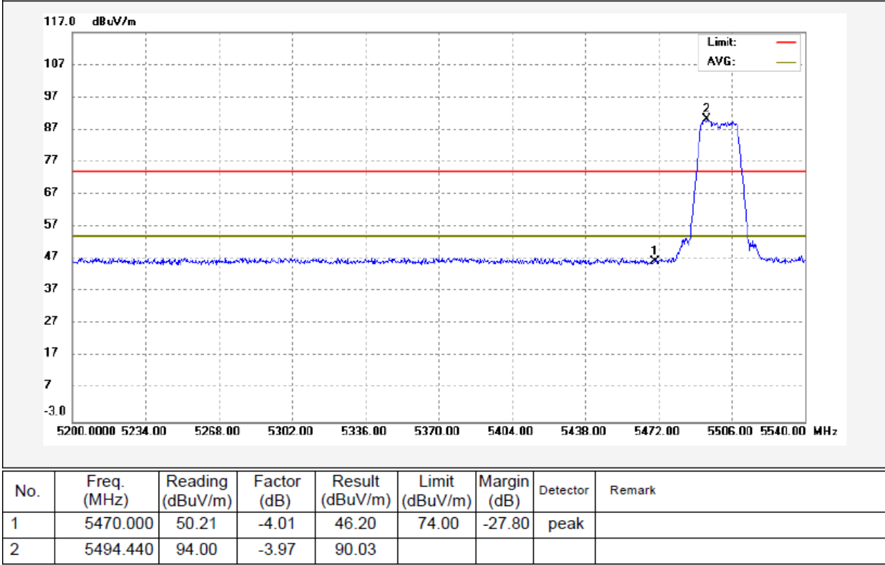
802.11a(HT20) U-NII-2C Transmitting Band edge-left side Vertical
