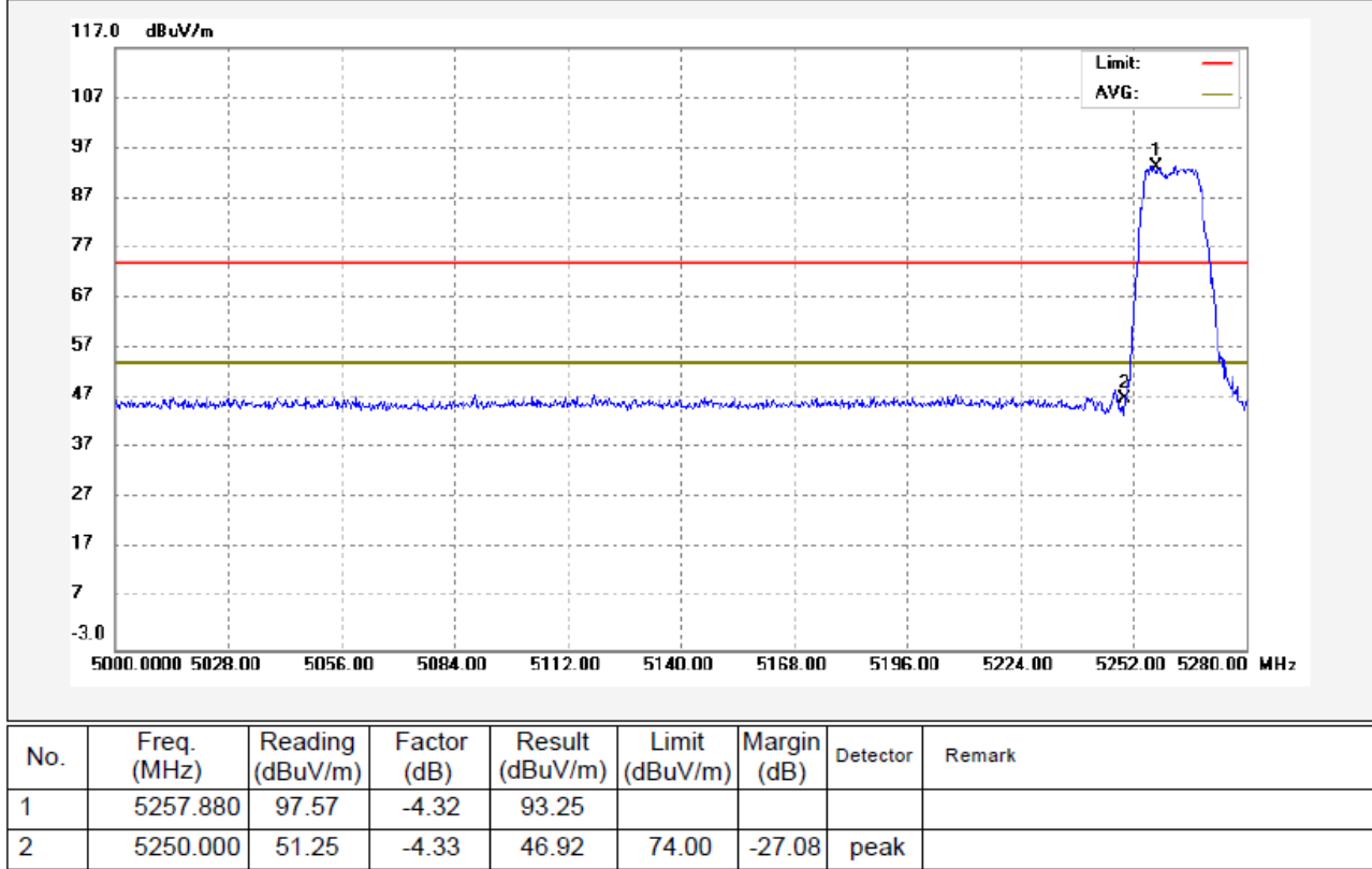
802.11n(HT20) U-NII-2A Transmitting Band edge-left side Vertical
