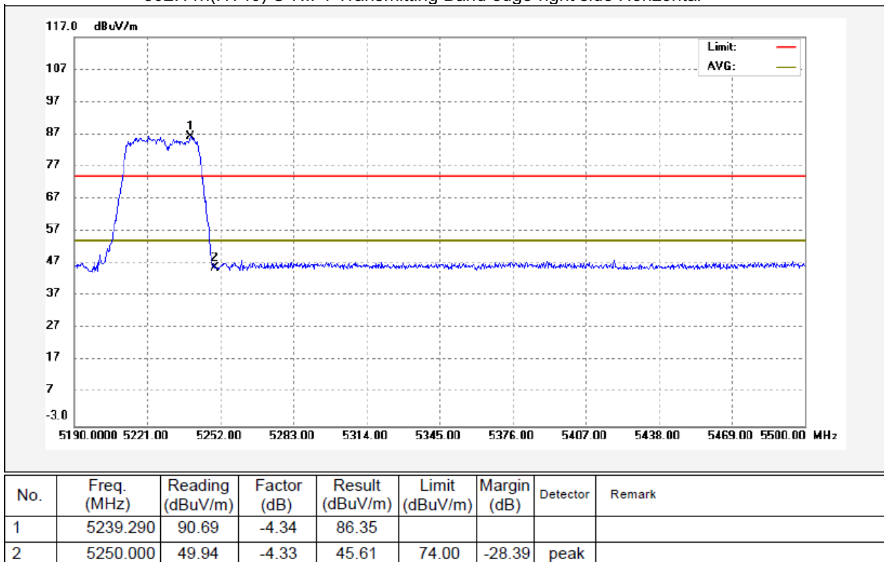
802.11n(HT40) U-NII-1 Transmitting Band edge-right side Horizontal
