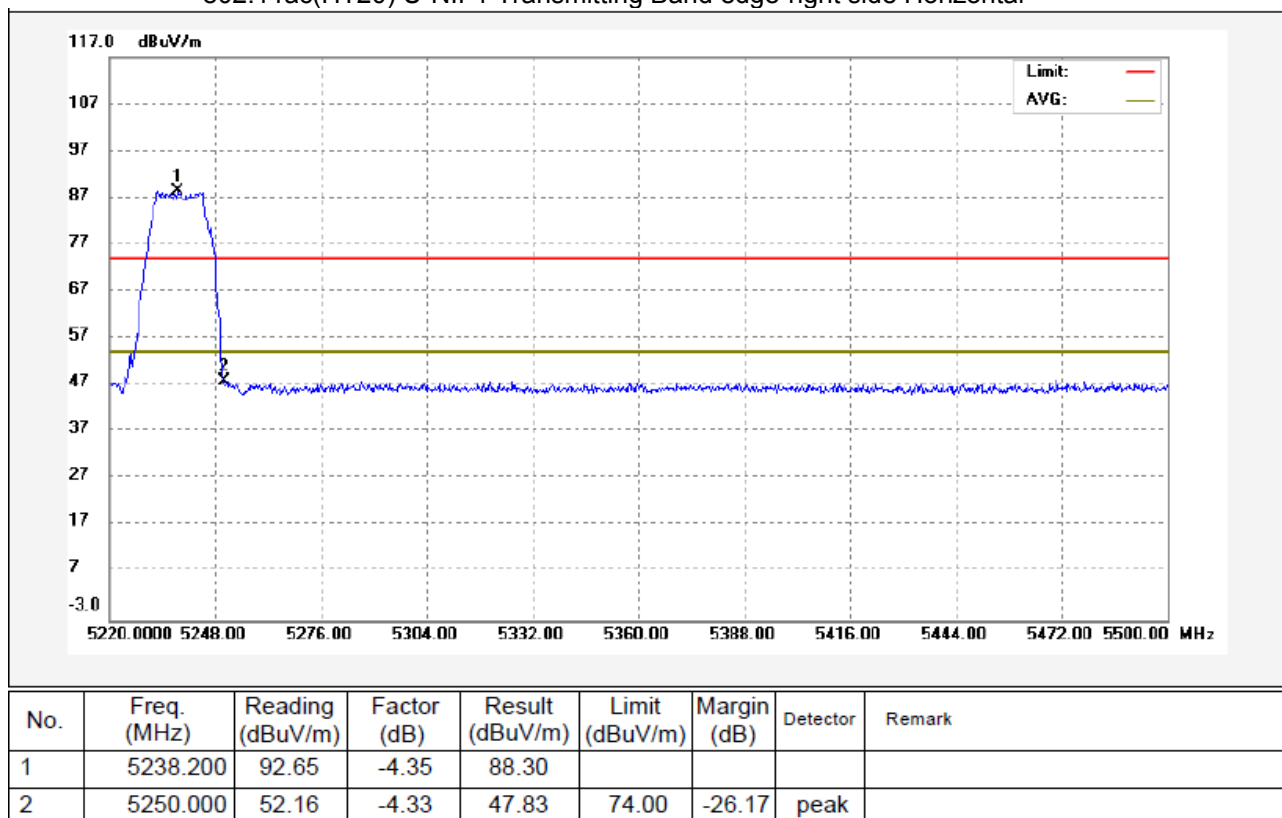
802.11ac(HT20) U-NII-1 Transmitting Band edge-right side Horizontal
