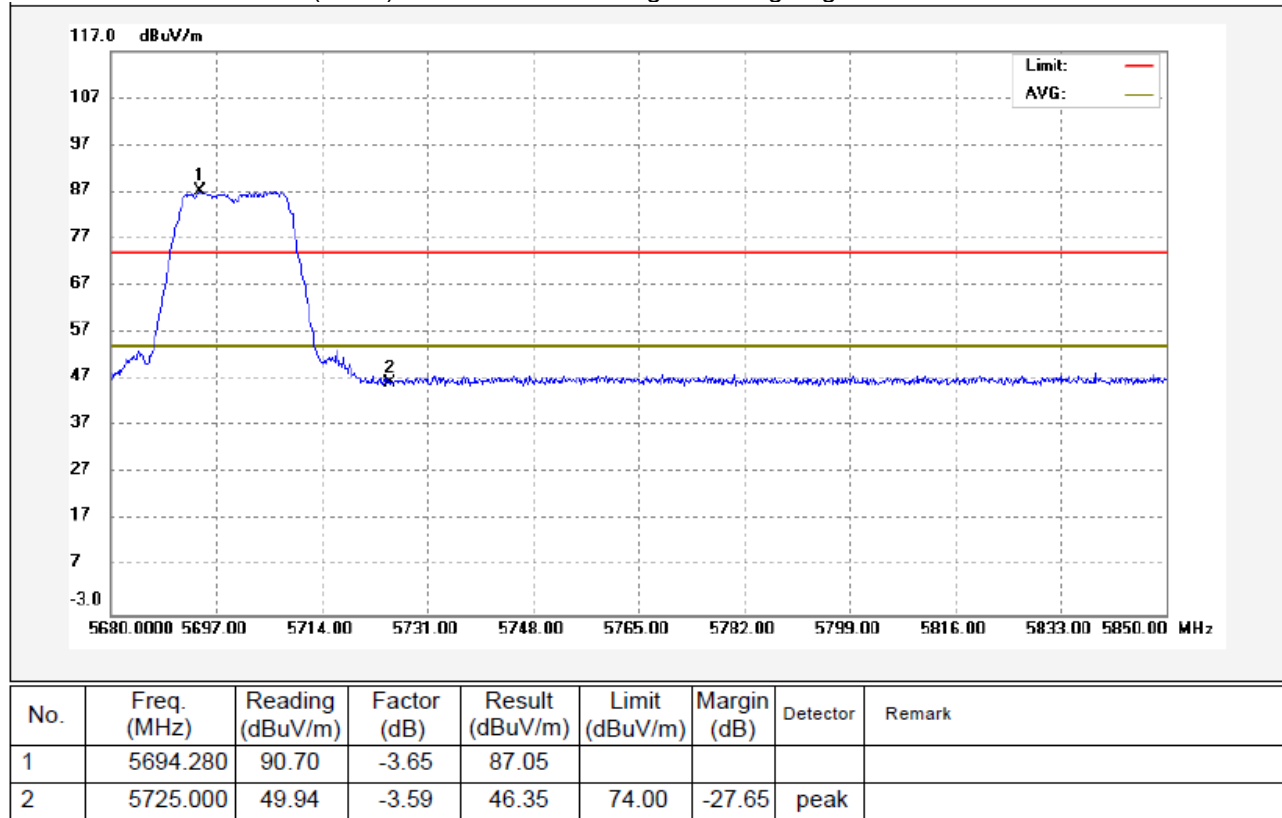
802.11n(HT20) U-NII-2C Transmitting Band edge-right side Vertical
