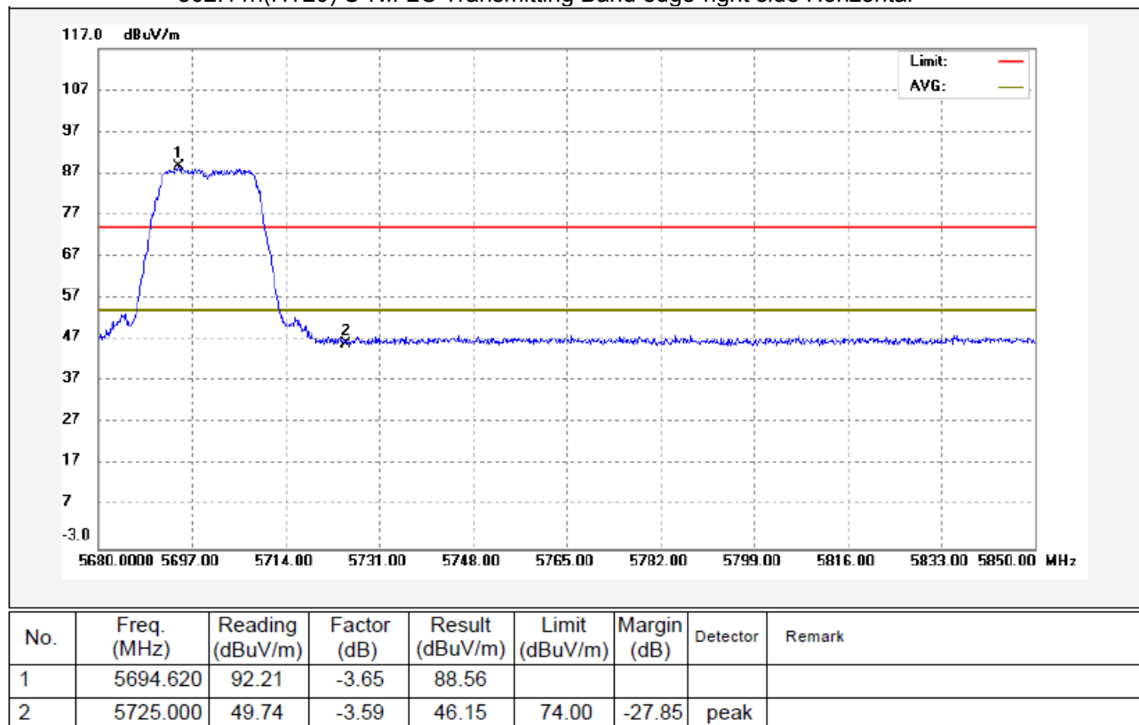
802.11n(HT20) U-NII-2C Transmitting Band edge-right side Horizontal
