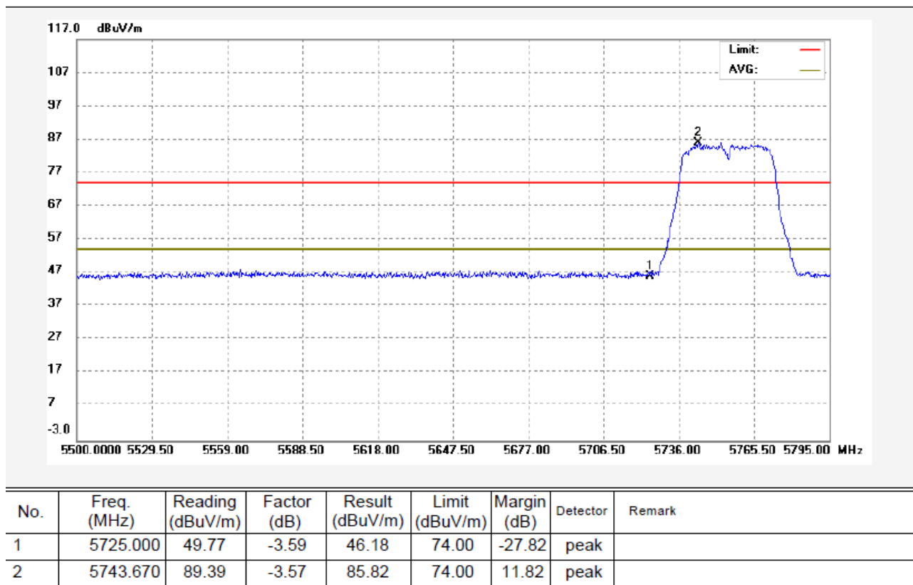
802.11n(HT40) U-NII-3 Transmitting Band edge-left side Vertical
