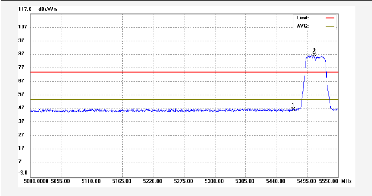
802.11ac(HT40) U-NII-2C Transmitting Band edge-left side Horizontal
