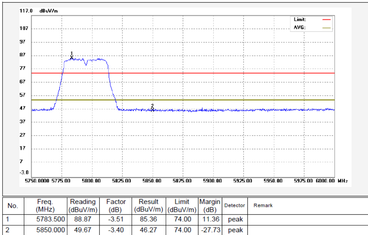
802.11n(HT40) U-NII-3 Transmitting Band edge-right side Horizontal
