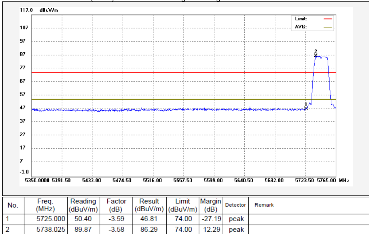
802.11a(HT20) U-NII-3 Transmitting Band edge-left side Horizontal
