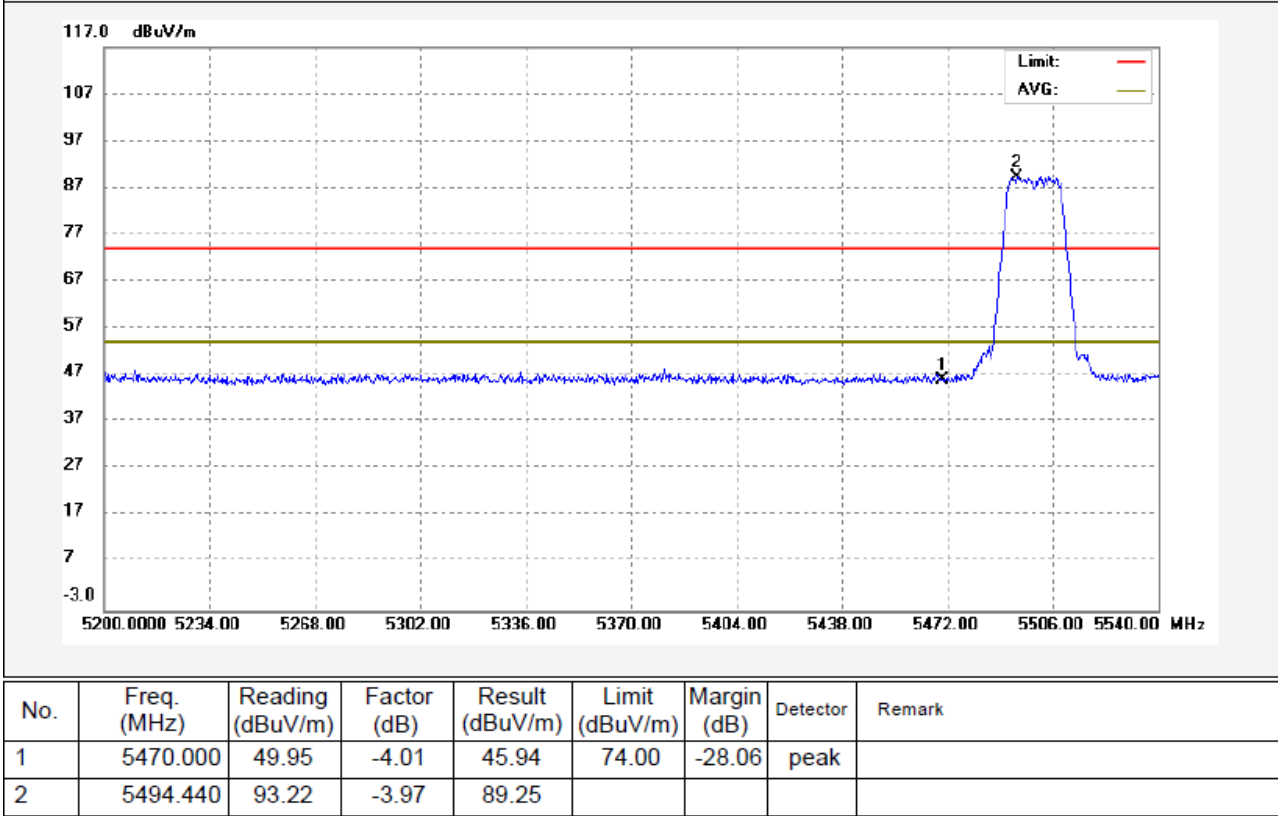
802.11a(HT20) U-NII-2C Transmitting Band edge-left side Horizontal
