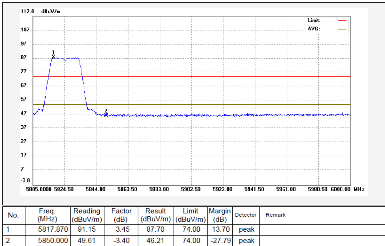
802.11n (HT20) U-NII-3 Transmitting Band edge-right side Horizontal
