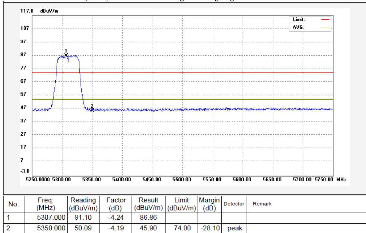
802.11n(HT40) U-NII-2A Transmitting Band edge-right side Horizontal
