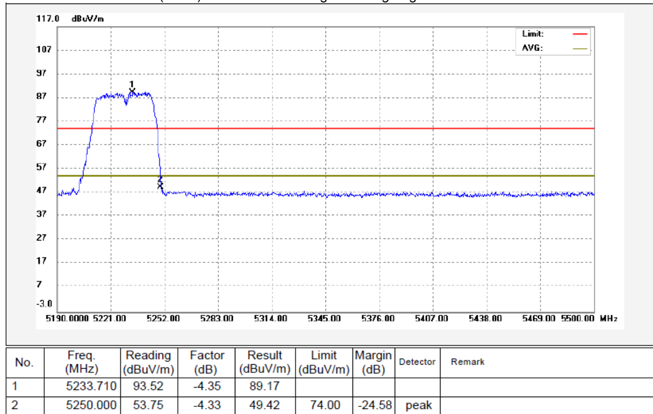
802.11ac(HT40) U-NII-1 Transmitting Band edge-right side Horizontal
