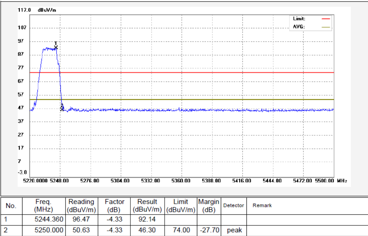
802.11a(HT20) U-NII-1 Transmitting Band edge-right side Horizontal
