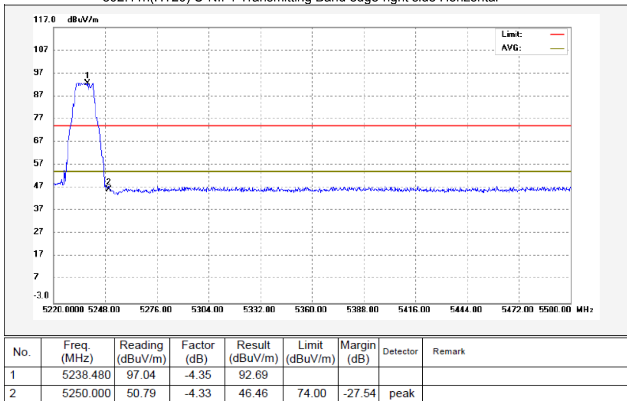
802.11n(HT20) U-NII-1 Transmitting Band edge-right side Horizontal
