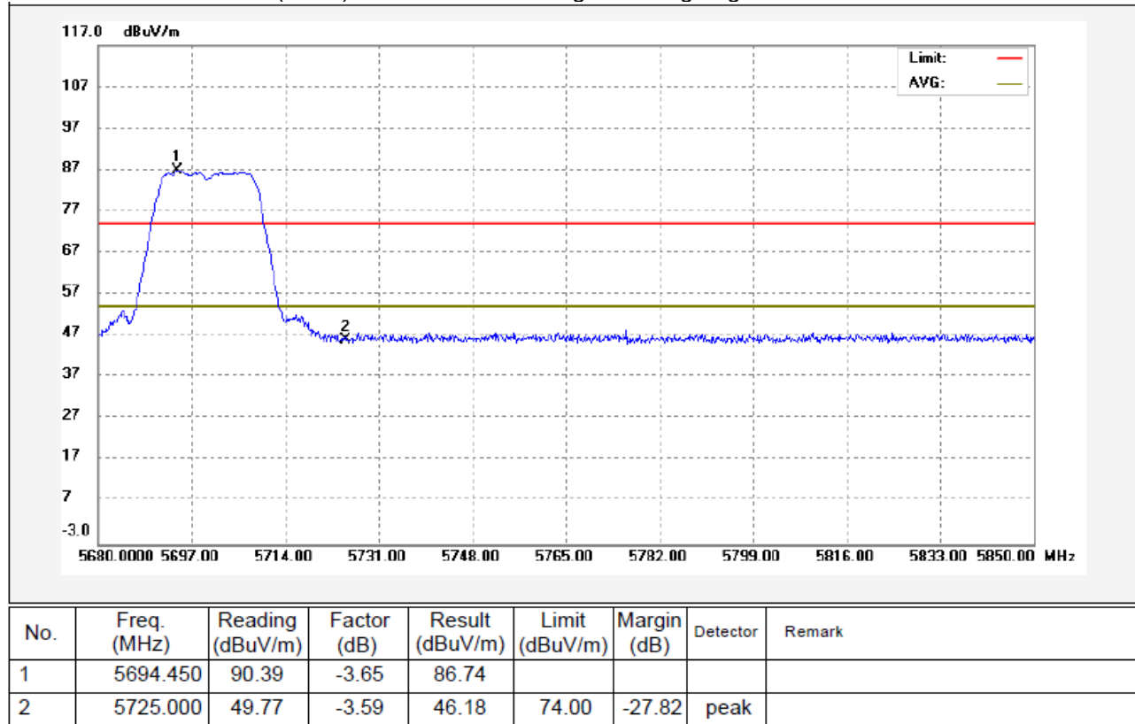
802.11a(HT20) U-NII-2C Transmitting Band edge-right side Vertical
