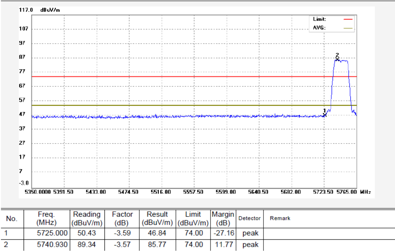
802.11ac(HT20) U-NII-3 Transmitting Band edge-left side Vertical
