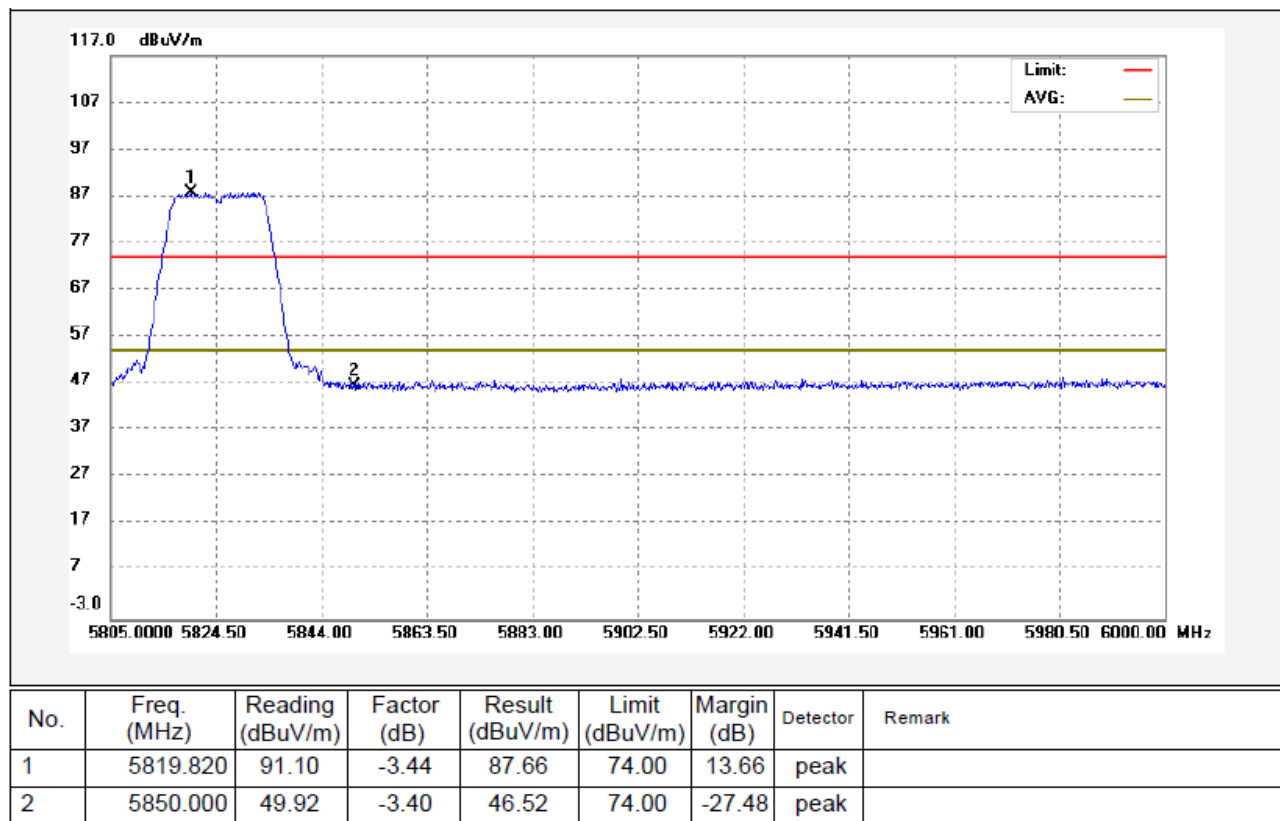
802.11ac(HT20) U-NII-3 Transmitting Band edge-right side Horizontal
