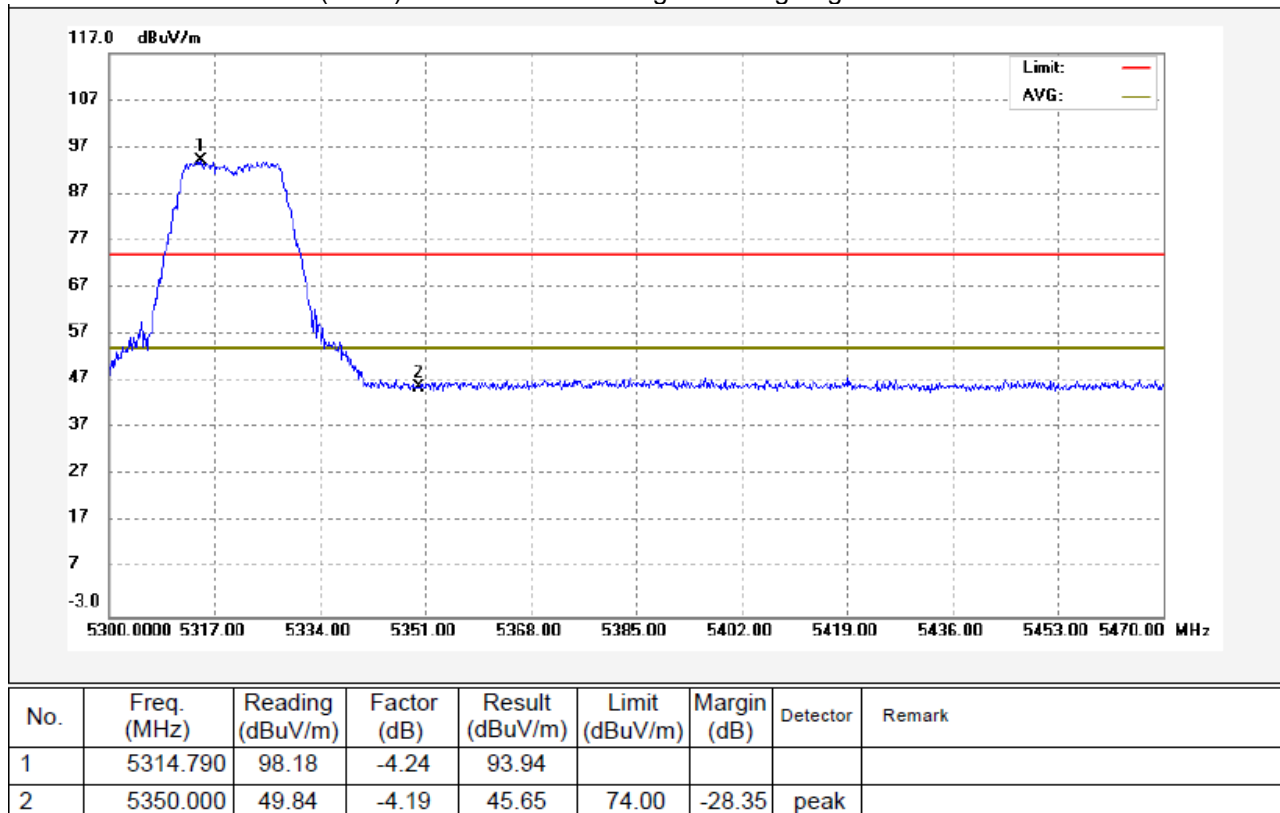
802.11ac(HT20) U-NII-2A Transmitting Band edge-right side Vertical
