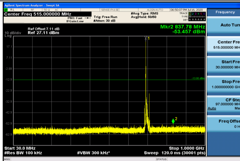
Band12-10MHz-16QAM-23060-1RB#0-30~1000MHz
