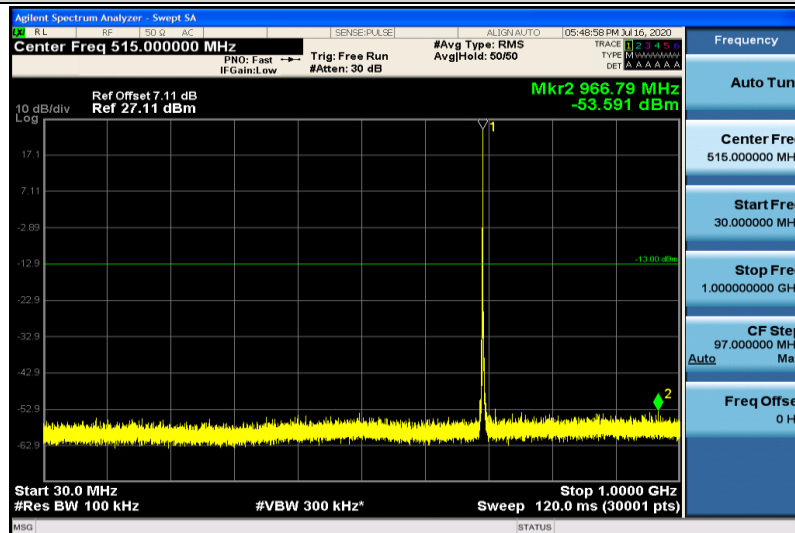
Band12-1.4MHz-16QAM-23017-1RB#0-30~1000MHz
