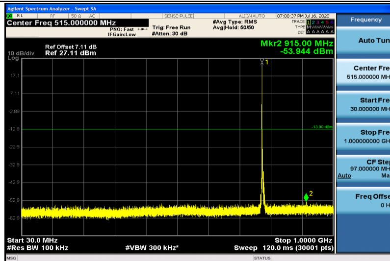
Band13-5MHz-QPSK-23205-1RB#0-30~1000MHz
