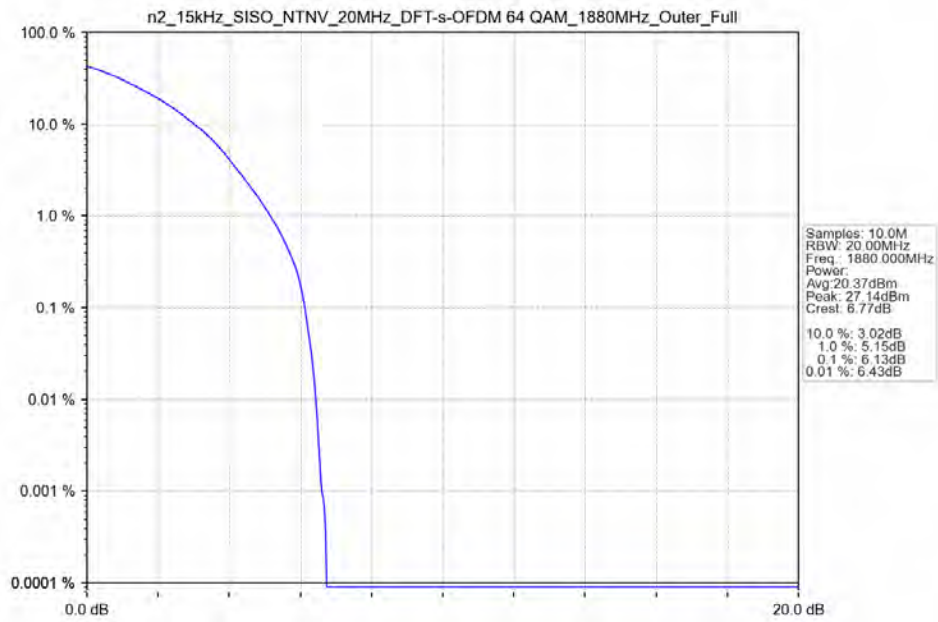
n2_15kHz_SISO_NTNV_20MHz_DFT-s-OFDM_64_QAM_1880MHz_Outer_Full_Ant41
