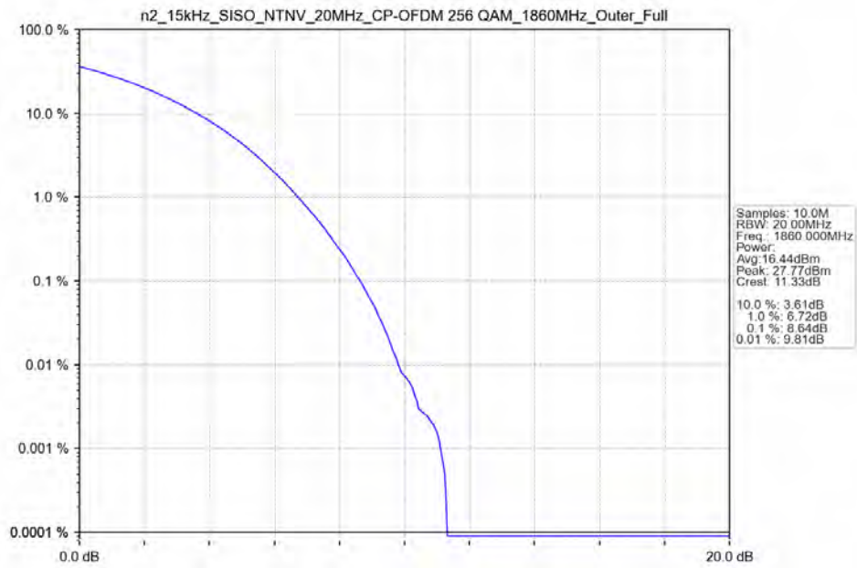
n2_15kHz_SISO_NTNV_20MHz_CP-OFDM_256_QAM_1860MHz_Outer_Full_Ant41
