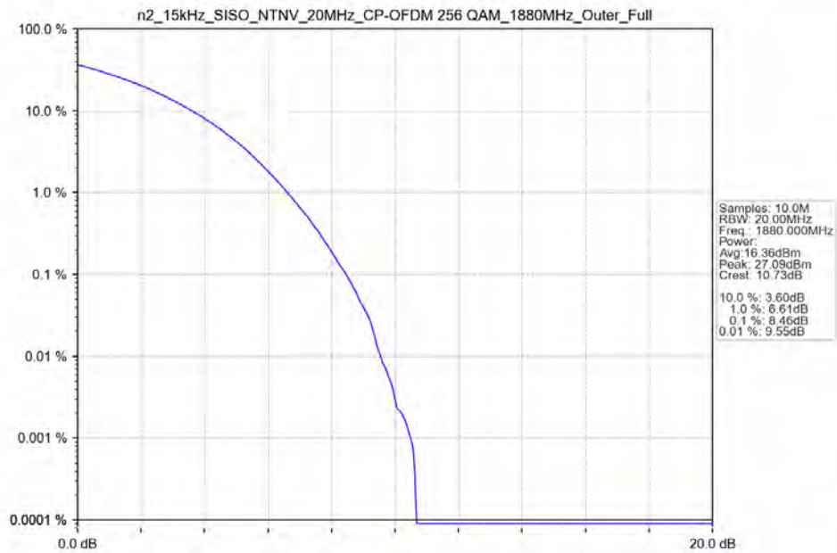
n2_15kHz_SISO_NTNV_20MHz_CP-OFDM_256_QAM_1880MHz_Outer_Full_Ant41
