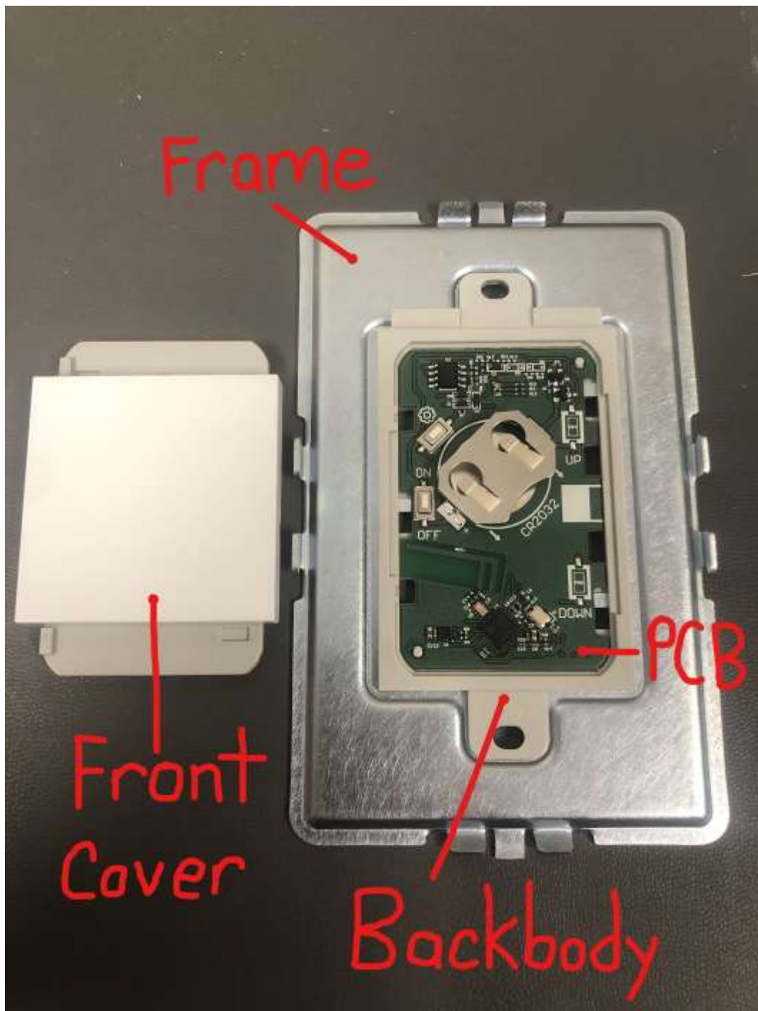
Internal Photo Legrand Model WNAL23 Assembly View
