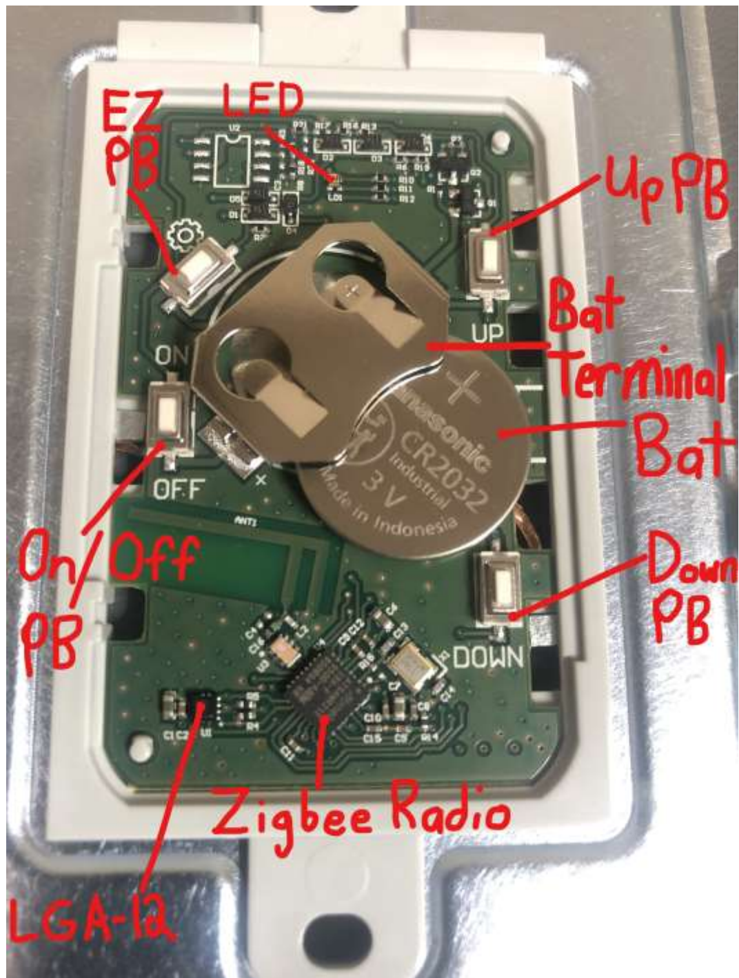
Internal Photo Legrand Model WNAL63 PCB View With Zigbee Radio Location
