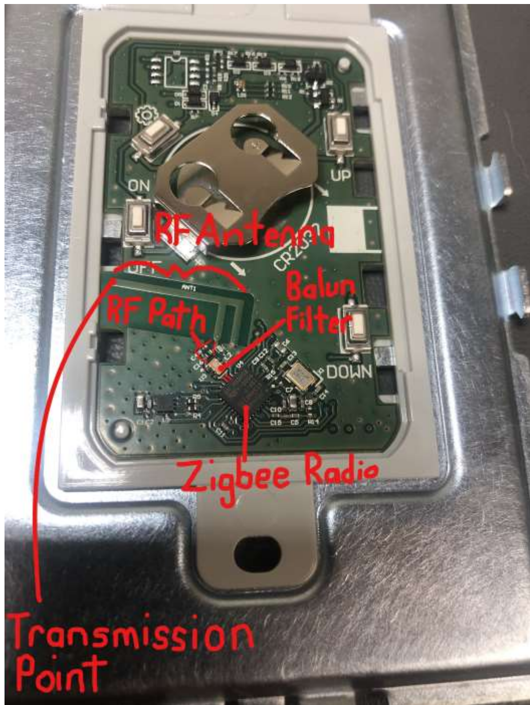
Internal Photo Legrand Model WNAL63 PCB View With Zigbee Radio Antenna Location
