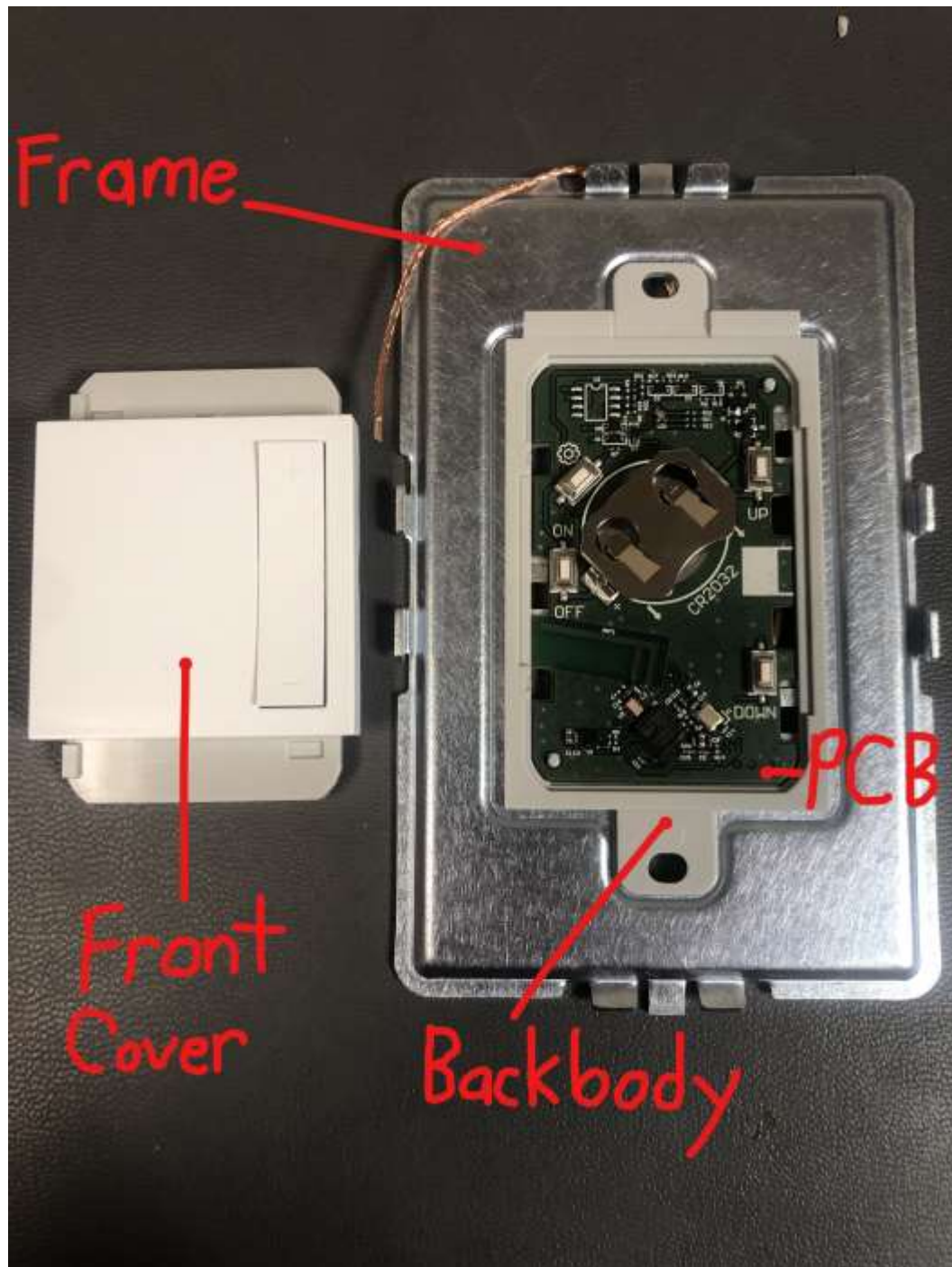
Internal Photo Legrand Model WNAL63 Assembly View
