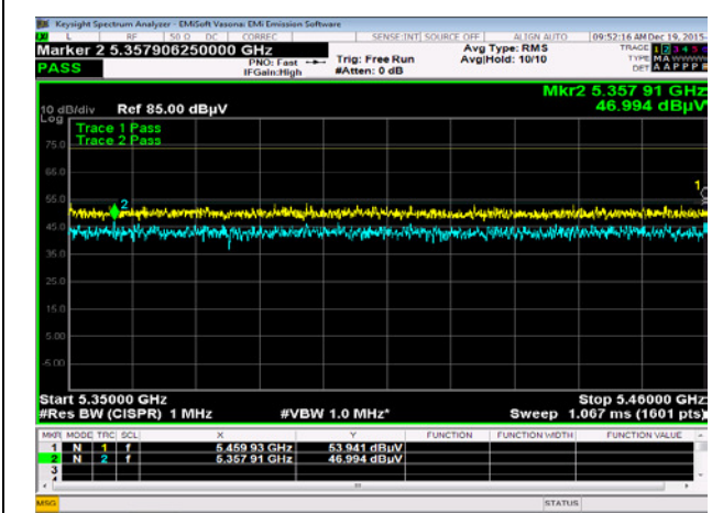
Lower Band 802.11ac-80 55300MHz
