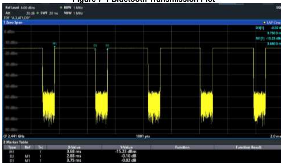
Figure 7-1 Bluetooth Transmission Plot
