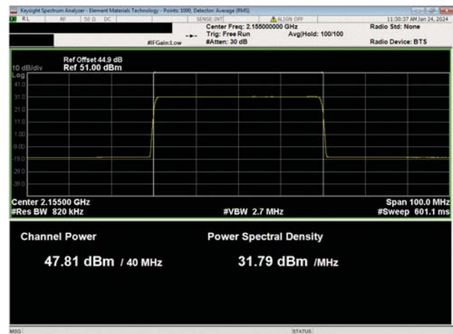
PCS Multicarrier Multiband Test Case 2 QPSK Modulation AWS Band n66, NR40, Mid Ch, 2155.0 MHz
