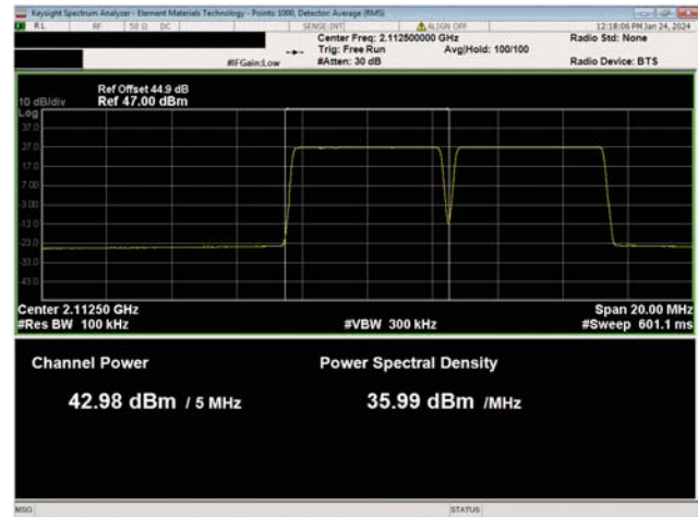
AWS Multicarrier Multiband Test Case 1 QPSK Modulation AWS Band n66, NR5, Low Ch, 2112.5 MHz
