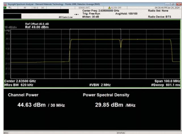
BRS Multicarrier Multiband Test Case 2 QPSK Modulation BRS Band n7, NR30, Low Ch, 2635.0 MHz
