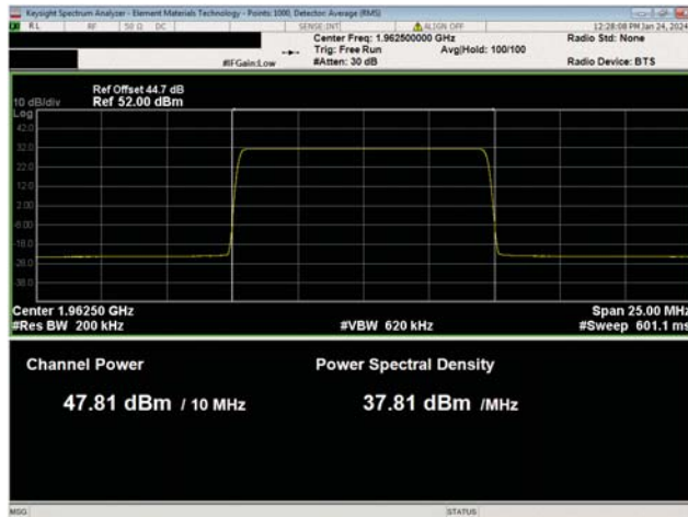
AWS Multicarrier Multiband Test Case 1 QPSK Modulation PSC Band n25, NR10, Mid Ch, 1962.5 MHz
