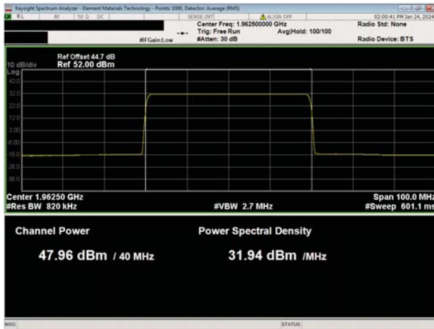
AWS Multicarrier Multiband Test Case 3 QPSK Modulation PSC Band n25, NR40, Mid Ch, 1962.5 MHz
