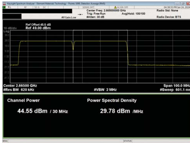
BRS Multicarrier Multiband Test Case 2 QPSK Modulation BRS Band n7, NR30, Low Ch, 2665.0 MHz
