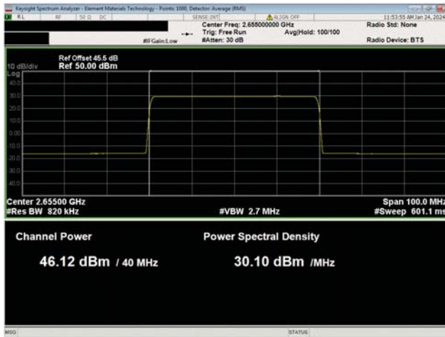
PCS Multicarrier Multiband Test Case 3 QPSK Modulation BRS Band n7, NR40, Mid Ch, 2655.0 MHz
