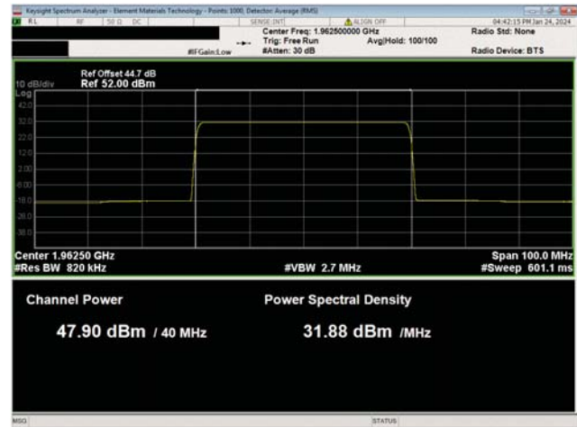
BRS Multicarrier Multiband Test Case 2 QPSK Modulation PSC Band n25, NR40, Mid Ch, 1962.5 MHz
