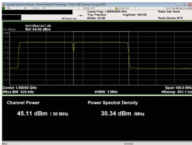
PCS Multicarrier Multiband Test Case 3 QPSK Modulation PSC Band n25, NR30, High Ch, 1980.0 MHz
