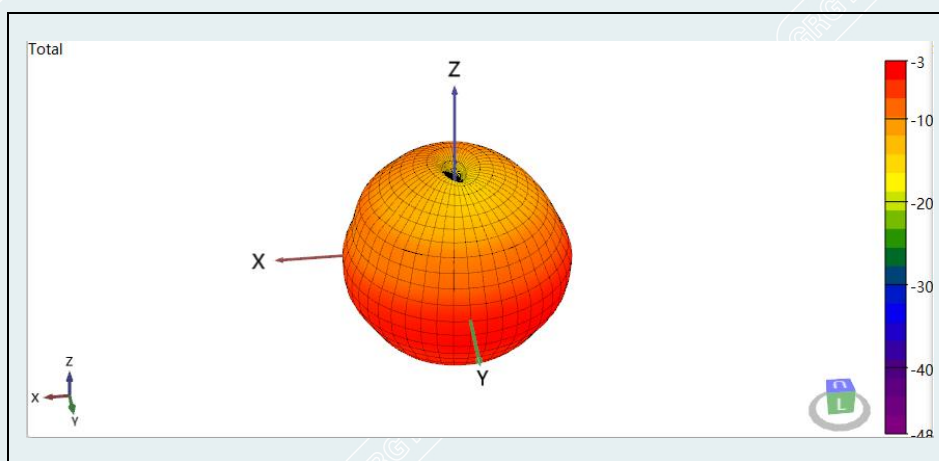
2500MHz (Gain: dBi)
