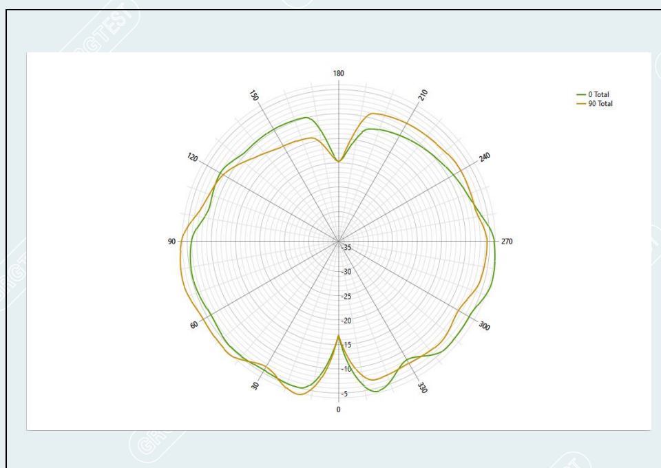
Phi=0 ° &amp;Phi=90 °_2500 MHz (Gain: dBi)
