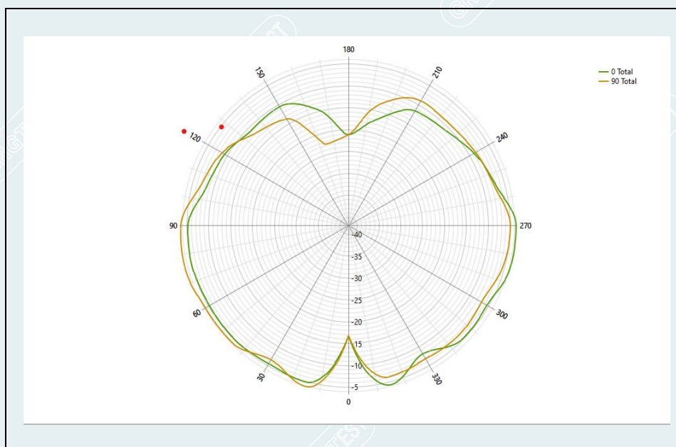
Phi=0 ° &amp;Phi=90 °_2460 MHz (Gain: dBi)
