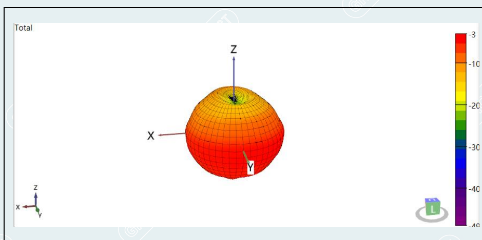
2460MHz (Gain: dBi)
