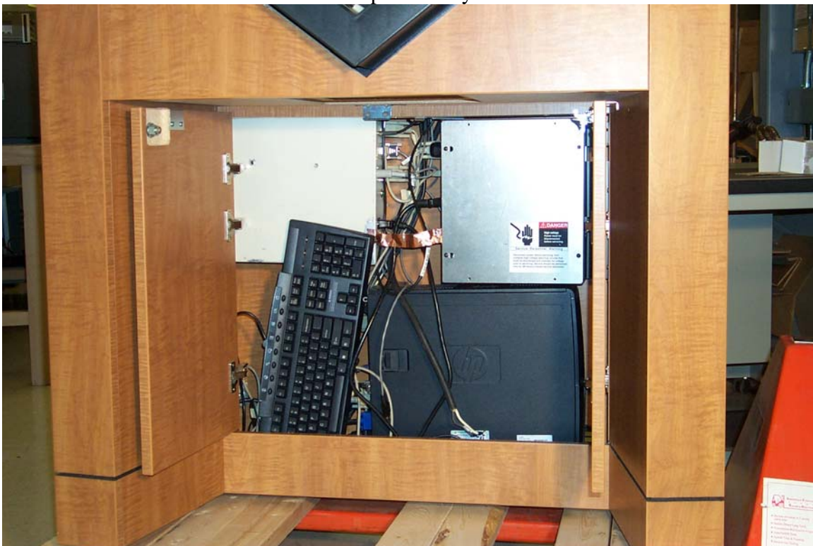
Kiosk Internal Component Layout – Front View
