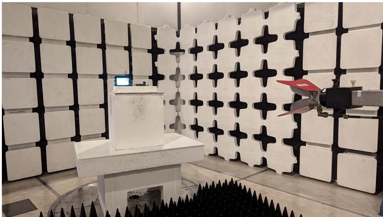
LTE Spurious
