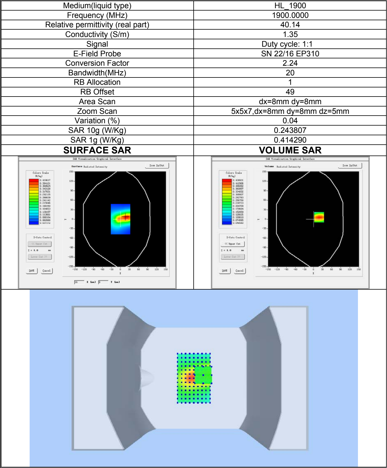
Plot 12:LTE BAND 2, High channel (Body-worn /Hotspot, Right Edge) Product Description:Smart Phone Test Date: 2023-05-16
