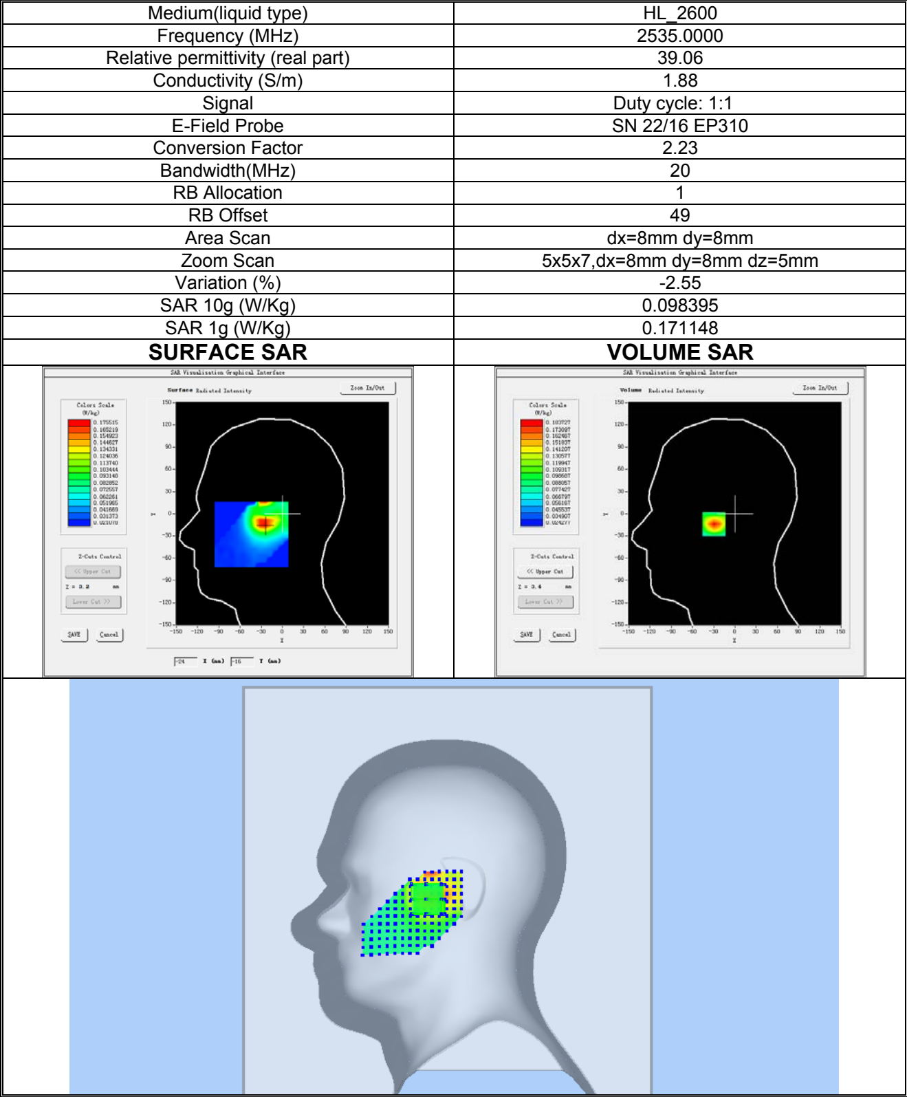
Plot 17:LTE BAND 7, Middle channel (Right Head Cheek) Product Description: Smart Phone Test Date: 2023-05-24
