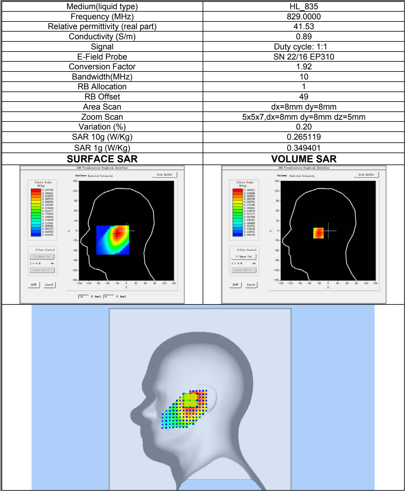
Plot 15:LTE BAND 5, Low channel (Right Head Cheek) Product Description: Smart Phone Test Date: 2023-05-22
