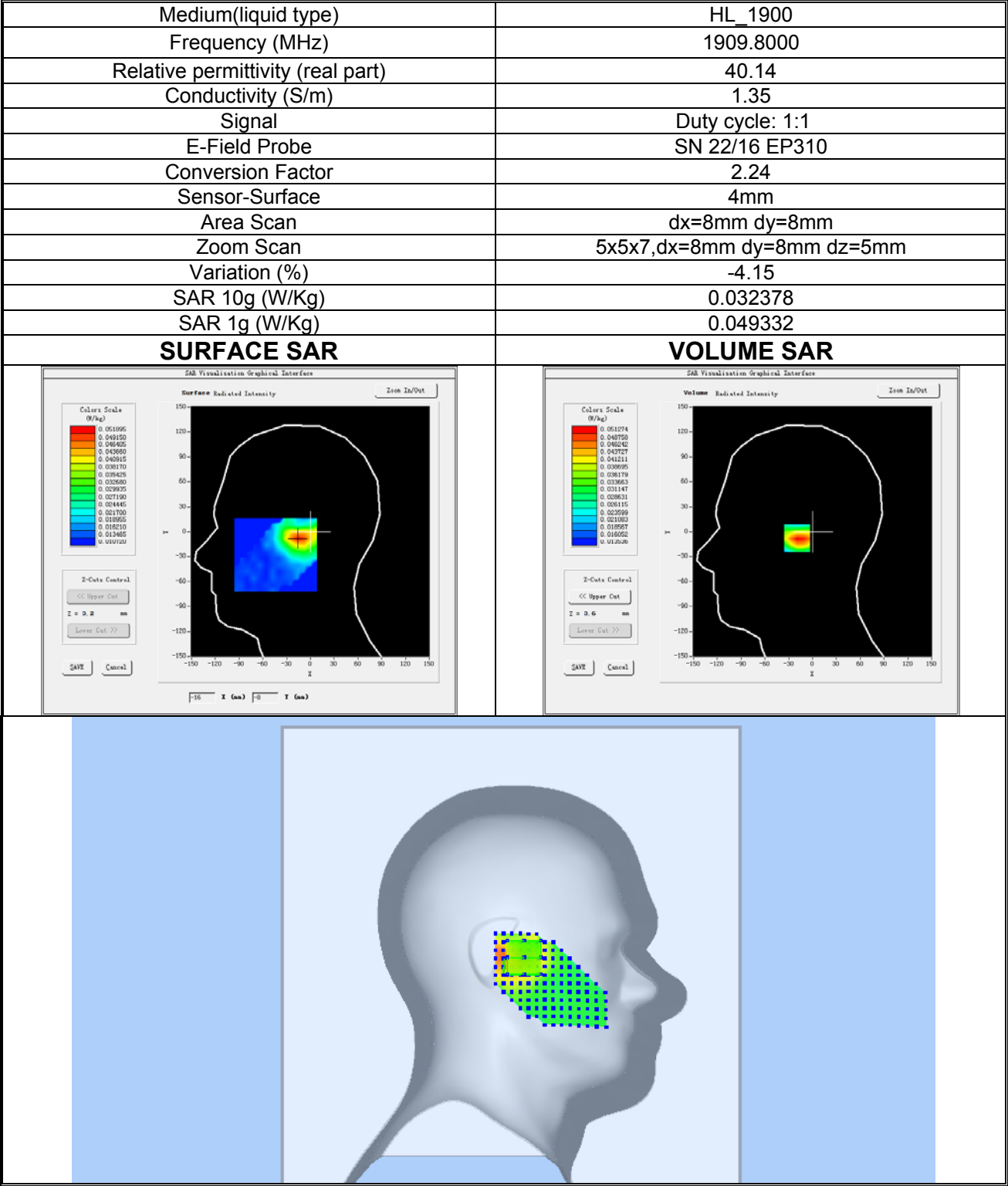
Plot 3: GPRS1900, High channel (Left Head Cheek) Product Description: Smart Phone Test Date: 2023-05-15
