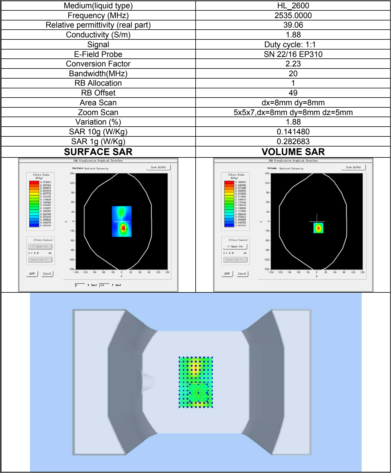
Plot 18: LTE BAND 7, Middle channel (Body-worn/ Hotspot, Bottom Edge) Product Description: Smart Phone Test Date: 2023-05-24
