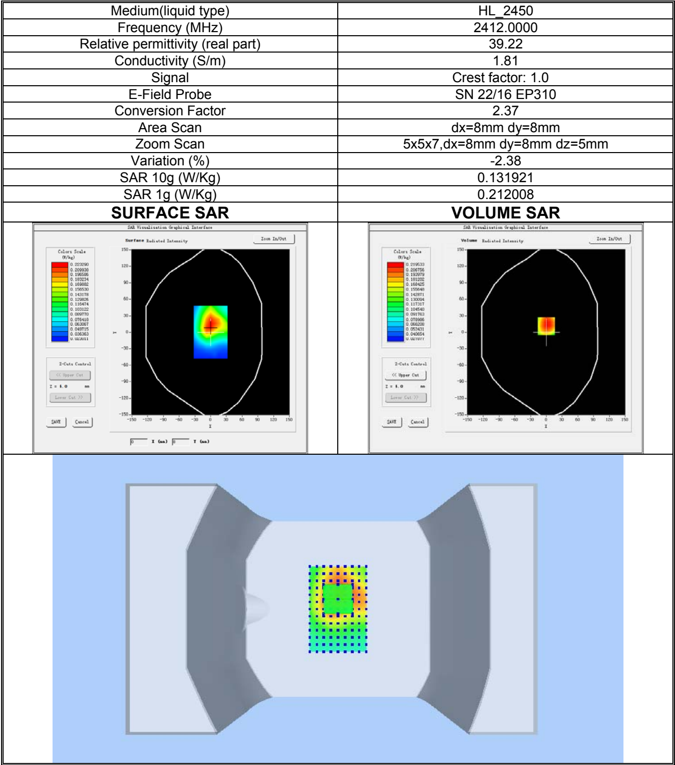
Plot 26: 2.4G Wi-Fi, Low channel (Body-worn/ Hotspot, Front Side) Product Description: Smart Phone Test Date: 2023-05-23
