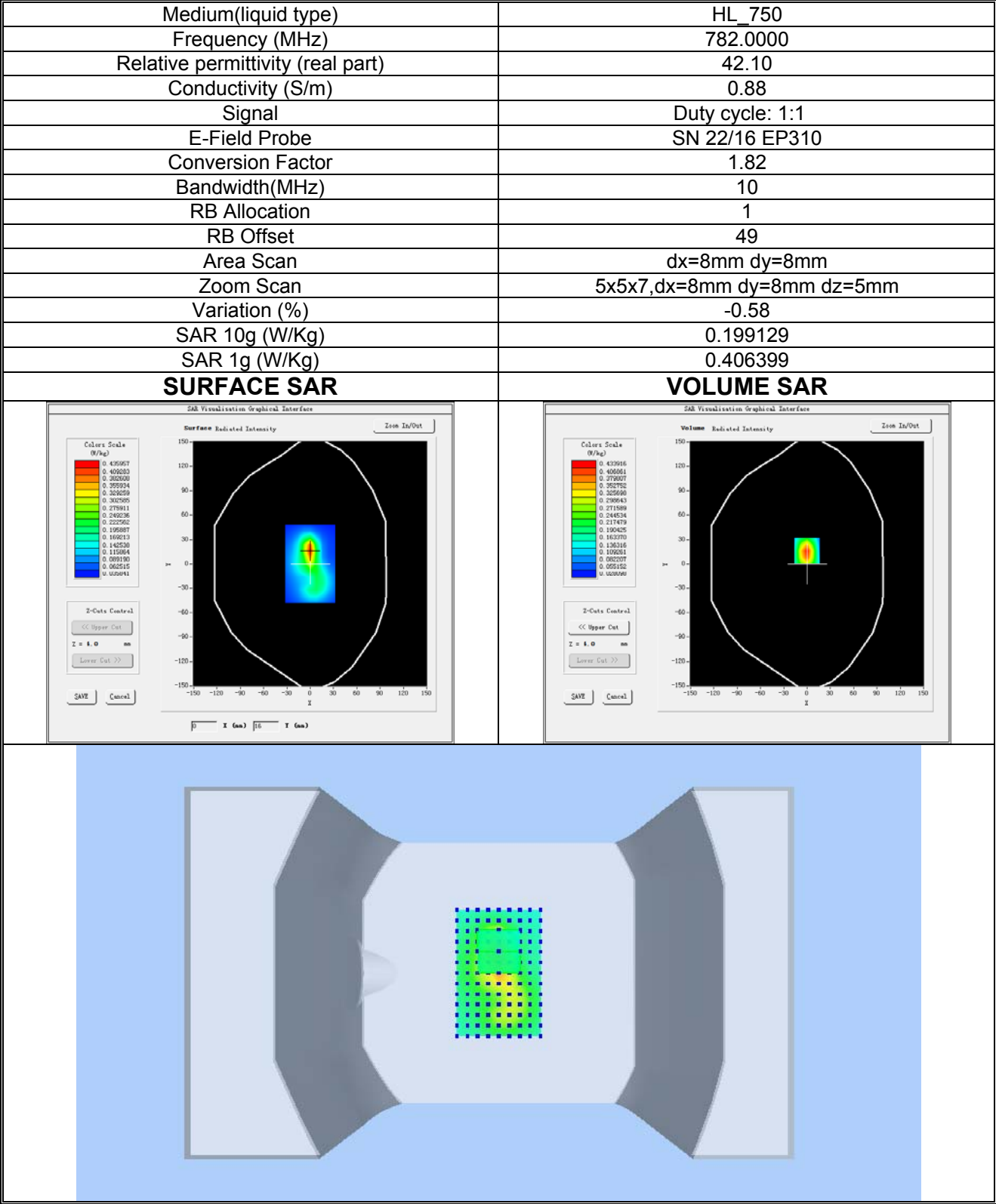
Plot 22: LTE BAND 13, Middle channel (Body-worn/ Hotspot, Bottom Edge) Product Description: Smart Phone Test Date: 2023-05-19
