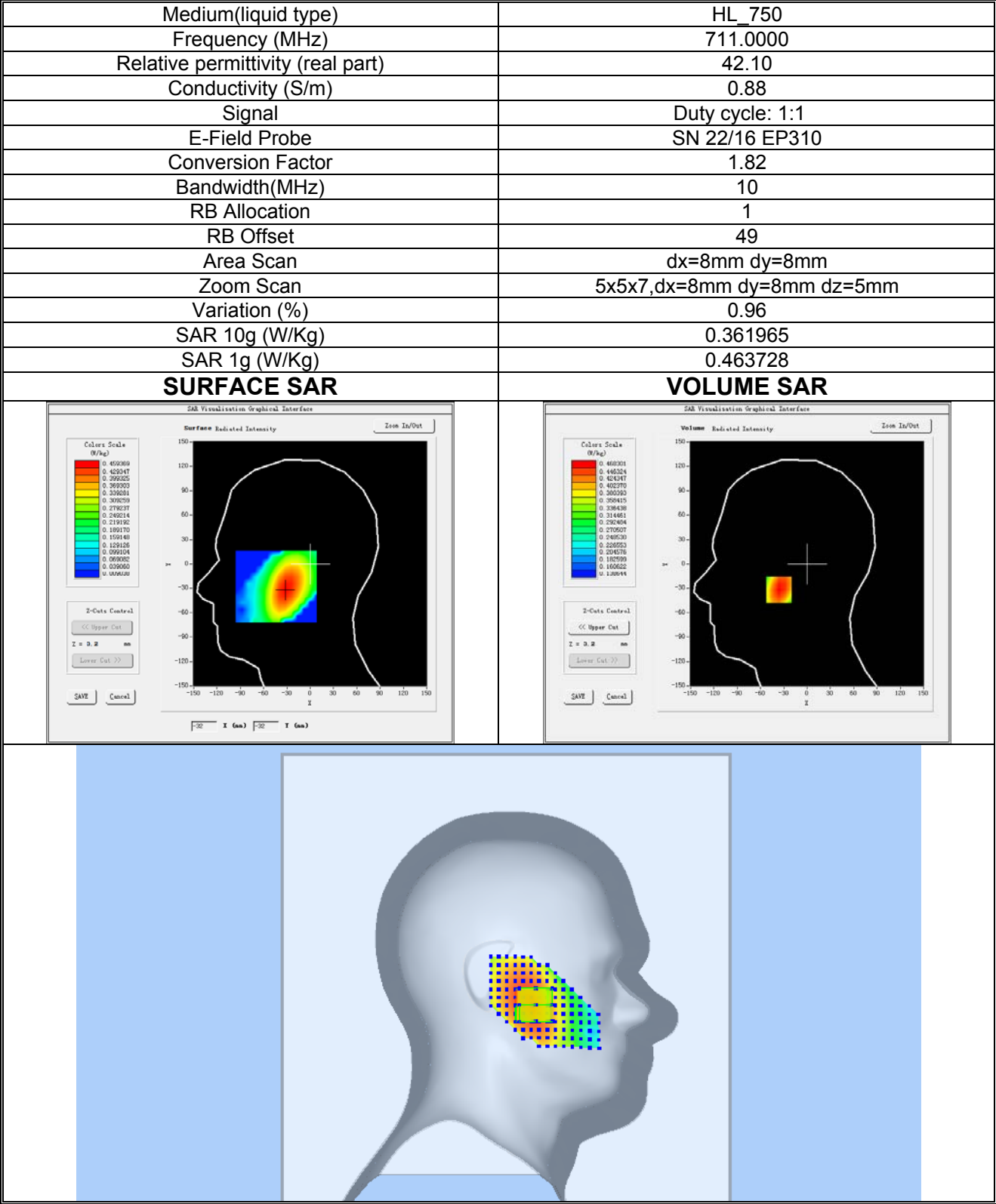
Plot 19:LTE BAND 12, High channel (Left Head Cheek) Product Description: Smart Phone Test Date: 2023-05-19
