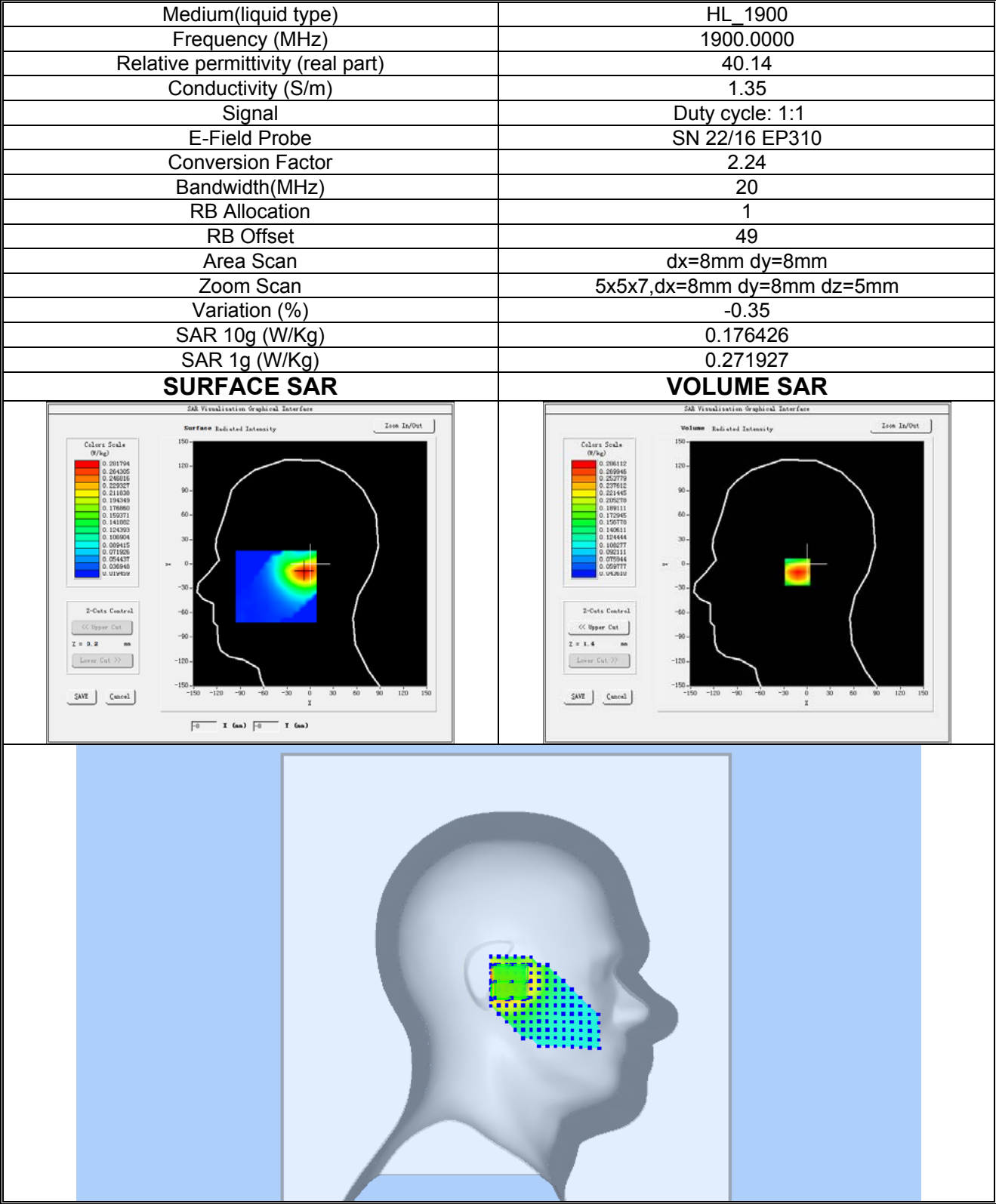
Plot 11:LTE BAND 2, High channel (Left Head Cheek) Product Description:Smart Phone Test Date: 2023-05-16
