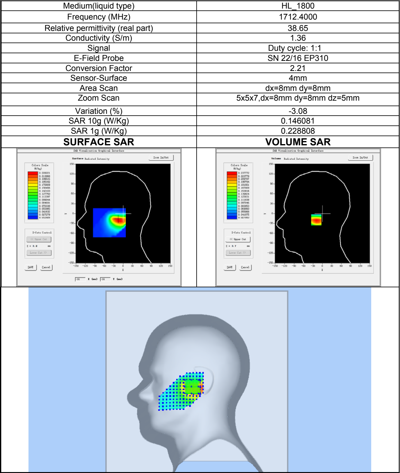
Plot 7: WCDMA BAND IV, Low channel (Right Head Cheek) Product Description: Smart Phone Test Date: 2023-05-15
