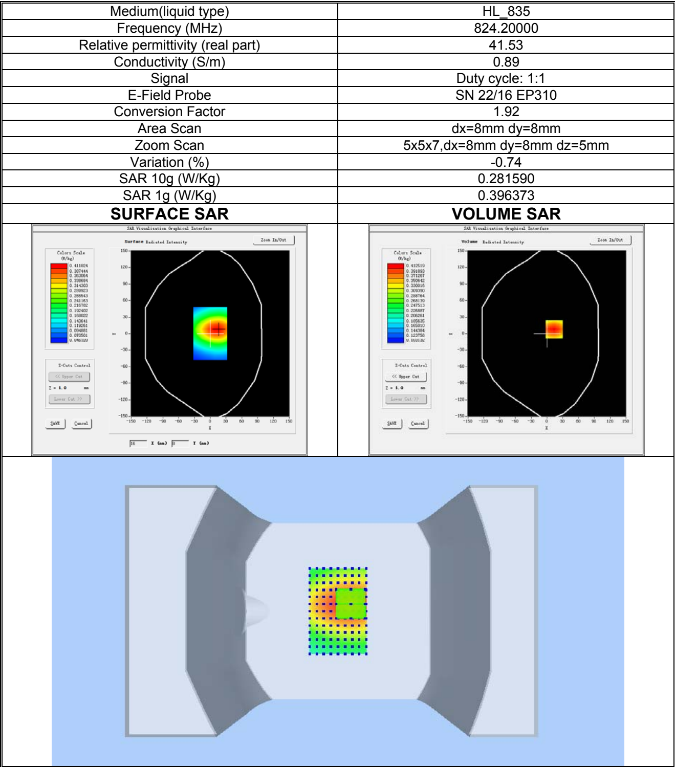
Plot 2: GPRS850MHz, Low channel (Body-worn /Hotspot, Right Edge) Product Description:Smart Phone Test Date: 2023-05-22
