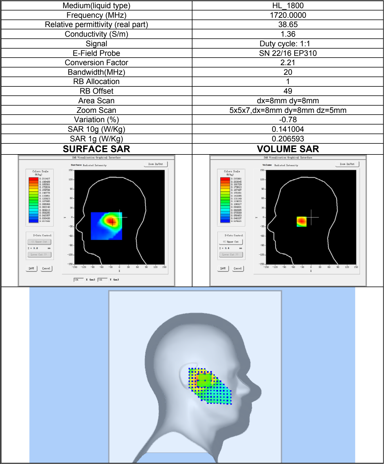
Plot 13:LTE BAND 4, Low channel (Left Head Cheek) Product Description: Smart Phone Test Date: 2023-05-16
