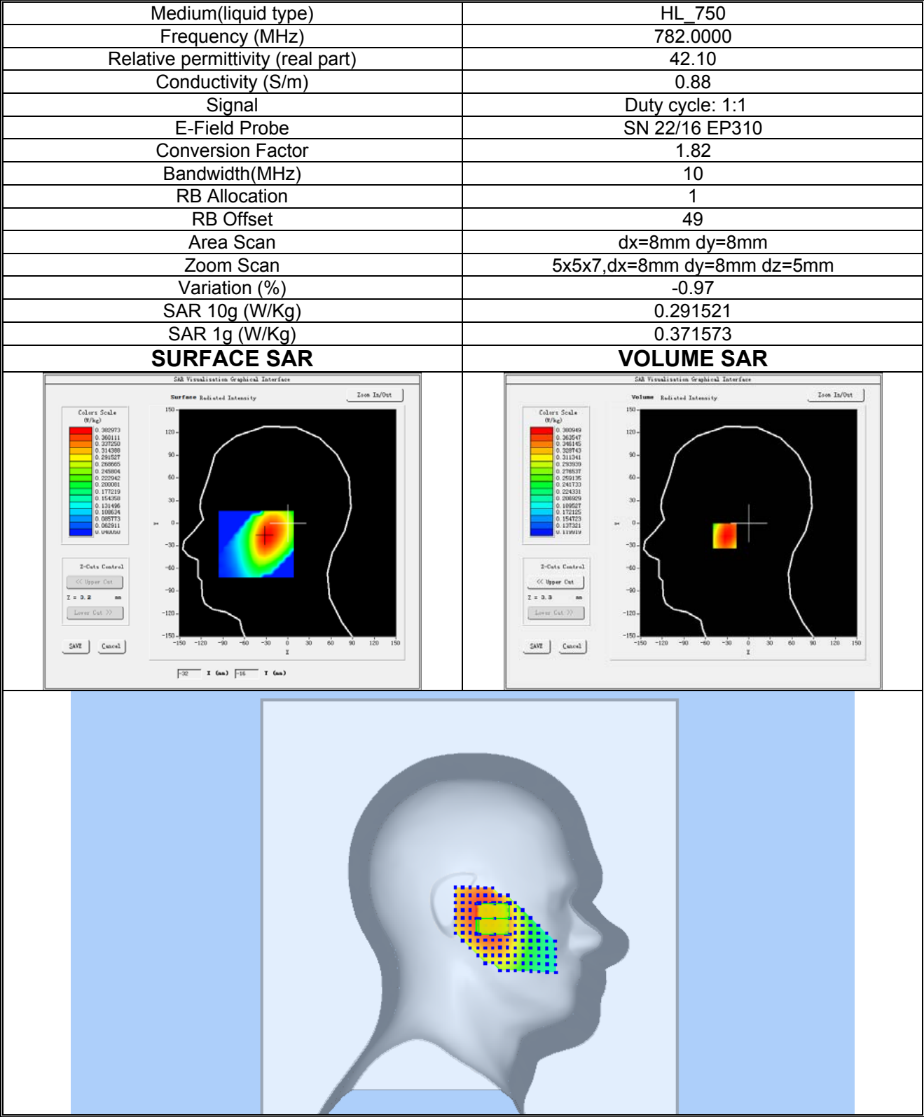
Plot 21:LTE BAND 13, Middle channel (Left Head Cheek) Product Description: Smart Phone Test Date: 2023-05-19
