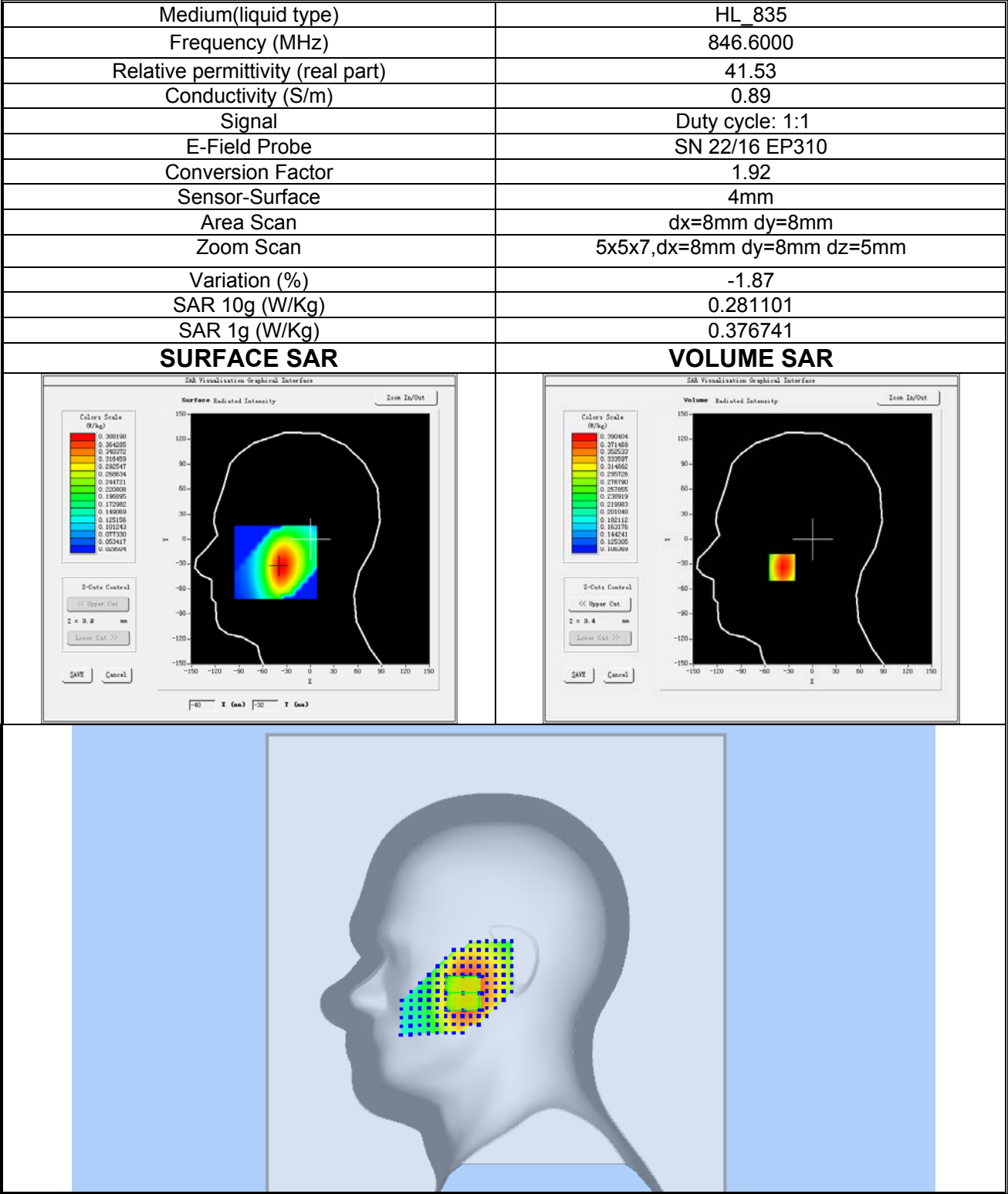
Plot 9: WCDMA BAND V, High channel (Right Head Cheek) Product Description: Smart Phone Test Date: 2023-05-22
