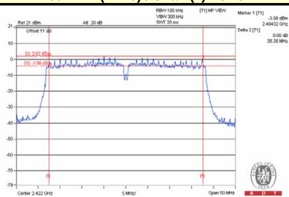
802.11n (HT40) / Chain(1) : CH3
