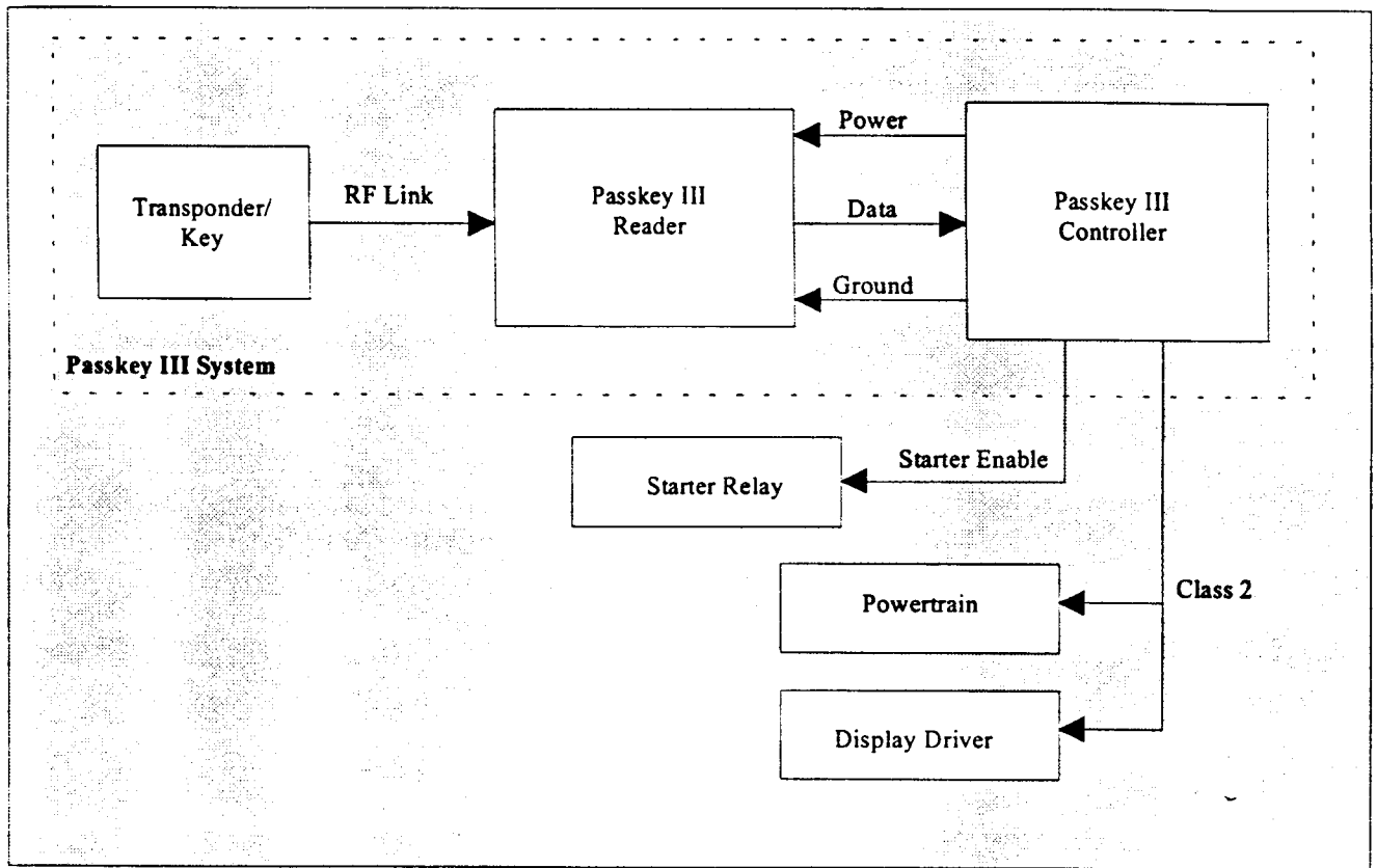
Figure 2.0. Passkey III (In-Dash) System Block Diagram
