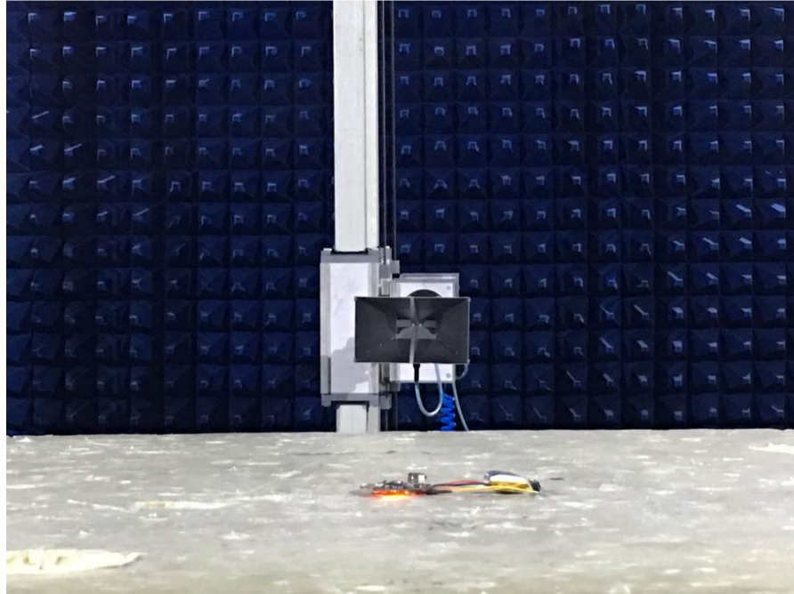
Photograph 4: Set-up for Spurious Emissions (18GHz-26GHz)
