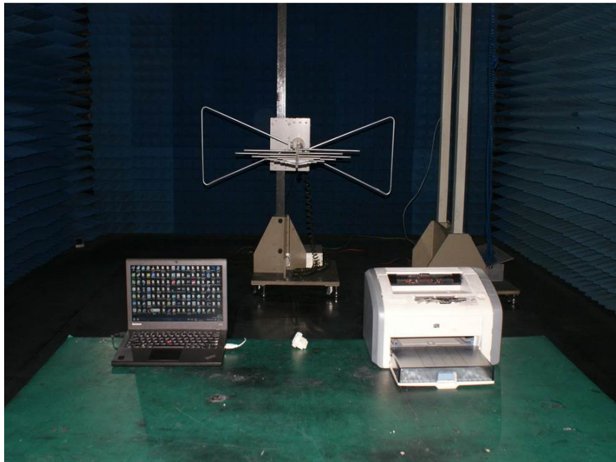
Photograph 6: Set-up for Radiated Emissions, below 1GHz
