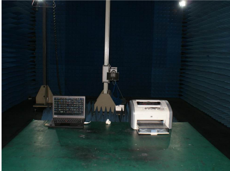
Photograph 7: Set-up for Radiated Emissions, above 1GHz
