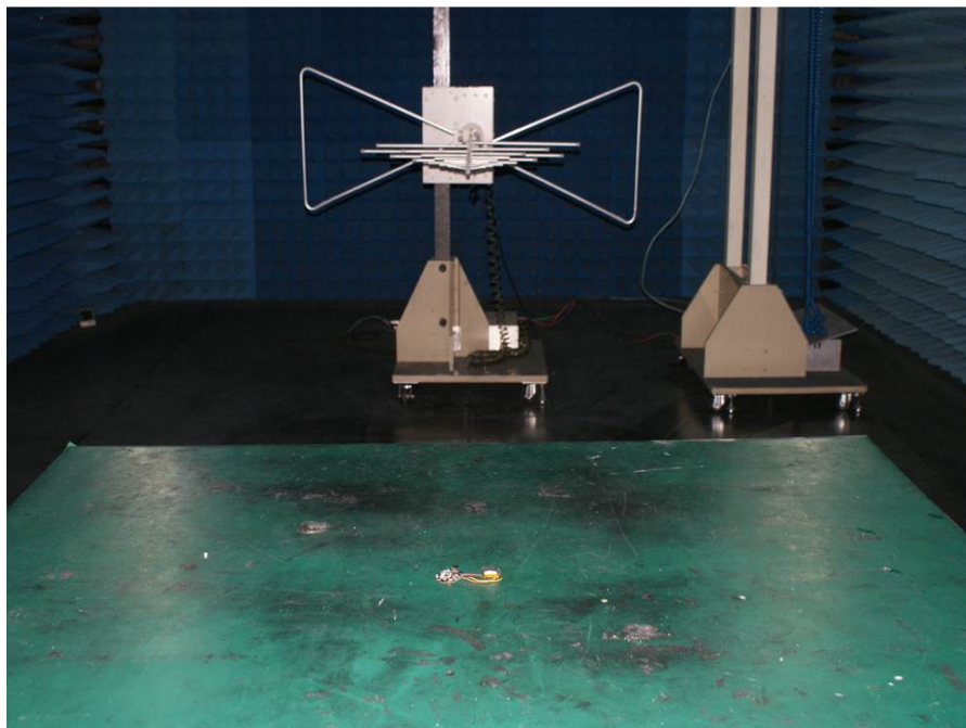
Photograph 2: Set-up for Spurious Emissions (30MHz-1GHz)
