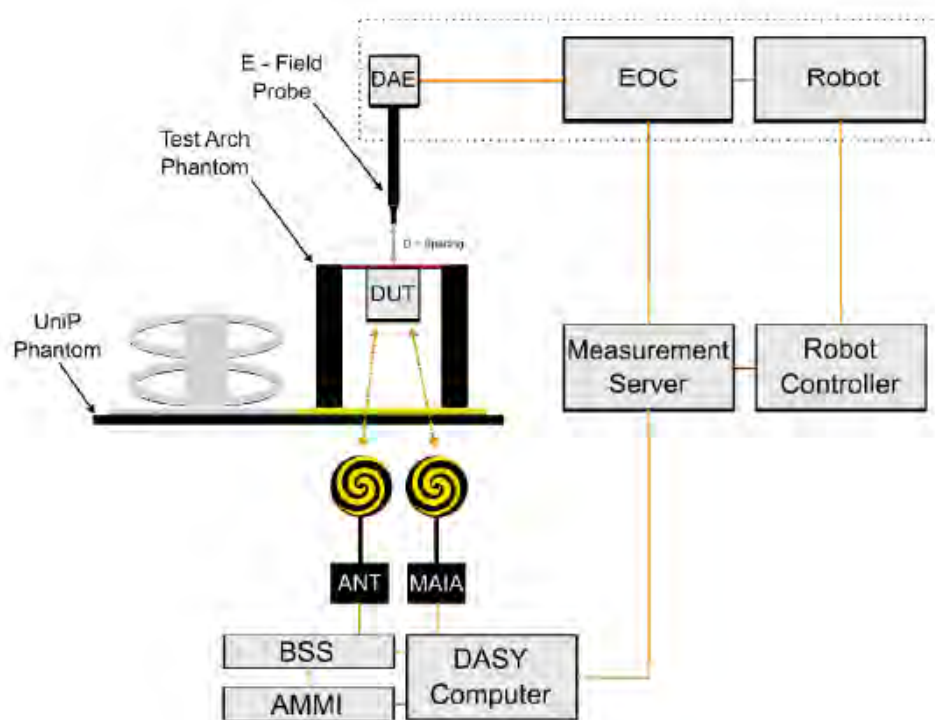
Fig. 1 HAC Test Measurement Set-up
