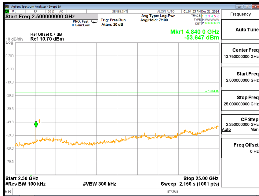
Channel 25 2475MHz
