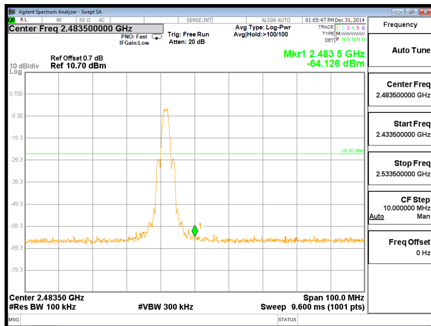
Channel 25 2475MHz
