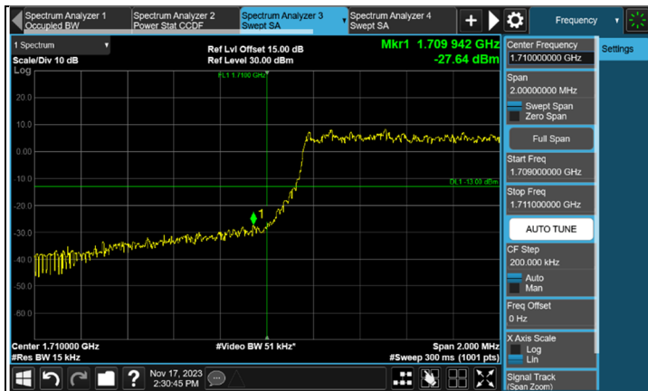
FULL CH 19957 (1710.7 MHz)
