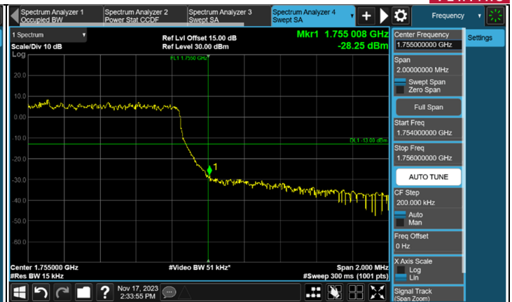
FULL CH 20393 (1754.3 MHz)
