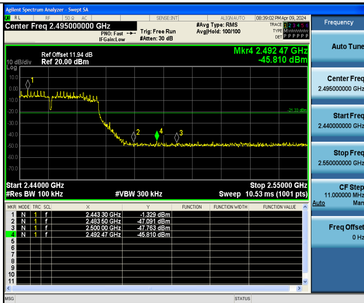
11N40SISO-Ant2-2452-PASS
