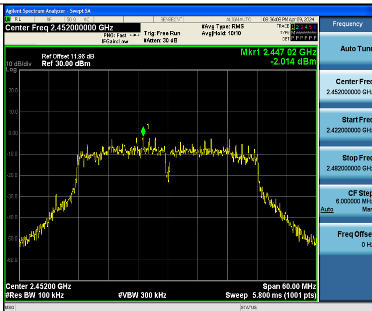
11N40SISO-Ant1-2452-0~Reference-PASS
