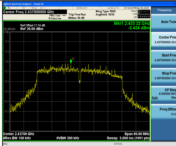
11N40SISO-Ant2-2437-0~Reference-PASS
