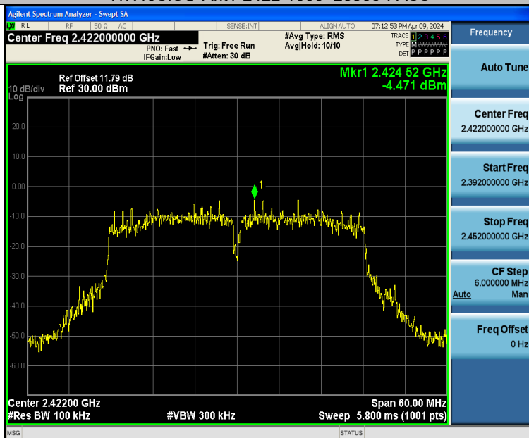
11N40SISO-Ant2-2422-0~Reference-PASS
