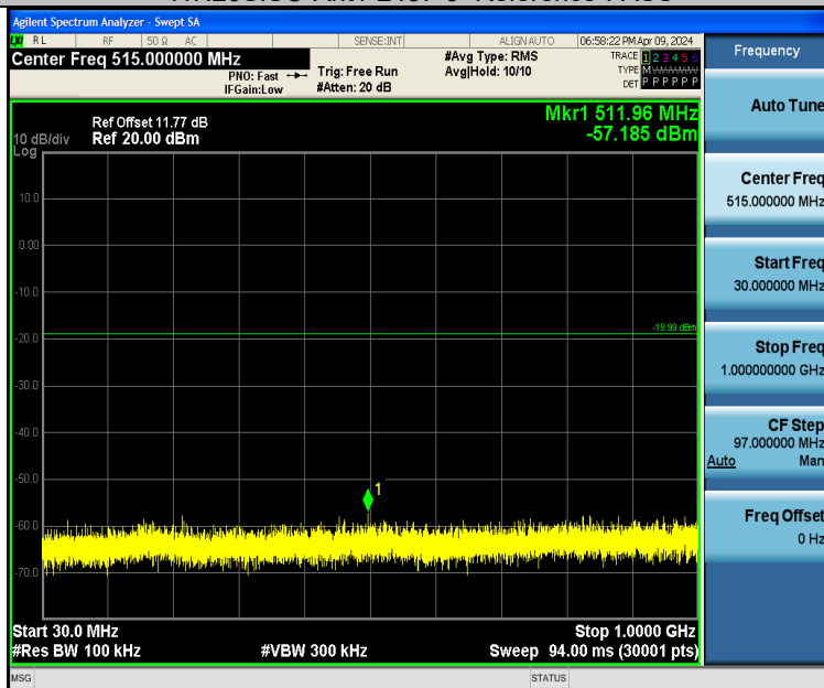
11N20SISO-Ant1-2437-30~1000-PASS
