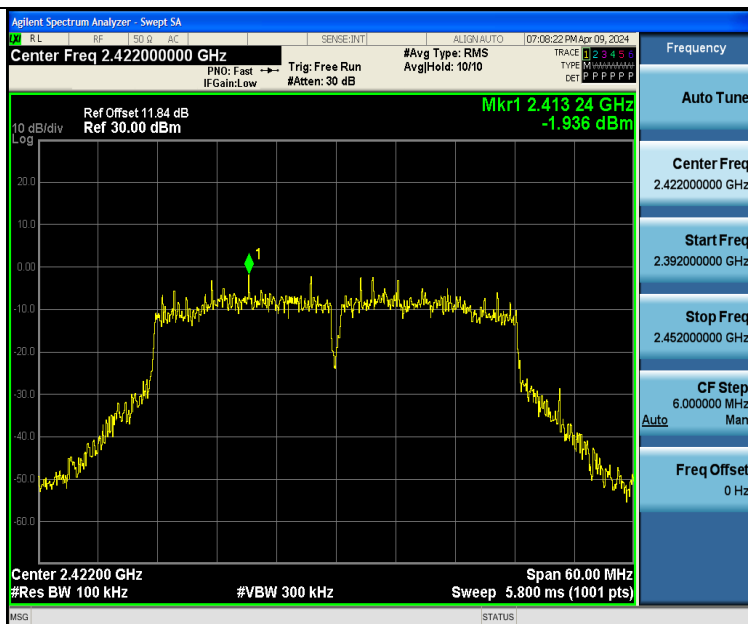
11N40SISO-Ant1-2422-0~Reference-PASS
