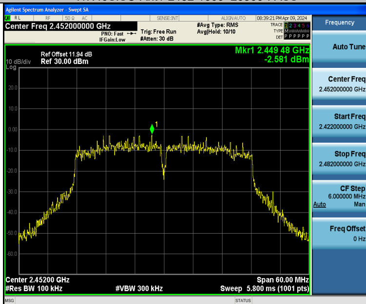
11N40SISO-Ant2-2452-0~Reference-PASS
