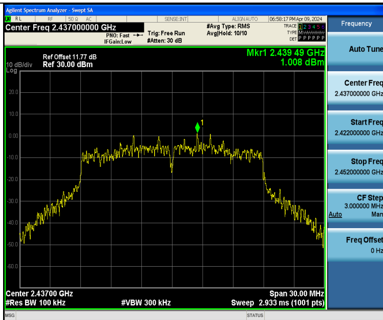
11N20SISO-Ant1-2437-0~Reference-PASS
