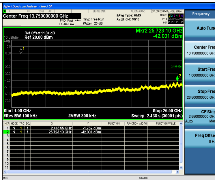
11N40SISO-Ant1-2422-1000~26500-PASS
