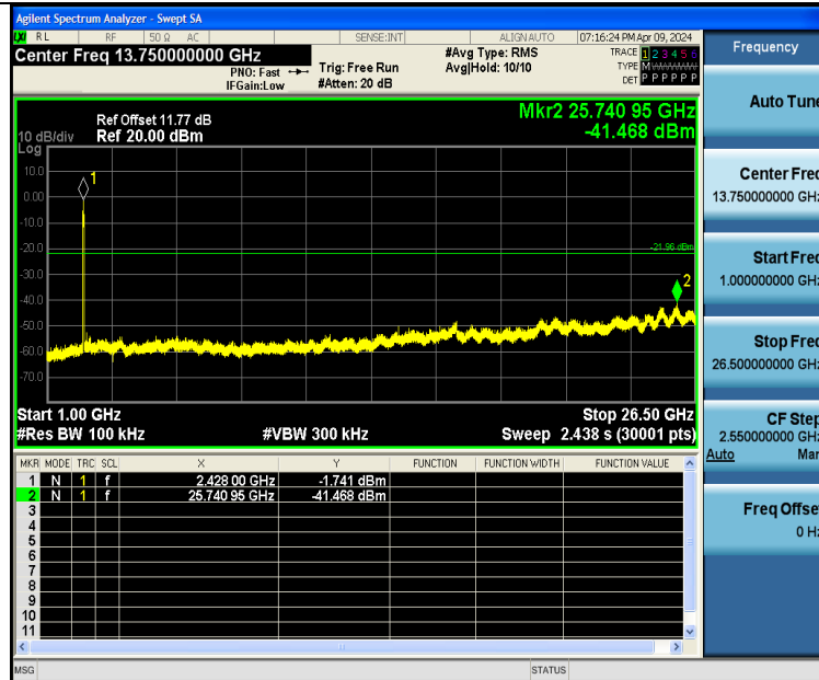
11N40SISO-Ant1-2437-1000~26500-PASS
