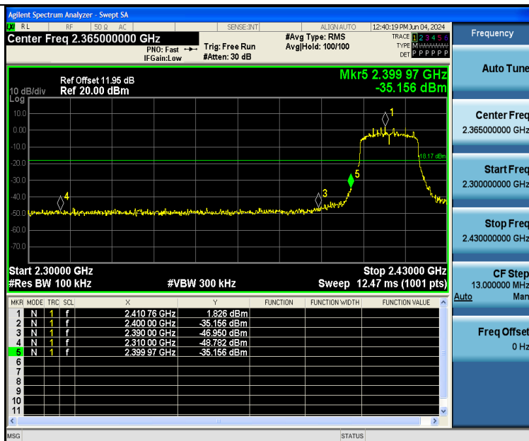
11AX20SISO-Ant1-2412-PASS
