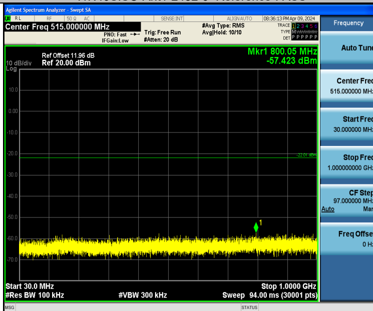
11N40SISO-Ant1-2452-30~1000-PASS
