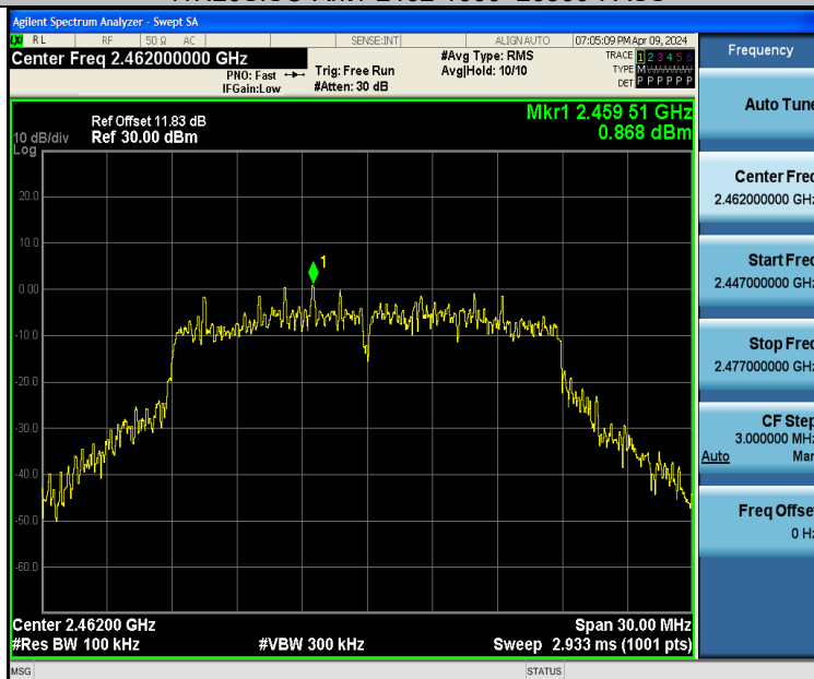
11N20SISO-Ant2-2462-0~Reference-PASS
