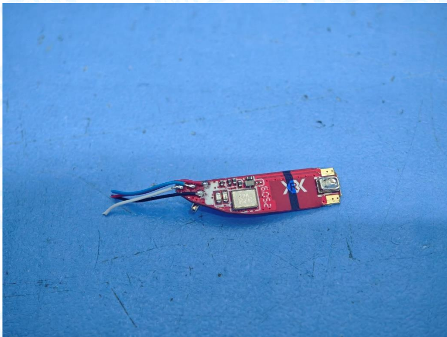
Photo 23 Appearance of PCB-Right
