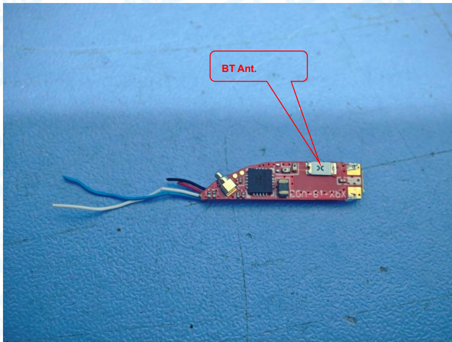
Photo 21 Appearance of PCB-Left
