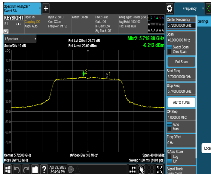
11N20SISO_Ant1_5720_UNII-3
