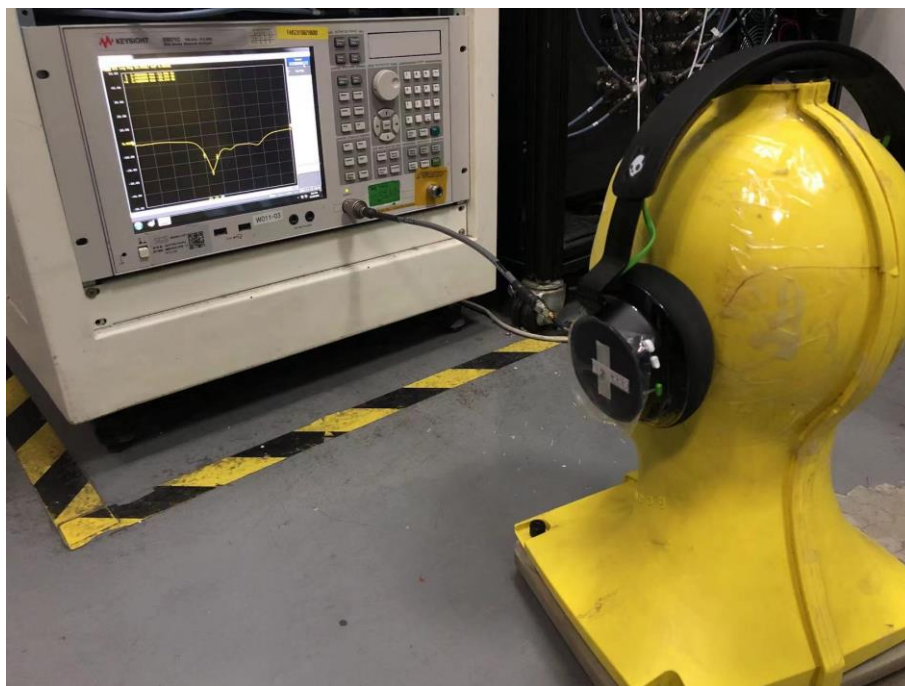
BH-#2 Impedance Setup
