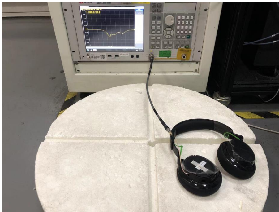
FS-#2 Impedance Setup
